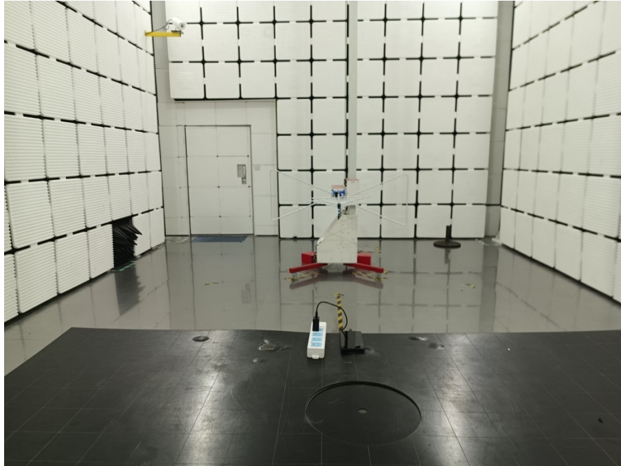
Transmitter unwanted emissions in the spurious domain (9kHz to 30MHz)
