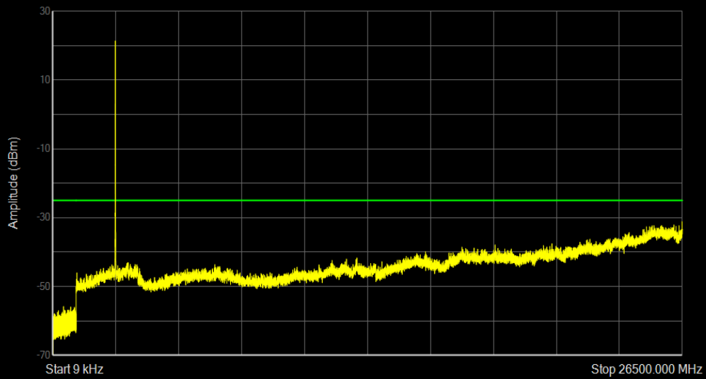
Band41 QPSK BW=5MHz Channel=41215 RB Size=25 Position=#0
