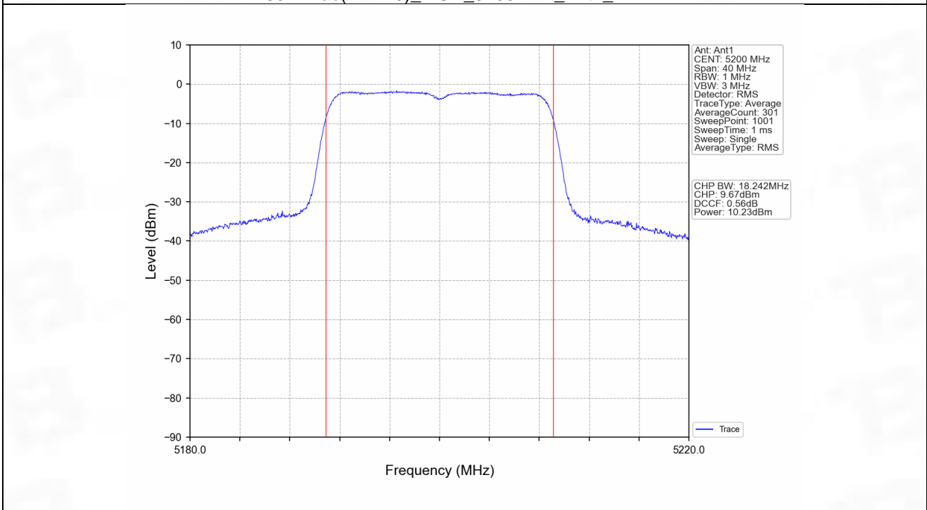
802.11ac(VHT20)_MCH_5200MHz_Ant1_NTNV
