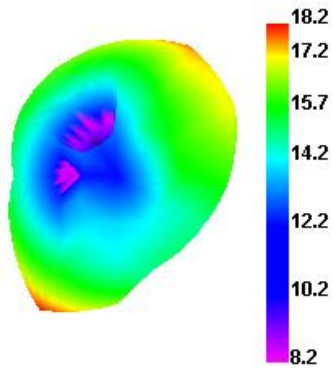
Wifi 1 TRP
