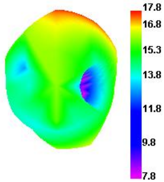
Wifi 165 TRP
