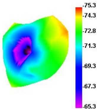
Wifi 13 TIS
