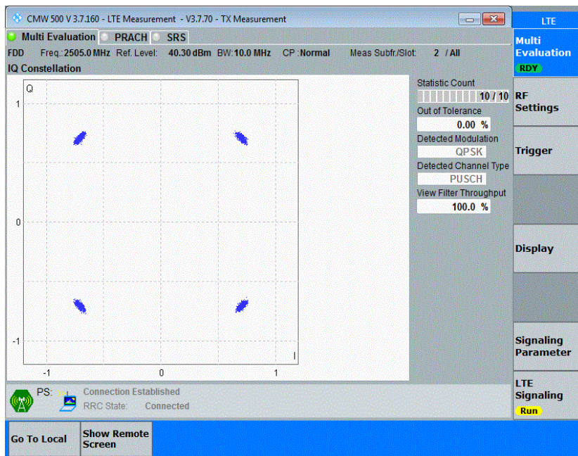
Band7-10MHz-QPSK-21100-50RB#0
