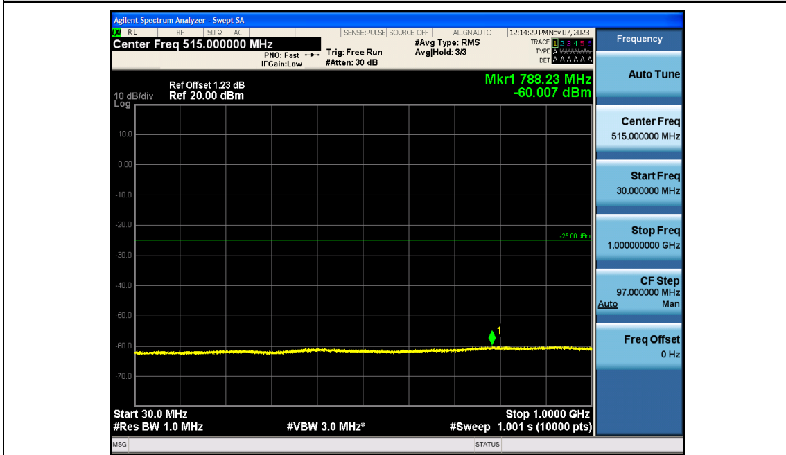
Band7-10MHz-16QAM-21100-1RB#0-Range2:1000~26500MHz
