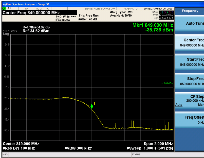
Band5-5MHz-16QAM-20625-1RB#24
