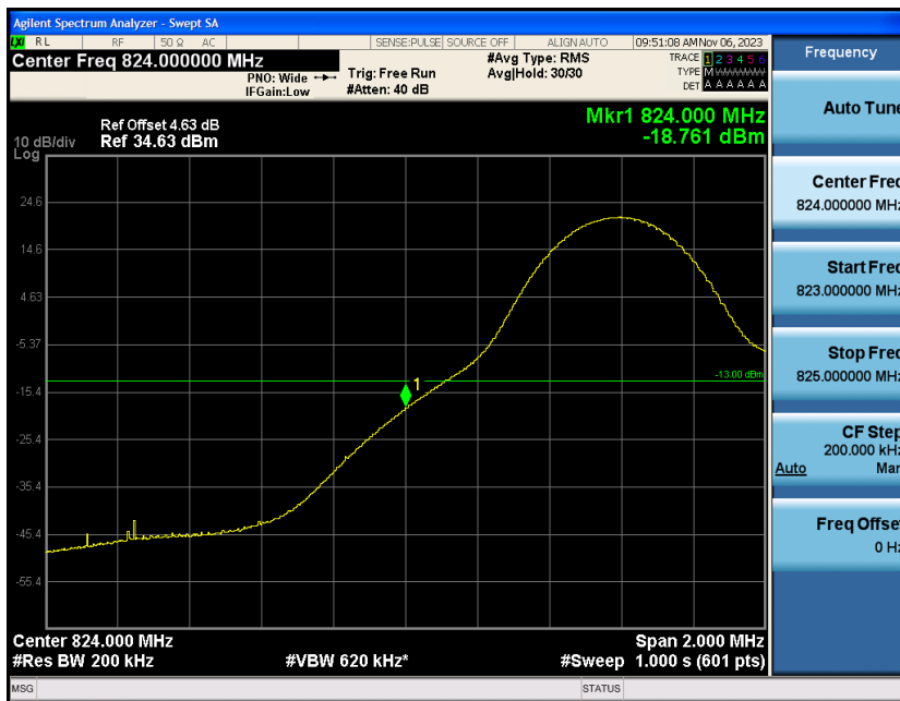
Band5-10MHz-16QAM-20450-1RB#49
