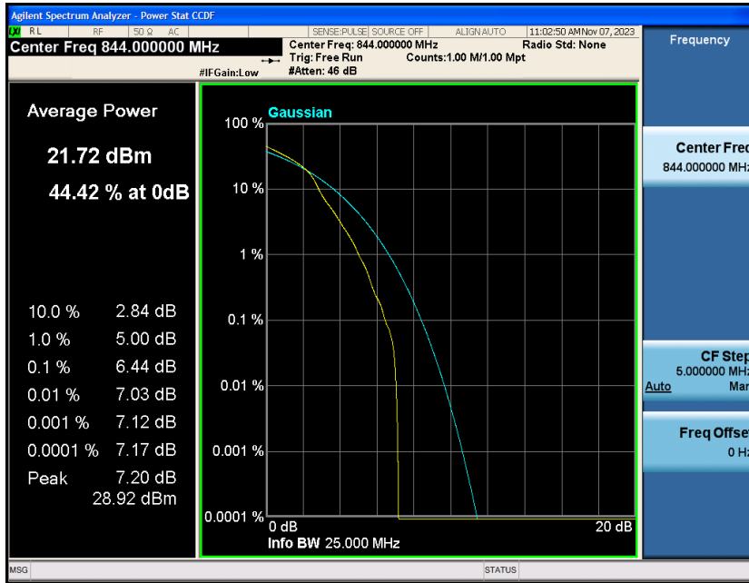
Band5-10MHz-16QAM-20600-50RB#0
