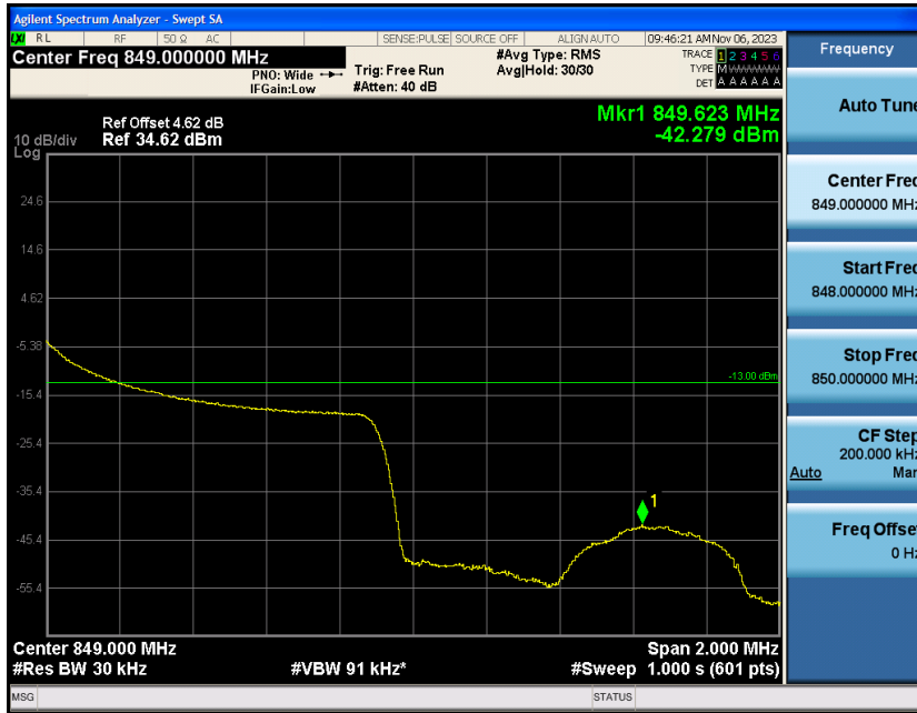
Band5-1.4MHz-QPSK-20643-1RB#5
