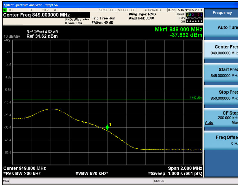
Band5-10MHz-QPSK-20600-1RB#49
