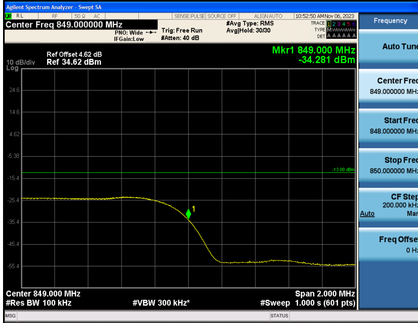
Band5-5MHz-QPSK-20625-1RB#24
