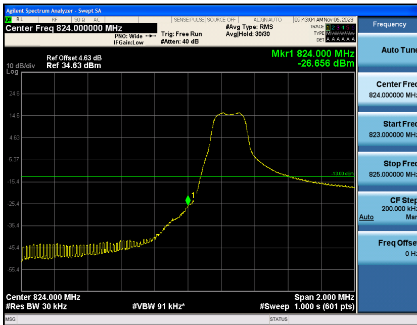
Band5-1.4MHz-16QAM-20407-1RB#5
