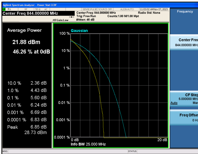
Band5-10MHz-16QAM-20450-1RB#0
