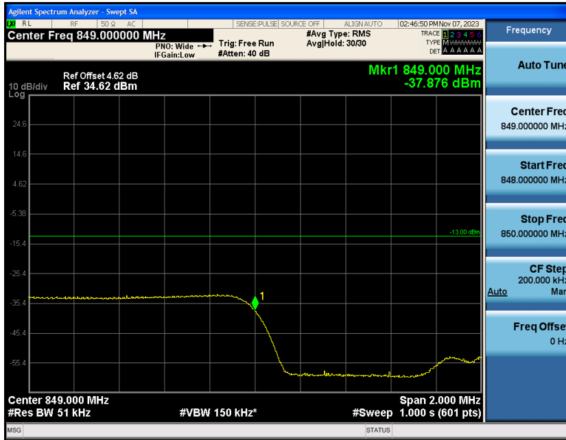
Band5-3MHz-16QAM-20635-1RB#14
