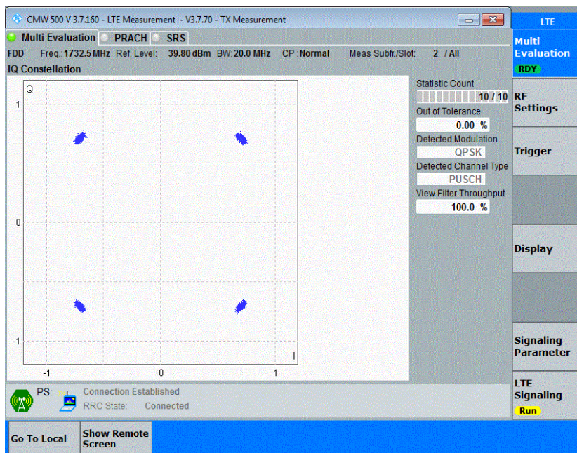
Band4-20MHz-QPSK-20300-100RB#0
