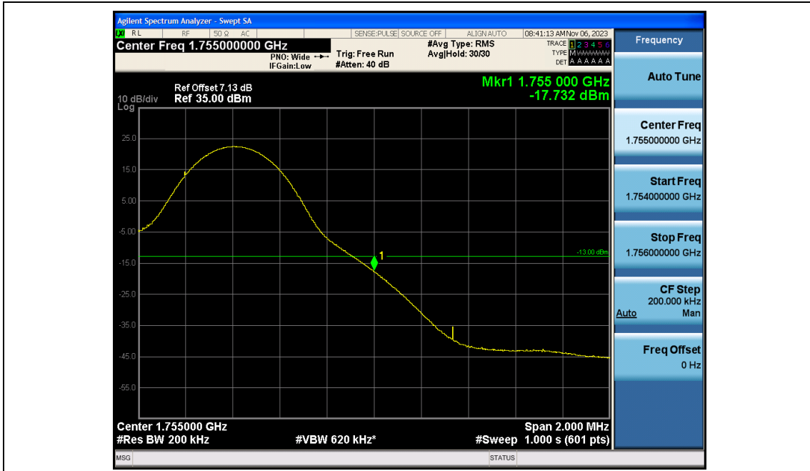
Band4-10MHz-16QAM-20350-50RB#0
