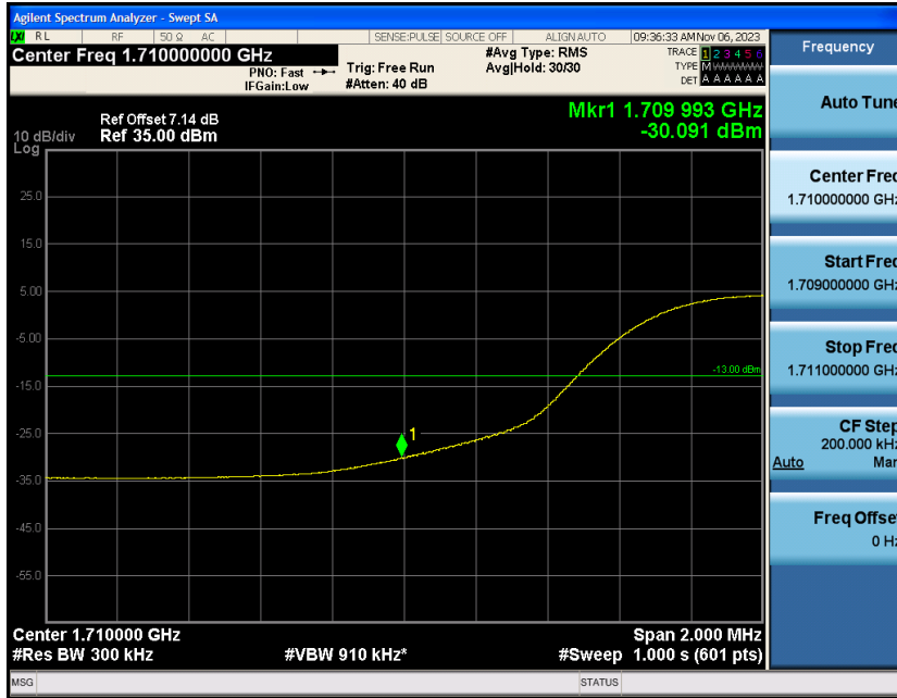
Band4-15MHz-16QAM-20325-1RB#0
