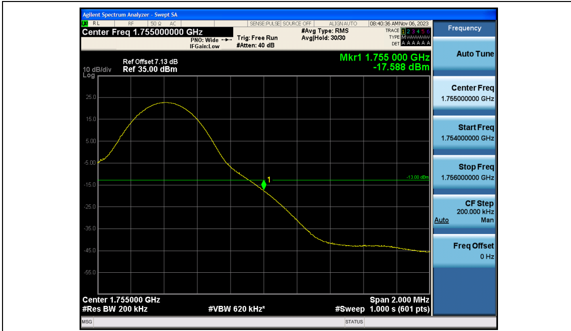
Band4-10MHz-QPSK-20350-50RB#0
