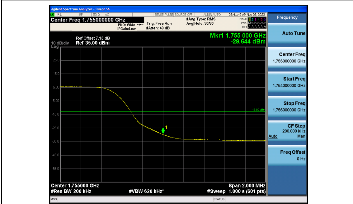
Band4-10MHz-16QAM-20000-1RB#0
