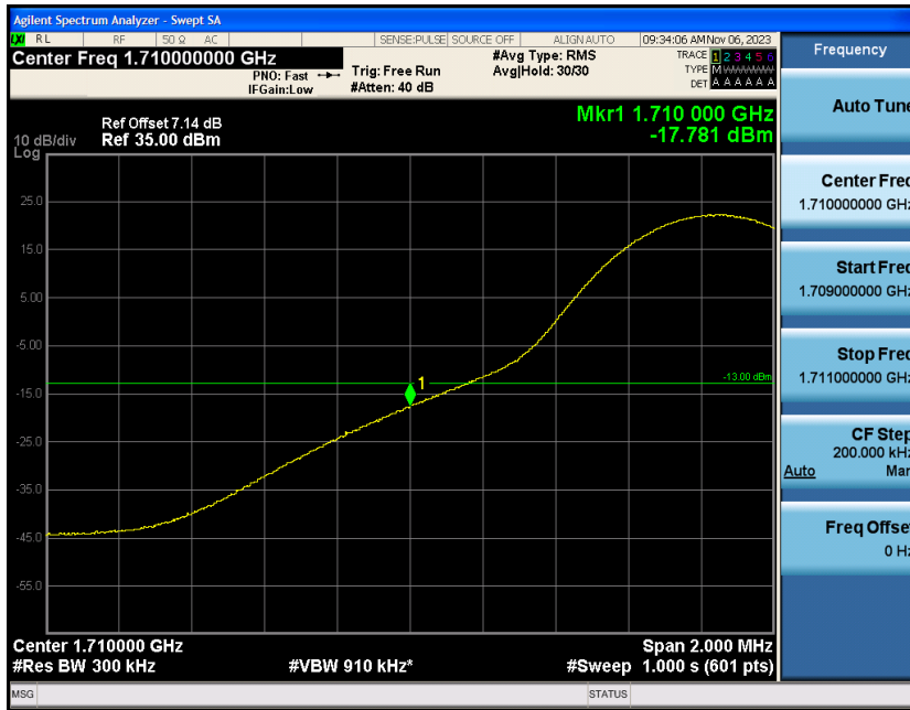
Band4-15MHz-16QAM-20025-1RB#74
