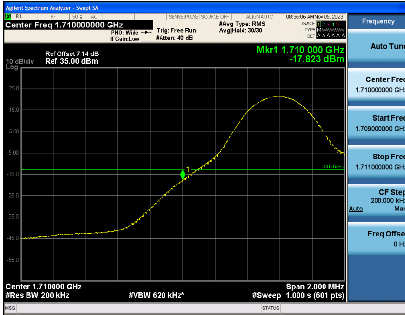
Band4-10MHz-16QAM-20000-1RB#49
