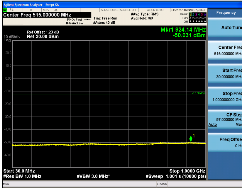
Band4-3MHz-16QAM-20385-1RB#0-Range2:1000~20000MHz
