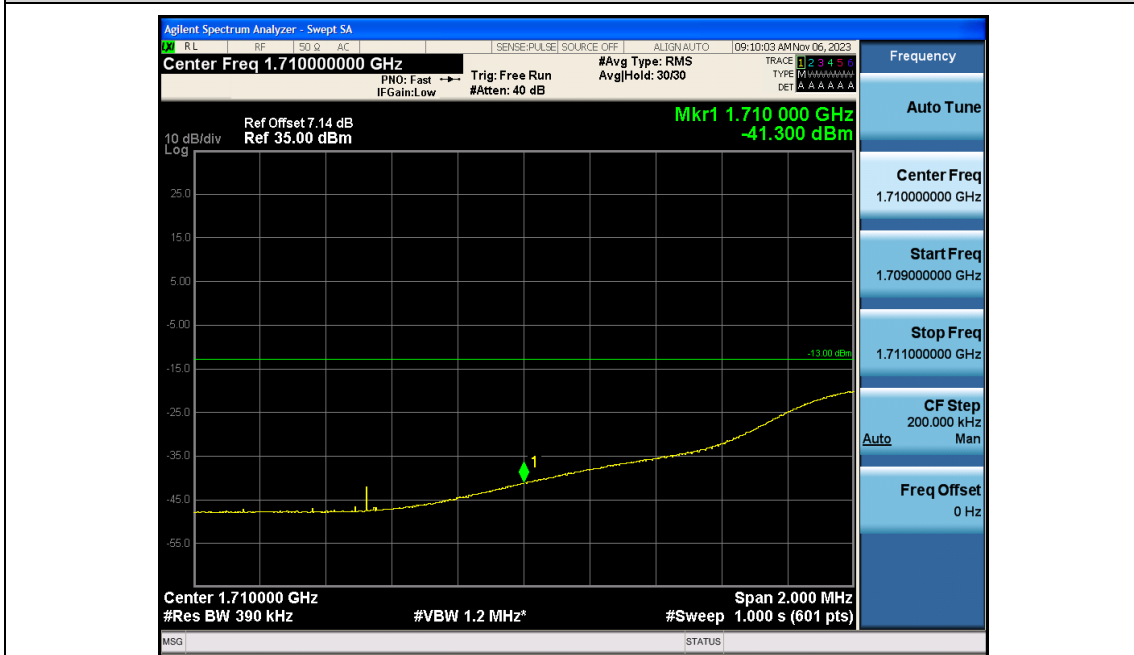
Band4-20MHz-16QAM-20050-100RB#0
