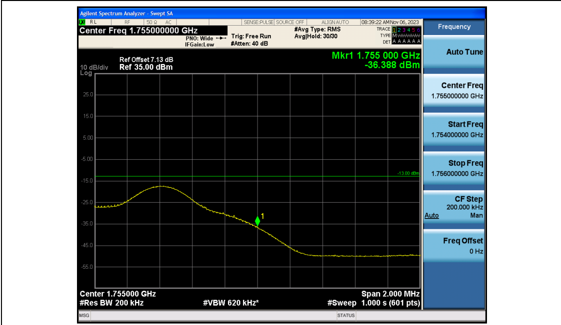
Band4-10MHz-QPSK-20350-1RB#49
