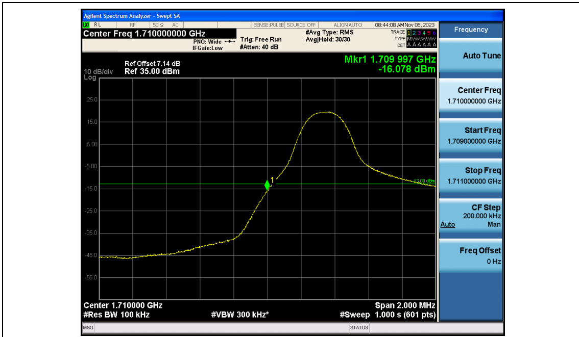
Band4-5MHz-16QAM-19975-1RB#24
