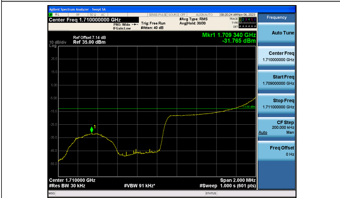
Band4-1.4MHz-16QAM-19957-6RB#0
