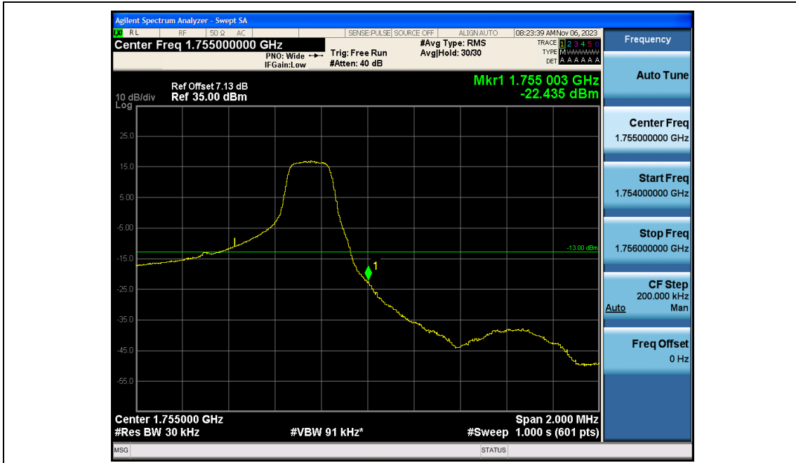
Band4-1.4MHz-QPSK-20393-6RB#0
