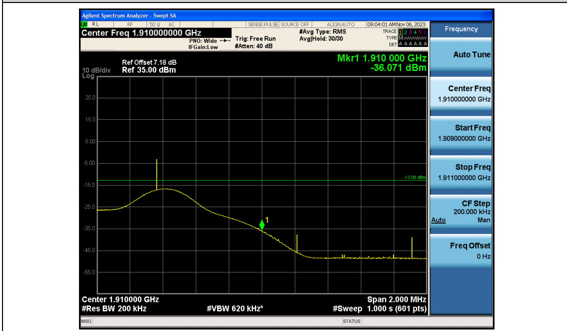
Band2-10MHz-QPSK-19150-1RB#49
