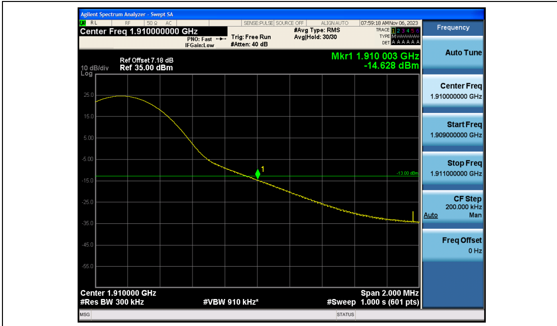
Band2-15MHz-QPSK-19125-75RB#0
