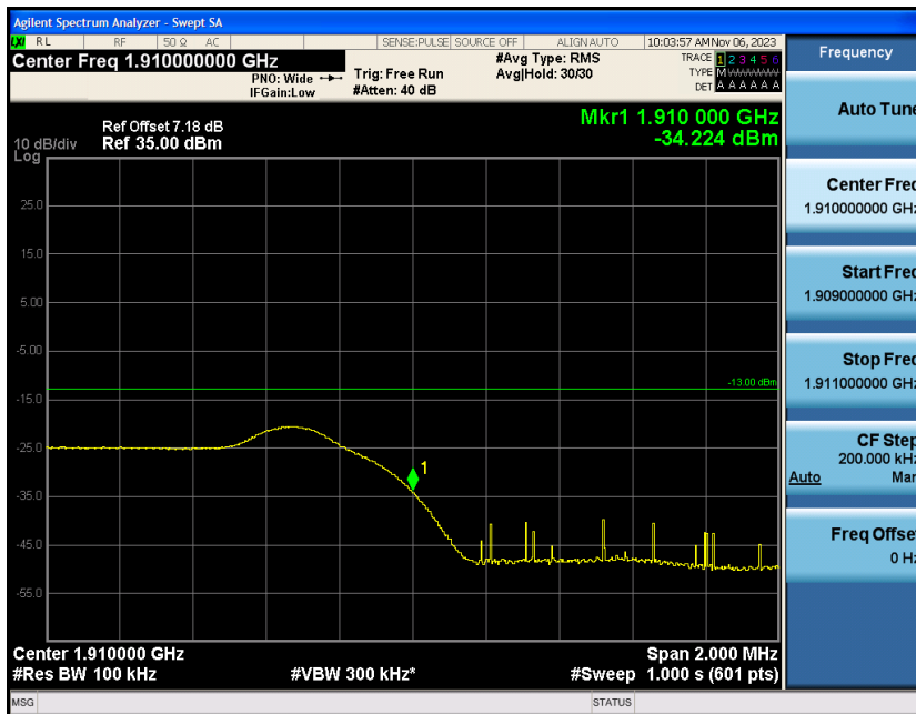
Band2-5MHz-16QAM-19175-1RB#24
