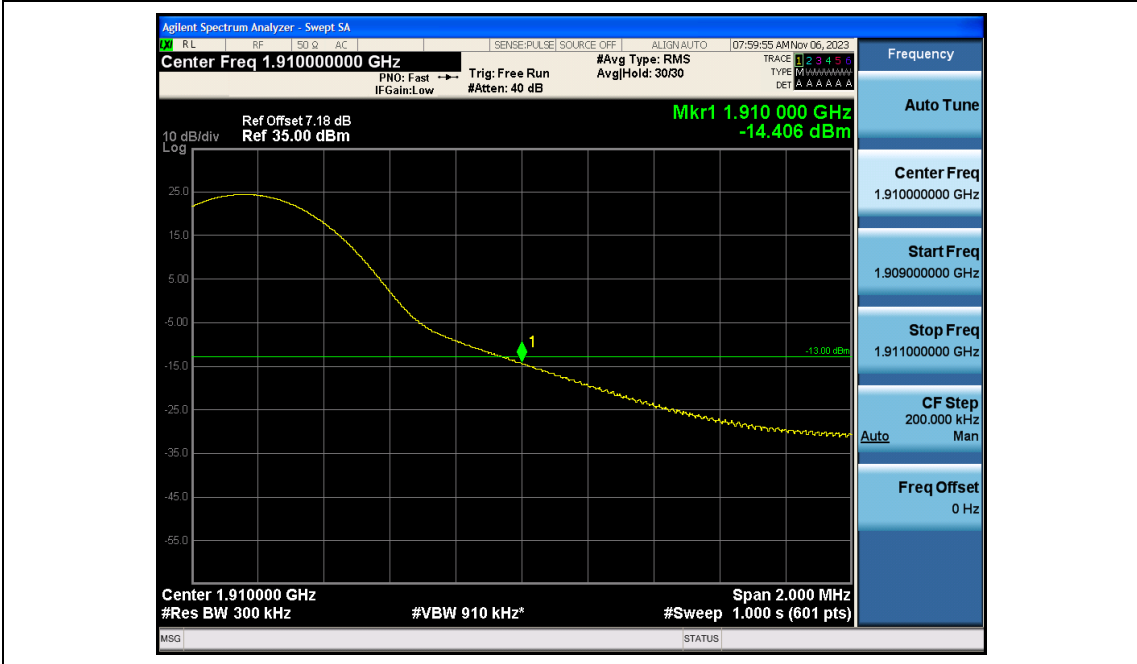
Band2-15MHz-16QAM-19125-75RB#0
