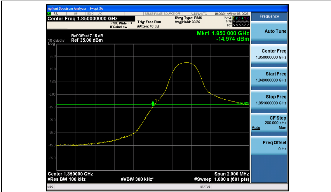
Band2-5MHz-16QAM-18625-1RB#24
