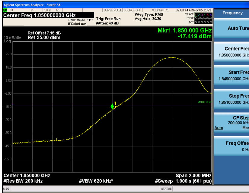
Band2-10MHz-16QAM-18650-1RB#49
