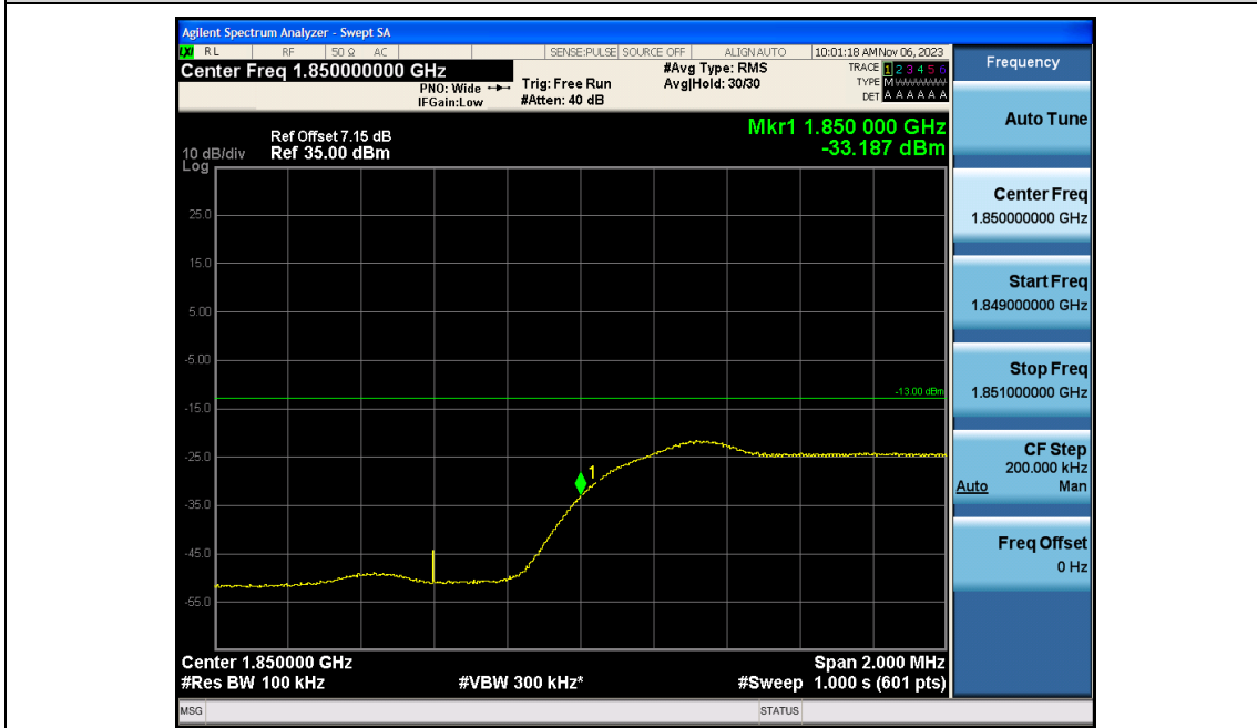
Band2-5MHz-16QAM-18625-25RB#0
