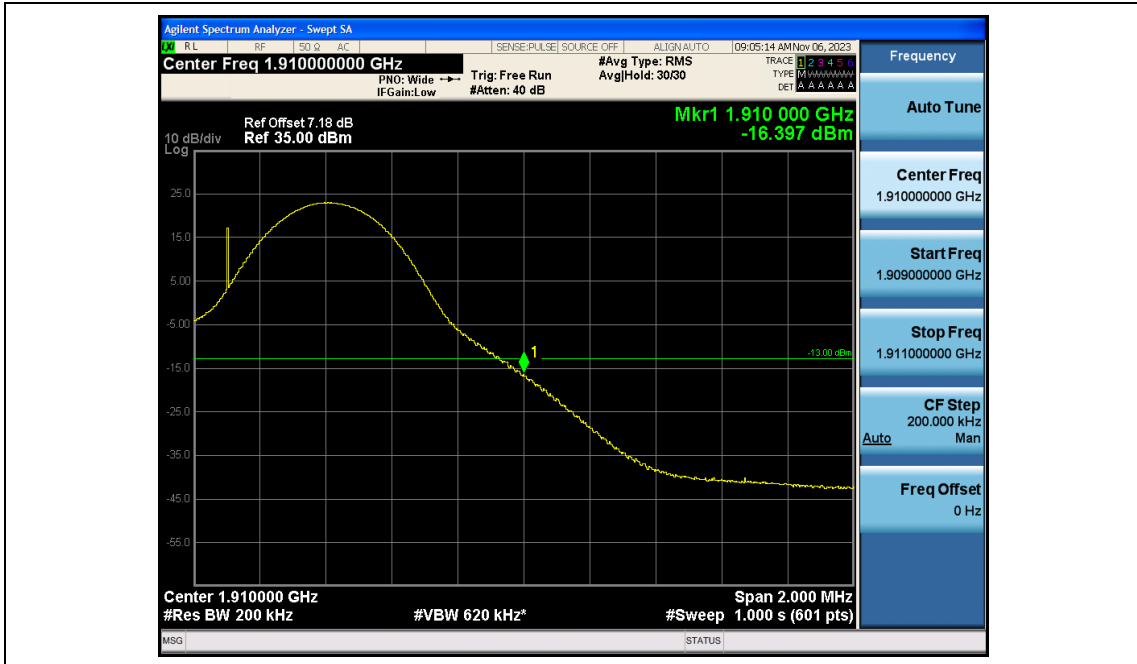
Band2-10MHz-QPSK-19150-50RB#0
