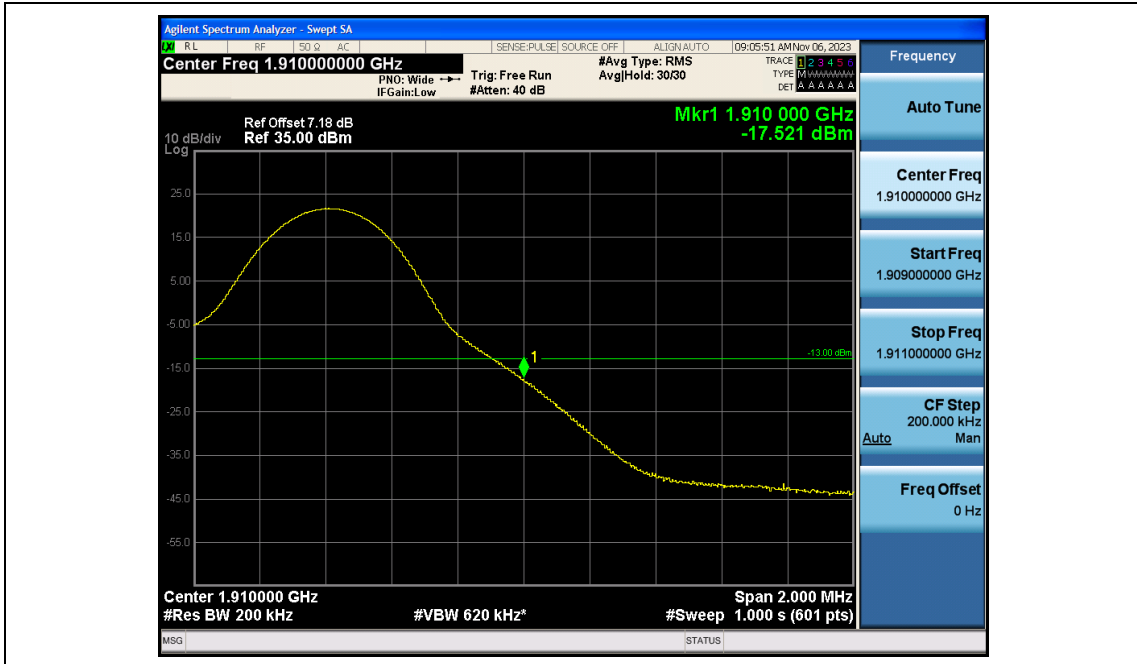
Band2-10MHz-16QAM-19150-50RB#0
