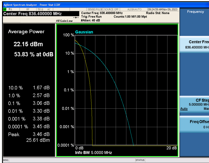
Band5-4233
