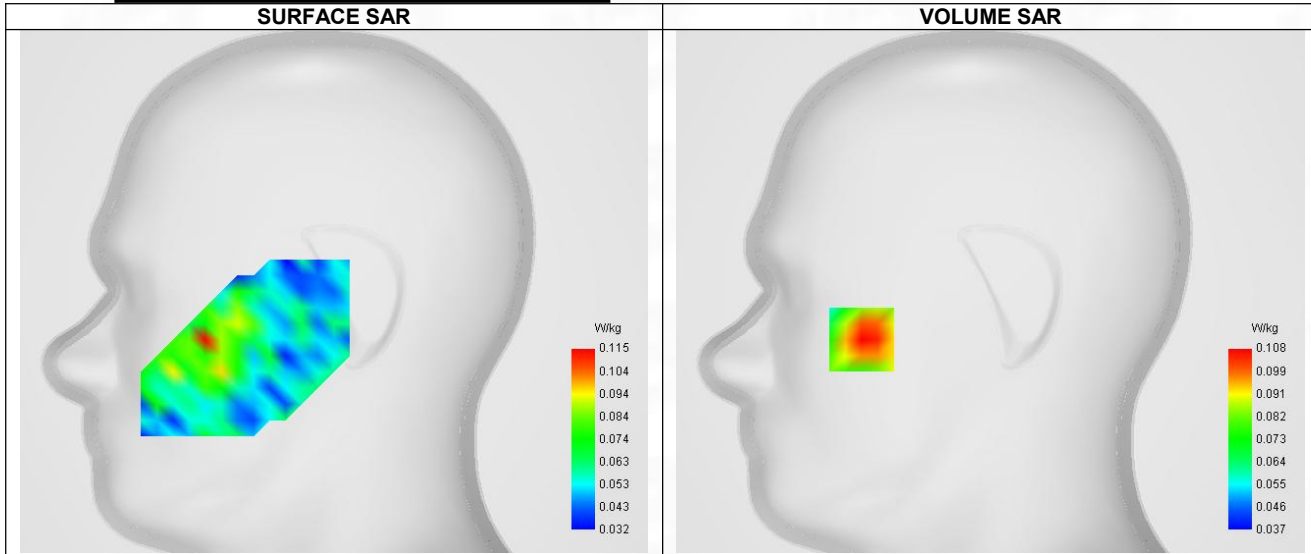
Maximum location: X=-64.00, Y=-24.00 ; SAR Peak: 0.16 W/kg
