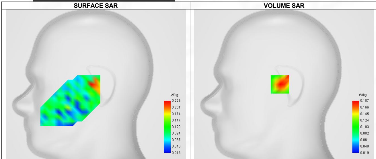
Maximum location: X=-7.00, Y=0.00 ; SAR Peak: 0.32 W/kg
