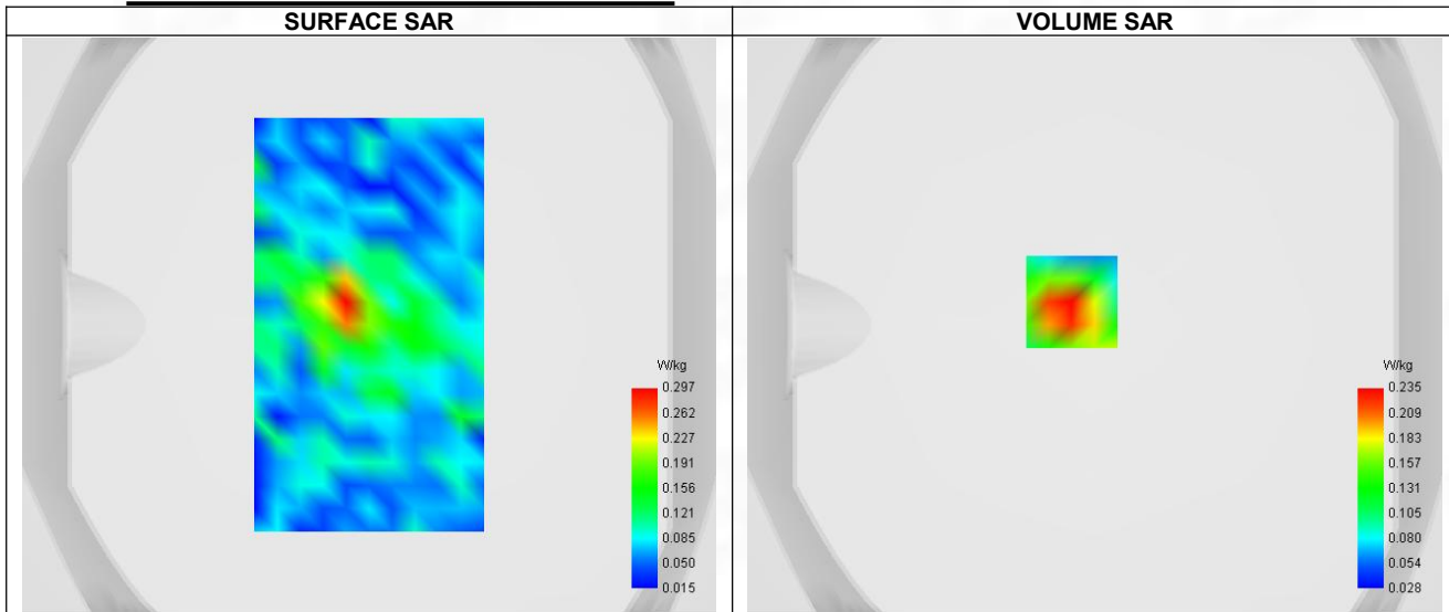
Maximum location: X=-8.00, Y=8.00 ; SAR Peak: 0.34 W/kg
