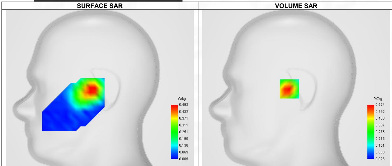
Maximum location: X=-11.00, Y=-2.00 ; SAR Peak: 0.83 W/kg
