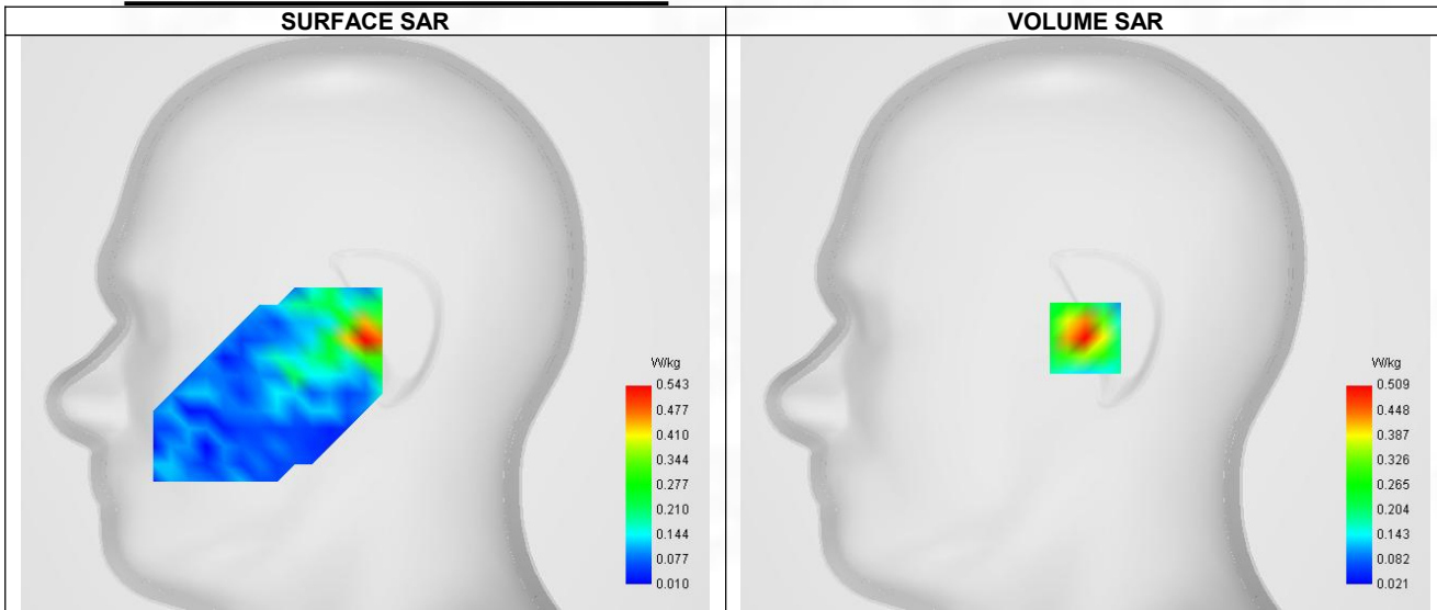
Maximum location: X=0.00, Y=-7.00 ; SAR Peak: 1.17 W/kg
