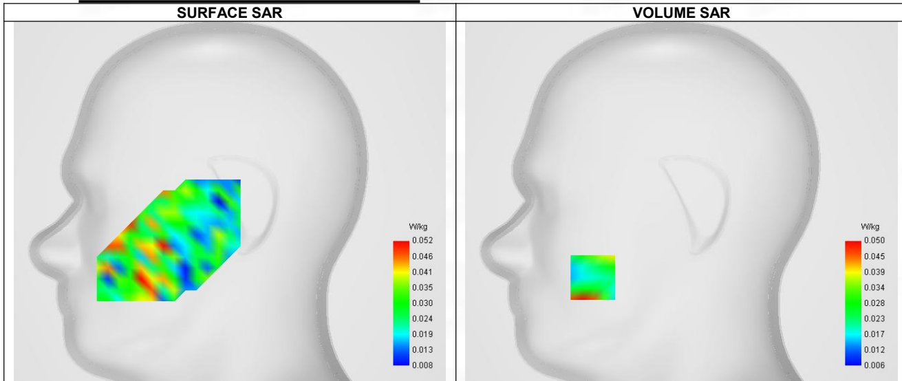
Maximum location: X=-64.00, Y=-55.00 ; SAR Peak: 0.11 W/kg
