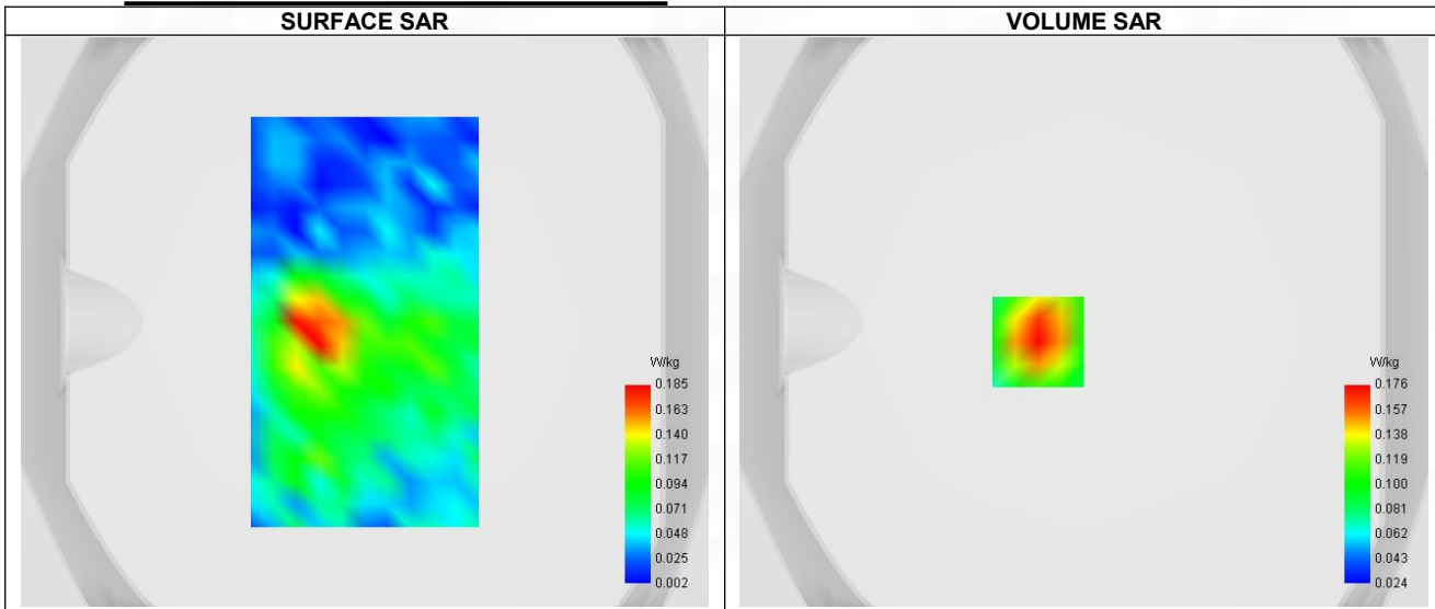
Maximum location: X=-16.00, Y=-7.00 ; SAR Peak: 0.27 W/kg
