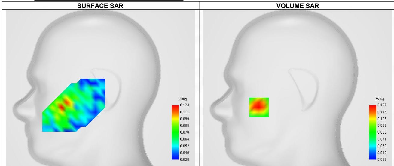
Maximum location: X=-64.00, Y=-32.00 ; SAR Peak: 0.19 W/kg
