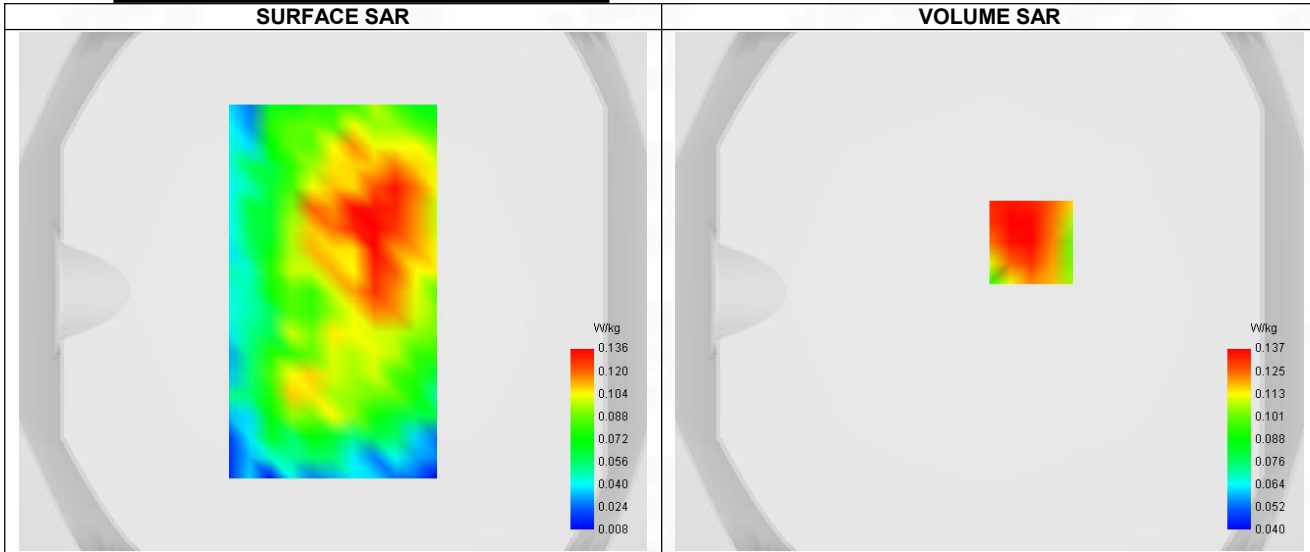
Maximum location: X=16.00, Y=19.00 ; SAR Peak: 0.19 W/kg
