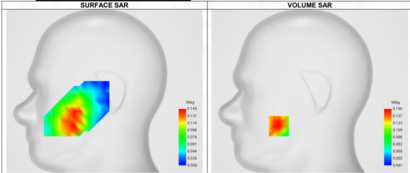
Maximum location: X=-49.00, Y=-56.00 ; SAR Peak: 0.21 W/kg
