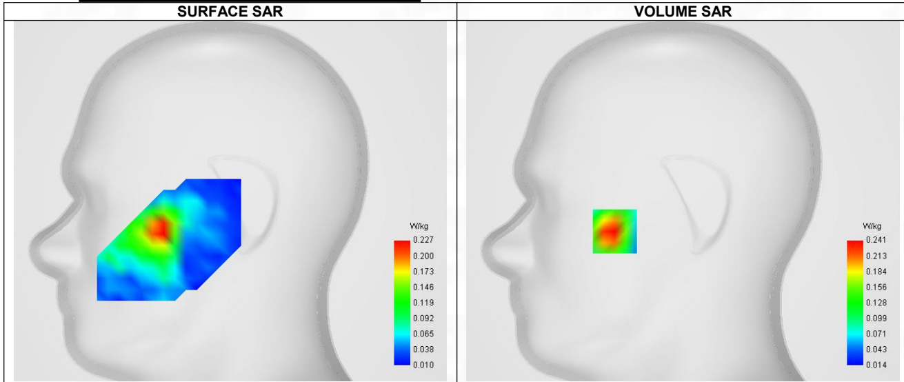
Maximum location: X=-49.00, Y=-22.00 ; SAR Peak: 0.36 W/kg
