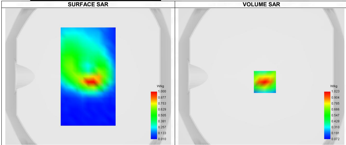
Maximum location: X=5.00, Y=-8.00 ; SAR Peak: 1.54 W/kg
