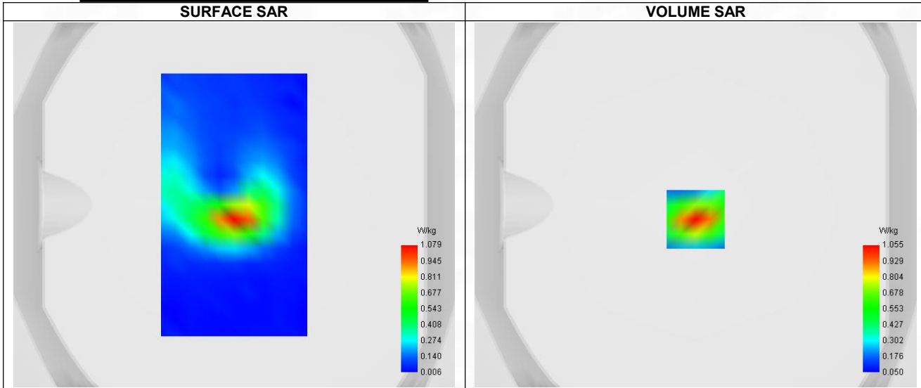
Maximum location: X=0.00, Y=-8.00 ; SAR Peak: 1.58 W/kg
