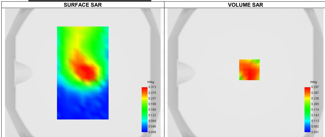
Maximum location: X=6.00, Y=5.00 ; SAR Peak: 0.43 W/kg
