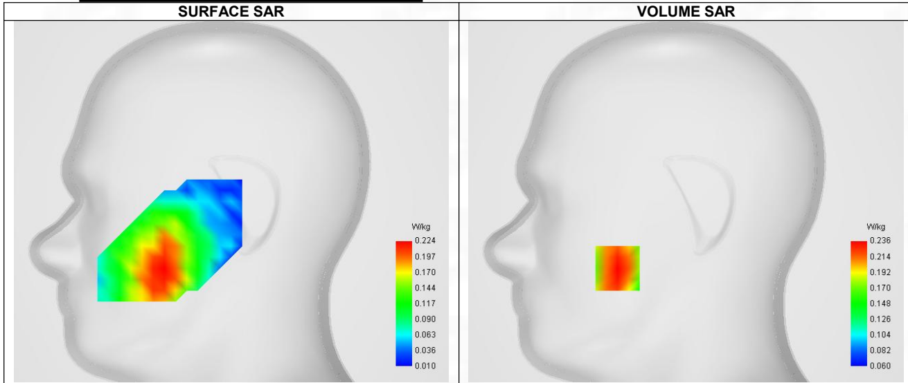
Maximum location: X=-49.00, Y=-48.00 ; SAR Peak: 0.29 W/kg
