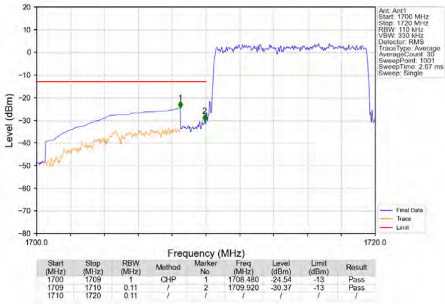
Band66_10MHz_16QAM_LCH_1715MHz_RB_50_0_NTNV
