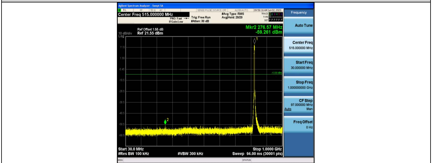
Band5-4132-30~1000MHz
