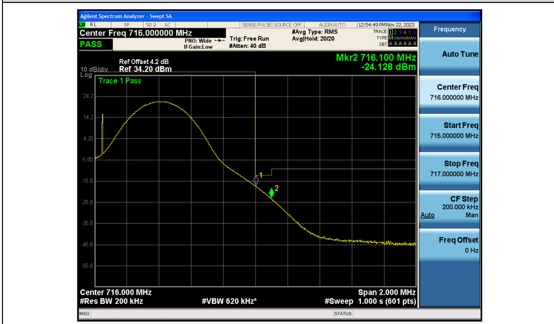
Band12-10MHz-16QAM-23130-50RB#0
