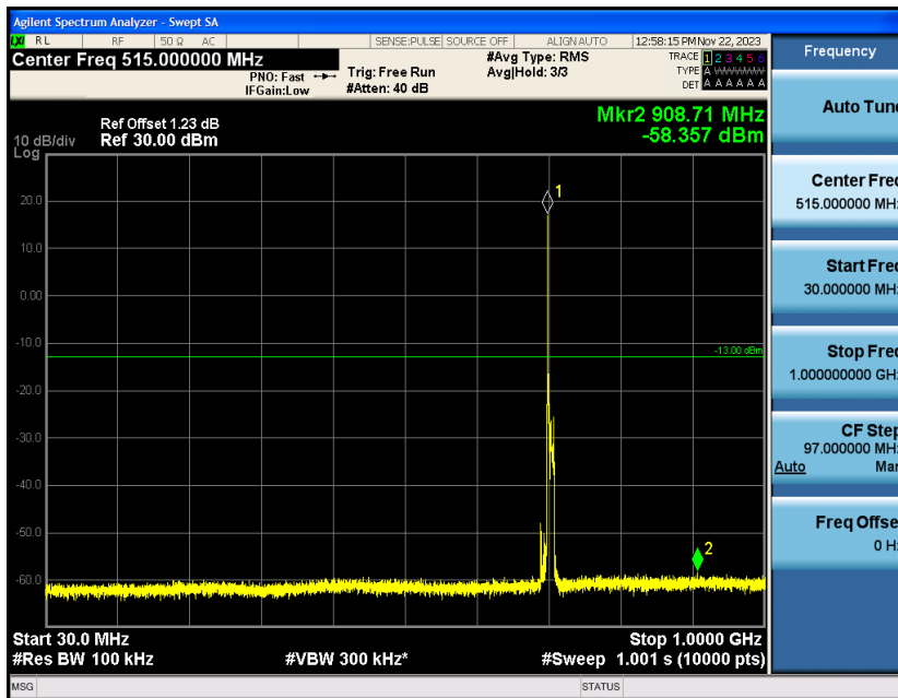
Band12-10MHz-QPSK-23130-1RB#0-Range2:1000~10000MHz
