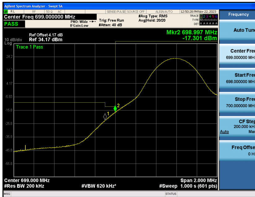
Band12-10MHz-QPSK-23060-1RB#49
