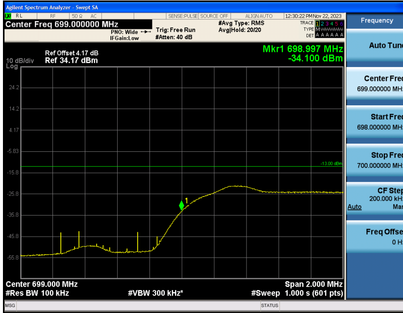
Band12-5MHz-16QAM-23035-25RB#0
