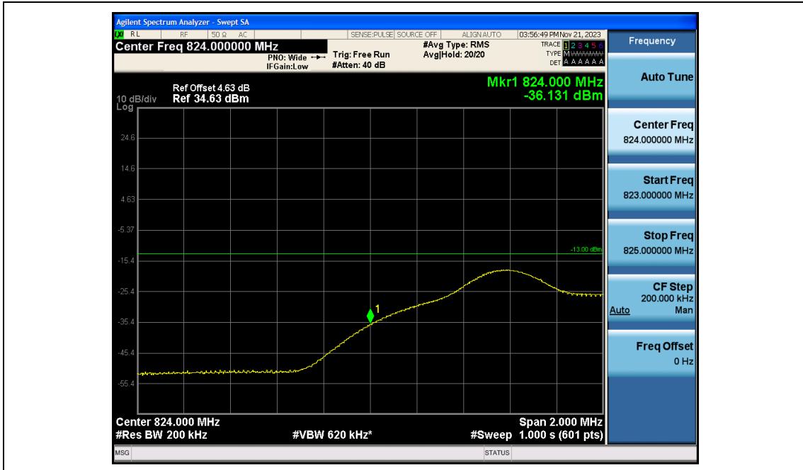
Band5-10MHz-16QAM-20450-50RB#0
