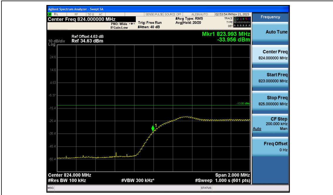
Band5-5MHz-16QAM-20425-25RB#0
