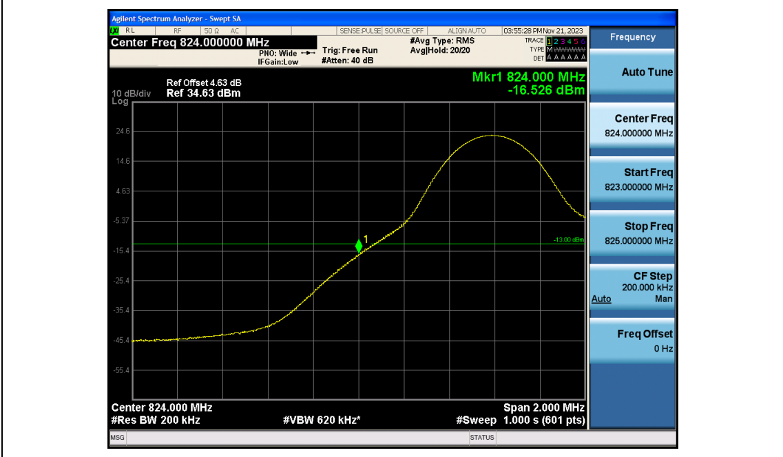
Band5-10MHz-QPSK-20450-1RB#49
