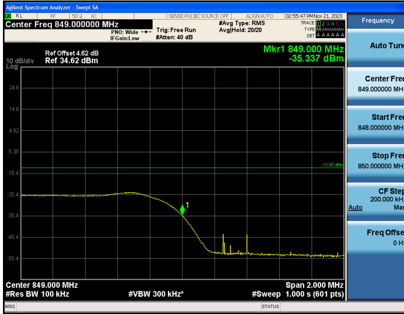
Band5-5MHz-16QAM-20625-1RB#24
