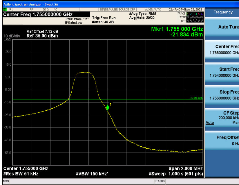
Band4-3MHz-QPSK-20385-15RB#0
