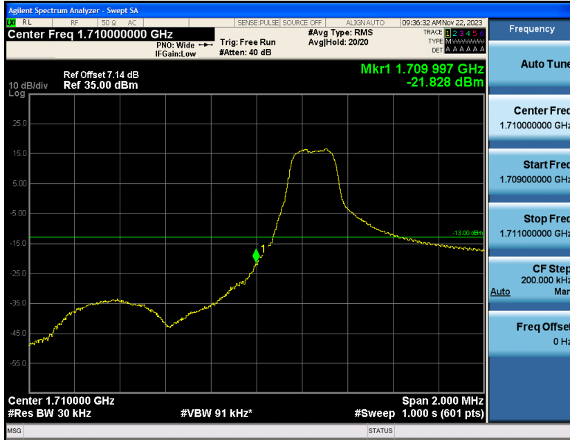
Band4-1.4MHz-16QAM-19957-1RB#5
