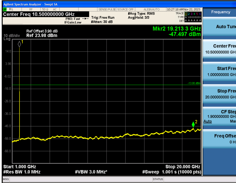
Band4-5MHz-16QAM-19975-1RB#0-Range1:30~100MHz
