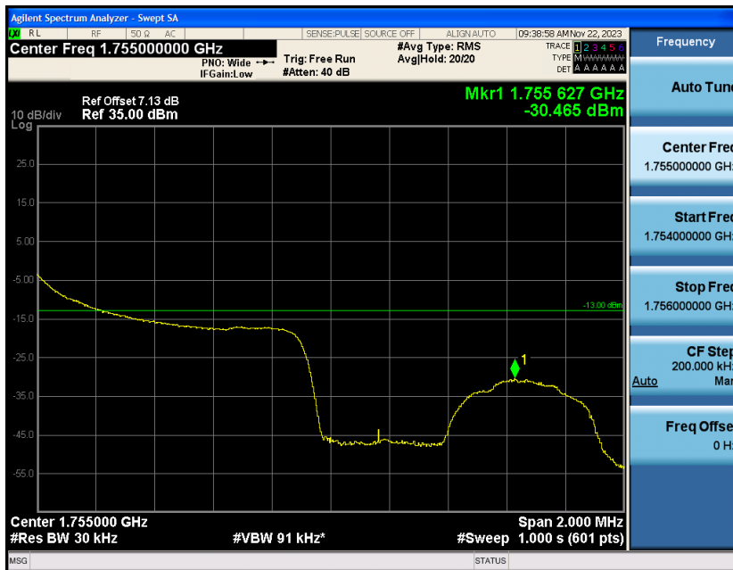
Band4-1.4MHz-QPSK-20393-1RB#5
