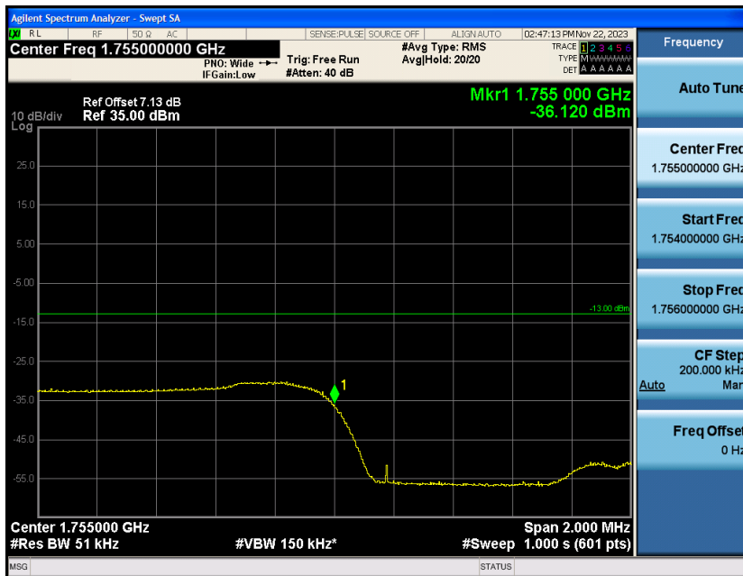
Band4-3MHz-16QAM-20385-1RB#14
