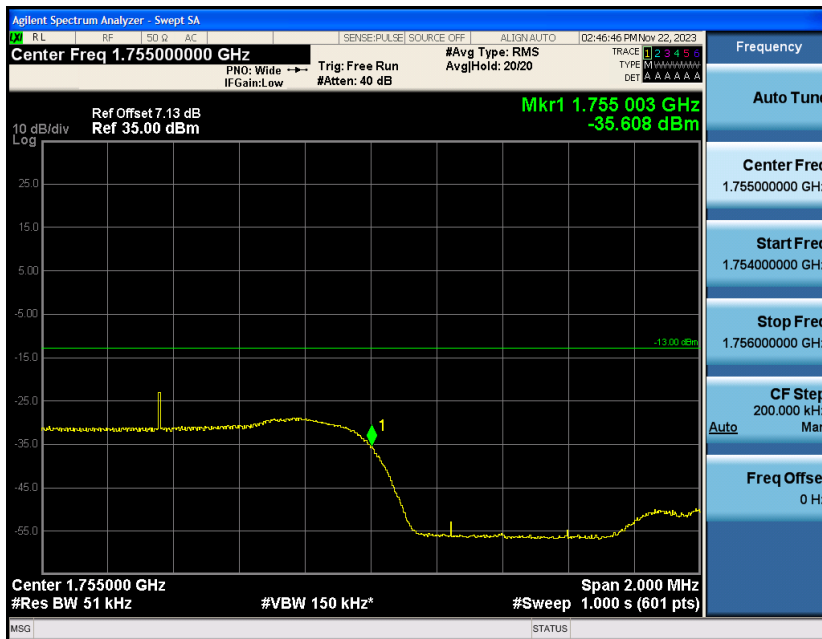
Band4-3MHz-QPSK-20385-1RB#14
