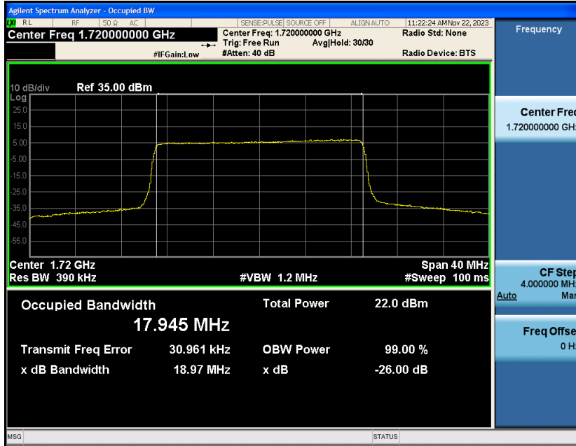
Band4-20MHz-QPSK-20175-100RB#0
