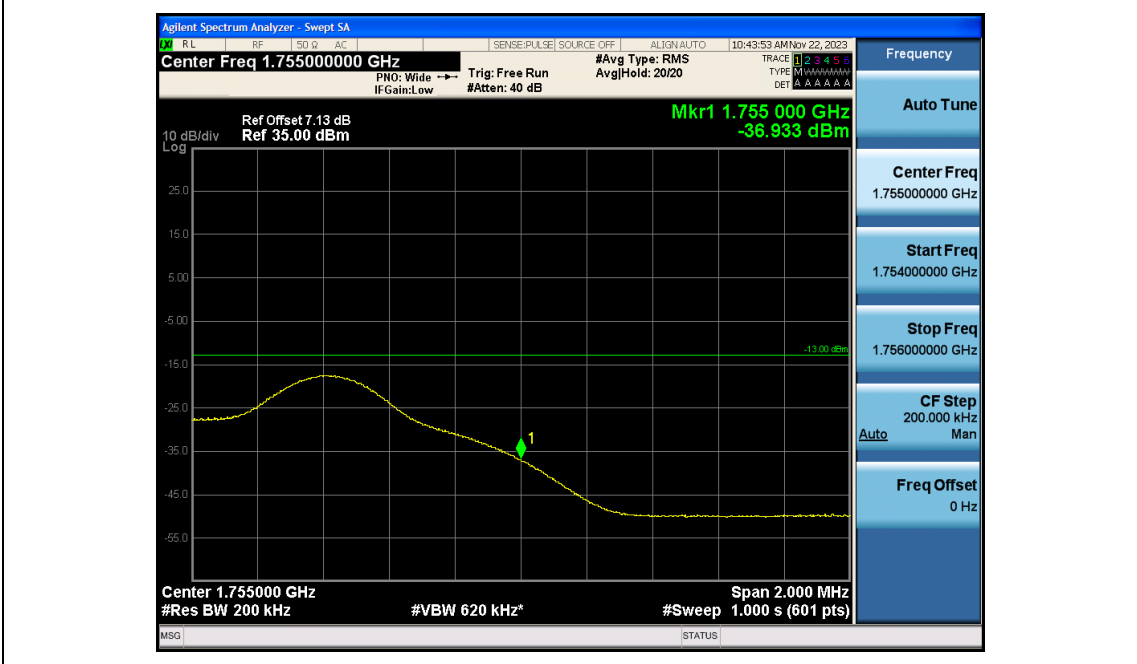
Band4-10MHz-QPSK-20350-1RB#49
