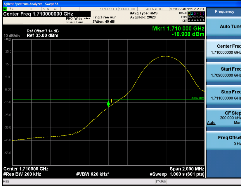
Band4-10MHz-16QAM-20000-1RB#49
