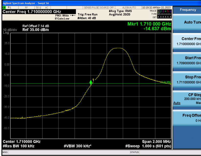
Band4-5MHz-QPSK-19975-1RB#24
