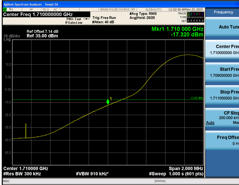
Band4-15MHz-QPSK-20025-1RB#74
