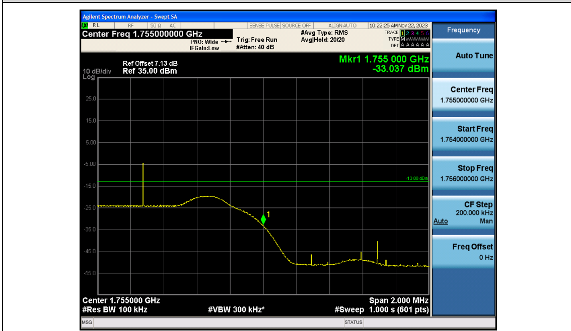
Band4-5MHz-QPSK-20375-1RB#24
