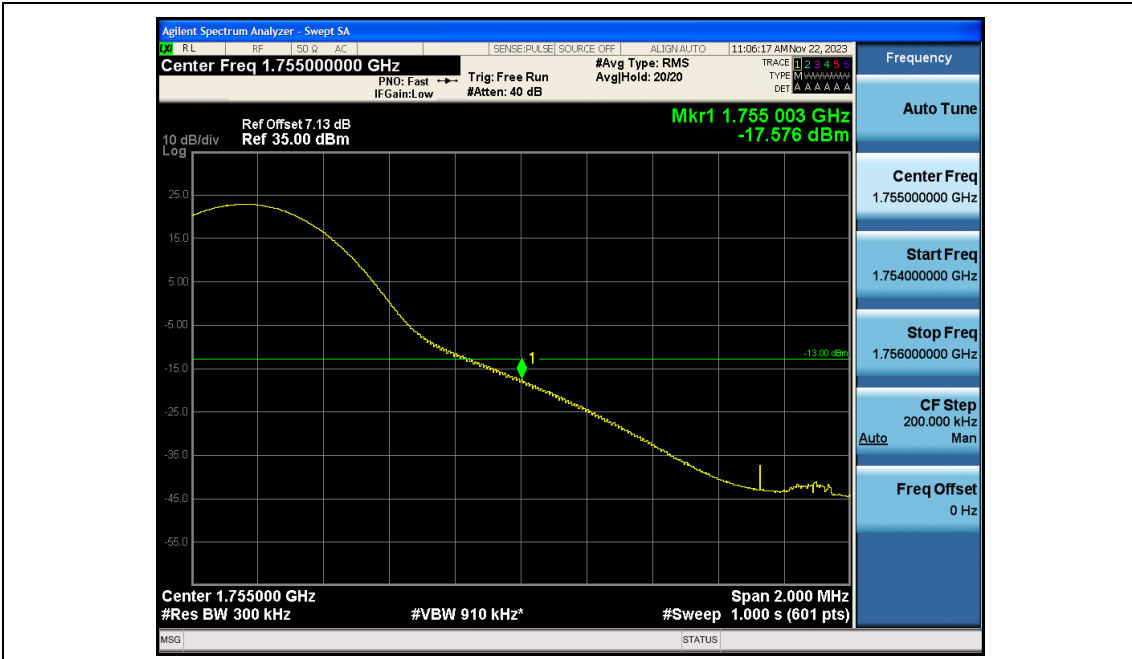
Band4-15MHz-QPSK-20325-75RB#0
