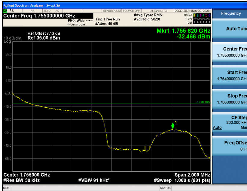
Band4-1.4MHz-16QAM-20393-1RB#5
