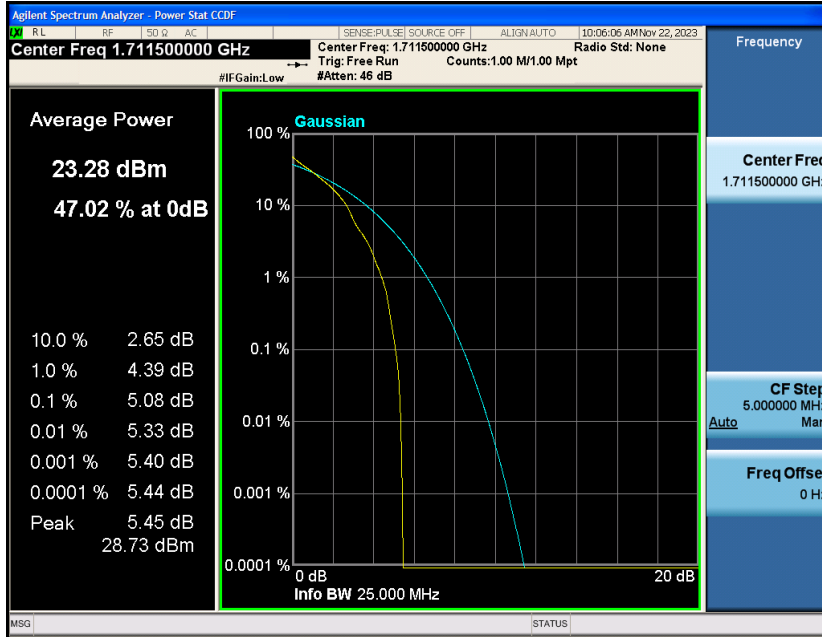
Band4-3MHz-QPSK-19965-15RB#0
