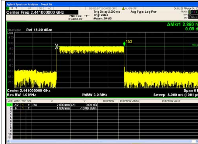
Pulse Width
