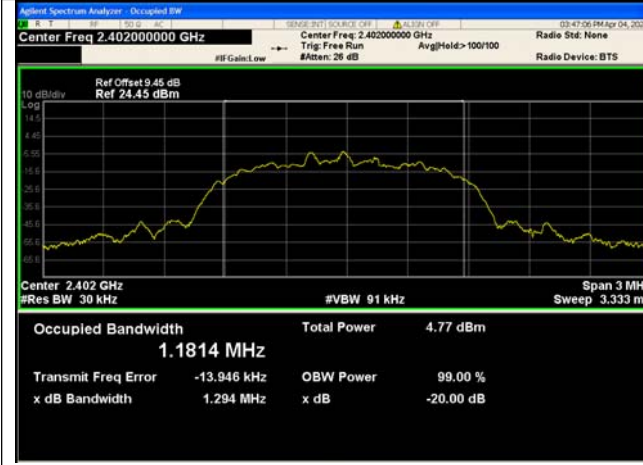
8DPSK_3-DH5_Channel 0
