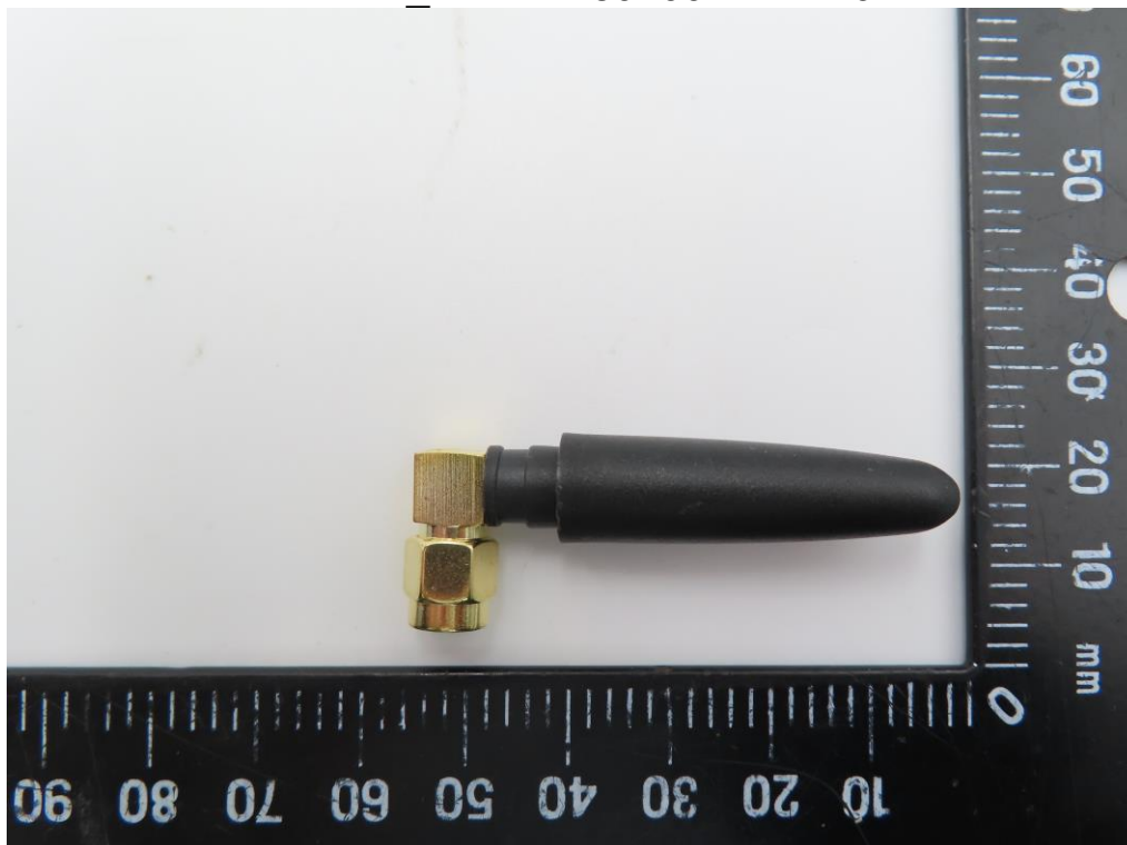
Antenna_RFDPA480700SMABX01
