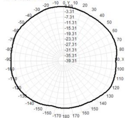
Total(H-XY), Max= 0.69dBi, CirD=6.01
