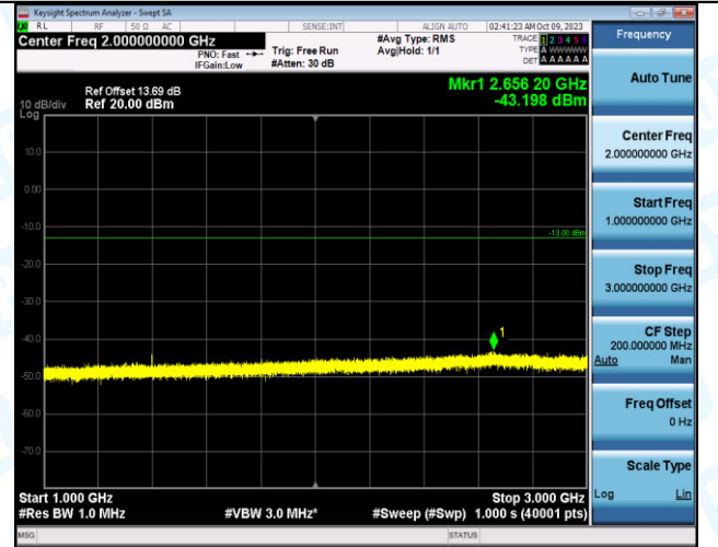
Band12_5MHz_QPSK_23035_1RB#0_1000~3000_1000~3000
