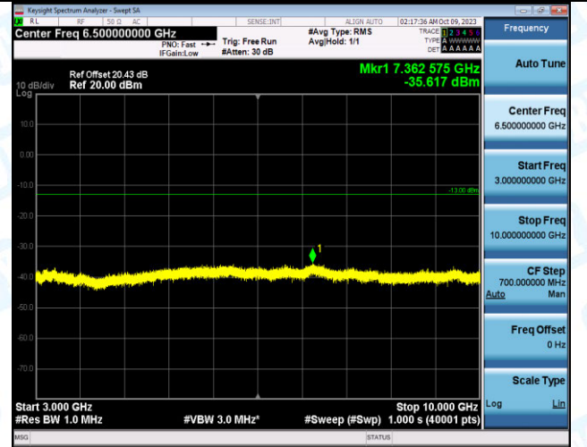
Band12_3MHz_16QAM_23165_15RB#0_3000~10000_30 00~10000
