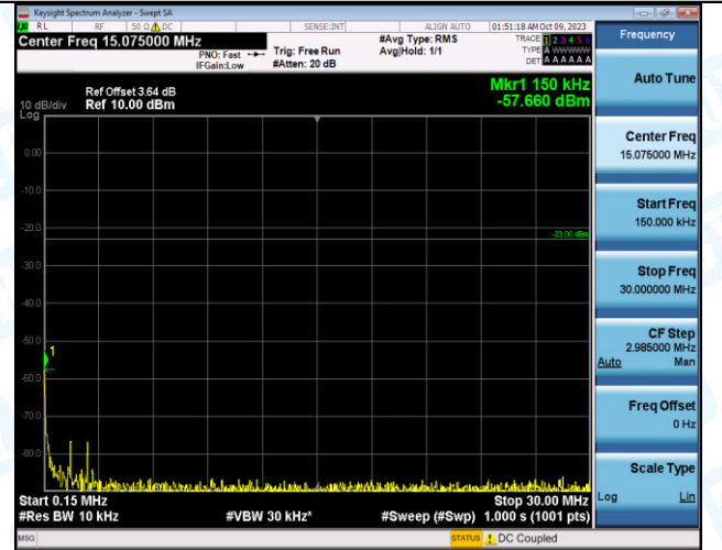
Band12_1.4MHz_QPSK_23173_6RB#0_0.15~30_0.15~30
