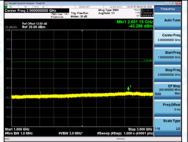
Band12_1.4MHz_QPSK_23095_1RB#0_1000~3000_1000 ~3000
