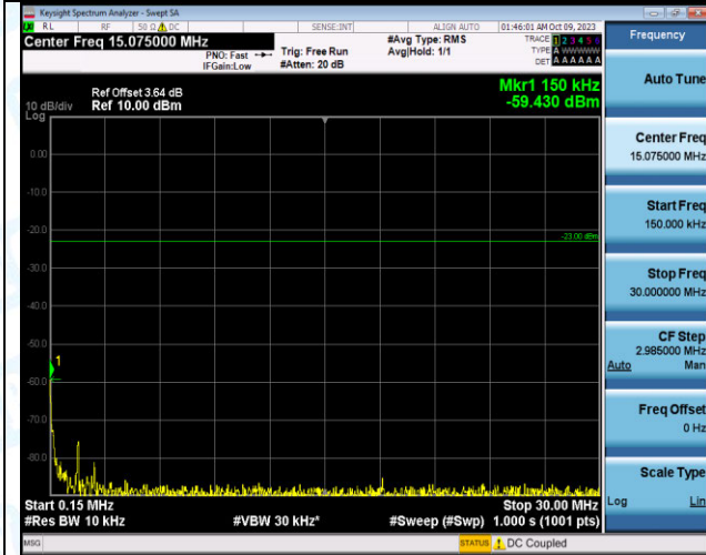
Band12_1.4MHz_16QAM_23017_6RB#0_0.15~30_0.15~ 30
