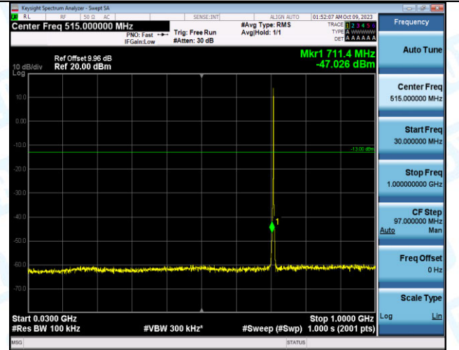
Band12_1.4MHz_16QAM_23173_6RB#0_30~1000_30~10 00
