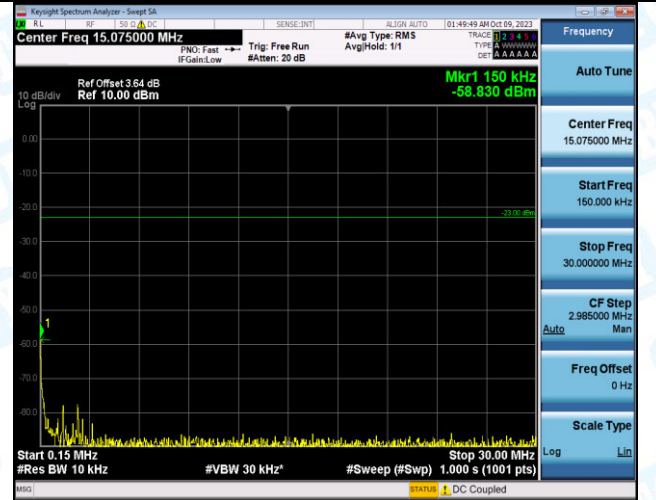
Band12_1.4MHz_QPSK_23173_1RB#0_0.15~30_0.15~30
