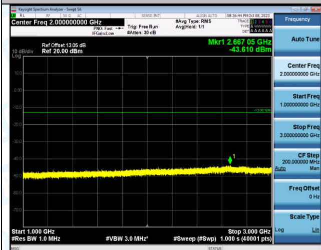
Band4_15MHz_QPSK_20025_1RB#74_1000~3000_1000 ~3000
