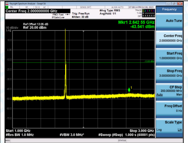
Band4_10MHz_QPSK_20350_1RB#0_1000~3000_1000~3000
