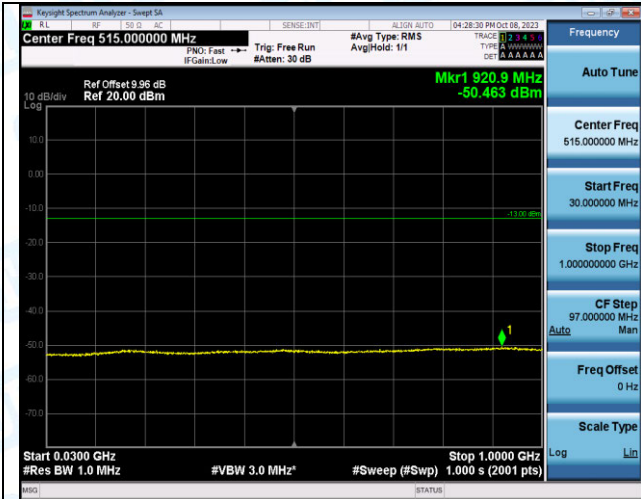
Band4_5MHz_QPSK_20375_1RB#0_30~1000_30~1000
