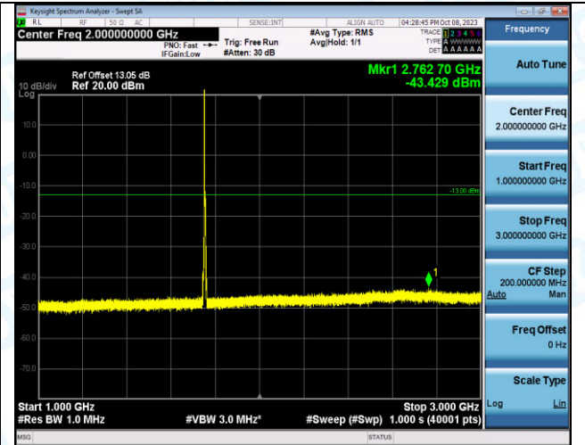
Band4_5MHz_QPSK_20375_1RB#0_1000~3000_1000~3000
