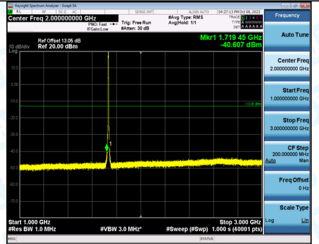
Band4_5MHz_QPSK_20175_25RB#0_1000~3000_1000~3000
