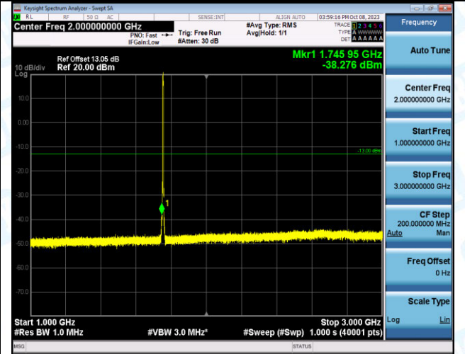
Band4_3MHz_QPSK_20385_15RB#0_1000~3000_1000~3000
