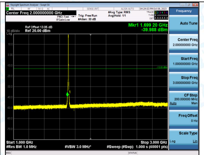
Band4_5MHz_QPSK_19975_25RB#0_1000~3000_1000~3000
