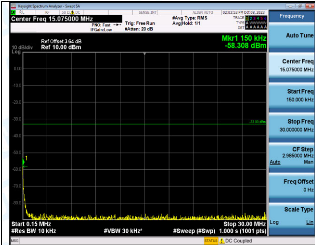
Band2_20MHz_16QAM_18900_1RB#99_0.15~30_0.15~3 0
