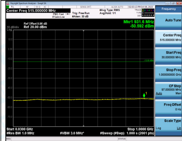
Band2_20MHz_QPSK_18900_1RB#99_30~1000_30~100 0
