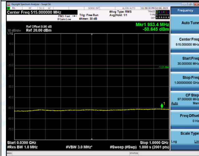
Band2_20MHz_QPSK_18900_1RB#0_30~1000_30~1000
