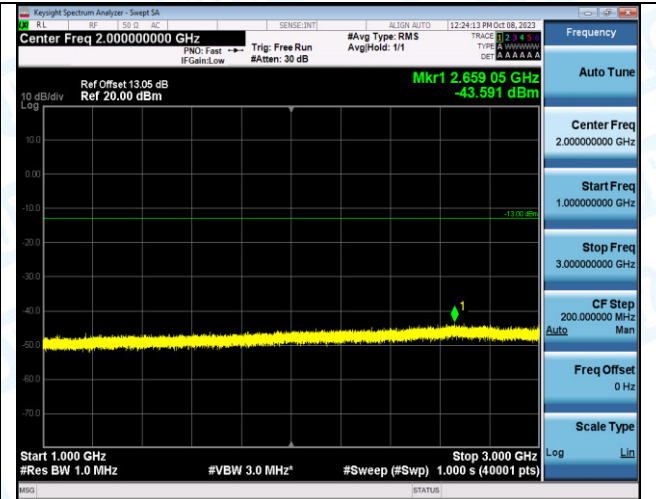
Band2_15MHz_16QAM_19125_1RB#74_1000~3000_1000~3000
