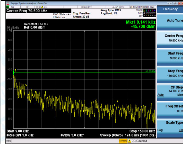
Band2_20MHz_QPSK_18900_1RB#0_0.009~0.15_0.009~0.15
