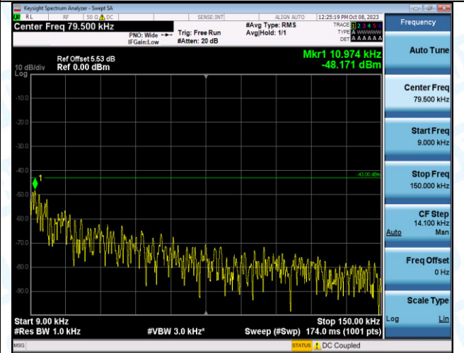
Band2_15MHz_QPSK_18675_75RB#0_0.009~0.15_0.009~0.15
