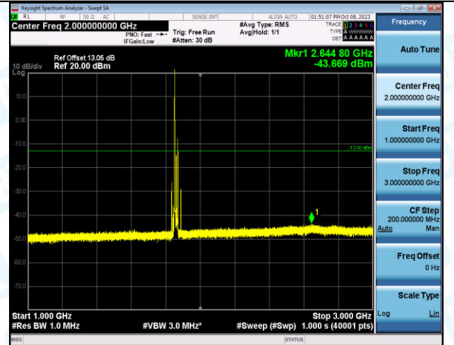
Band2_20MHz_QPSK_18700_1RB#0_1000~3000_1000~3000
