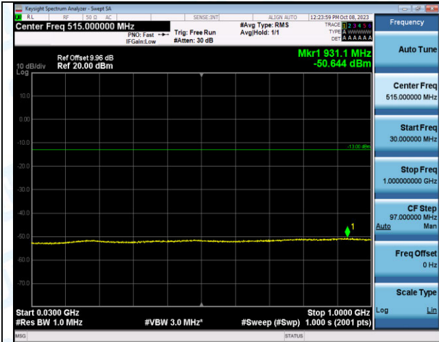
Band2_15MHz_16QAM_19125_1RB#74_30~1000_30~1000
