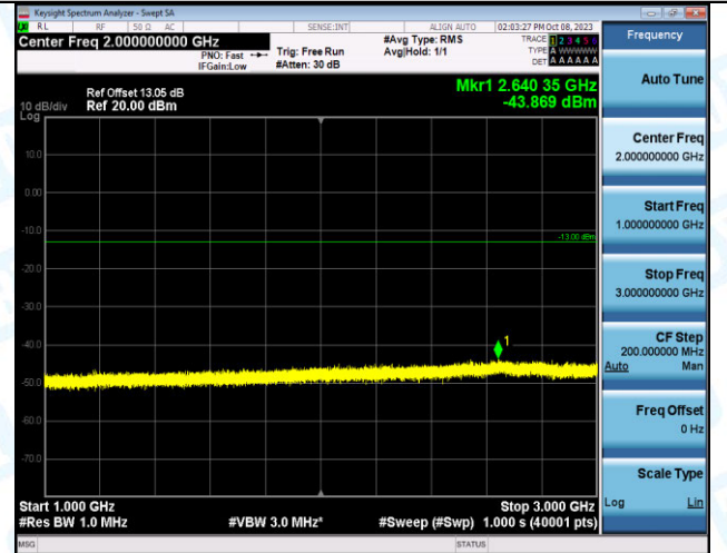
Band2_20MHz_QPSK_18900_1RB#99_1000~3000_1000 ~3000
