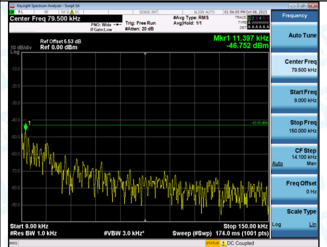
Band2_20MHz_16QAM_18700_1RB#99_0.009~0.15_0.009~0.15 9~0.15
