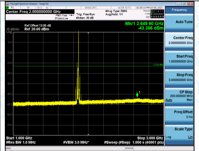
Band2_20MHz_QPSK_18700_1RB#99_1000~3000_1000~3000 ~3000
