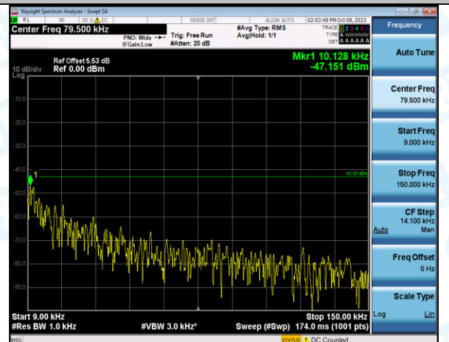
Band2_20MHz_16QAM_18900_1RB#99_0.009~0.15_0.00 9~0.15
