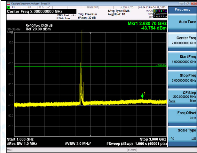
Band2_20MHz_16QAM_18900_1RB#99_1000~3000_100 0~3000
