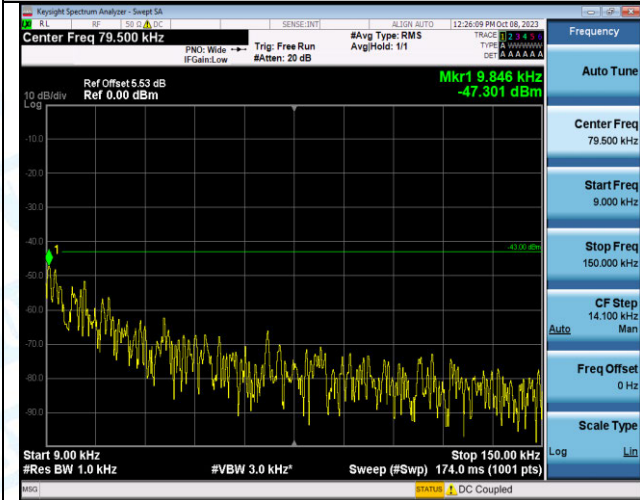
Band2_15MHz_QPSK_18900_75RB#0_0.009~0.15_0.009 ~0.15
