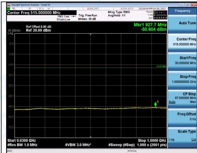
Band2_20MHz_QPSK_19100_1RB#0_30~1000_30~1000
