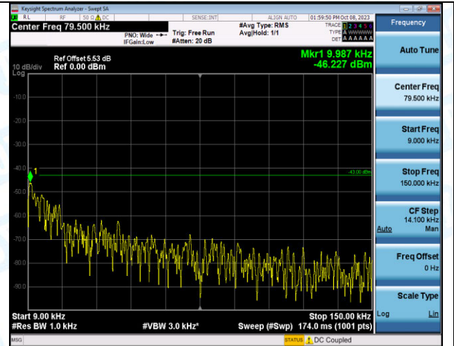
Band2_20MHz_16QAM_18900_1RB#0_0.009~0.15_0.009 ~0.15
