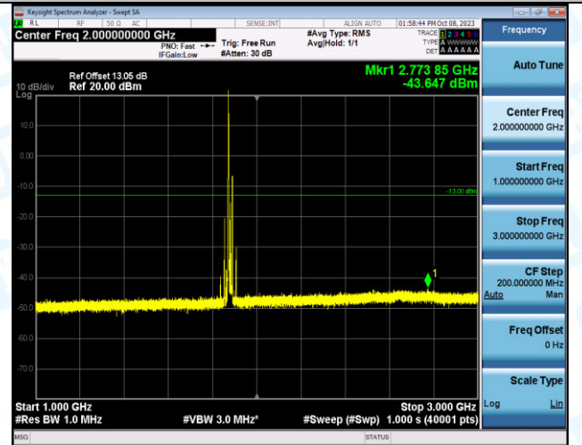
Band2_20MHz_QPSK_18900_1RB#0_1000~3000_1000~3000
