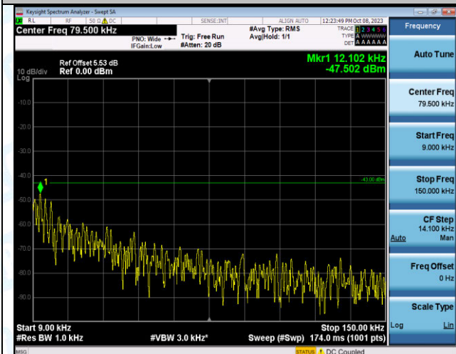
Band2_15MHz_16QAM_19125_1RB#74_0.009~0.15_0.009~0.15
