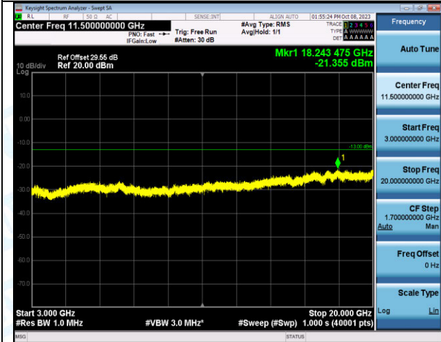
Band2_20MHz_QPSK_18700_1RB#99_3000~20000_3000~20000 0~20000
