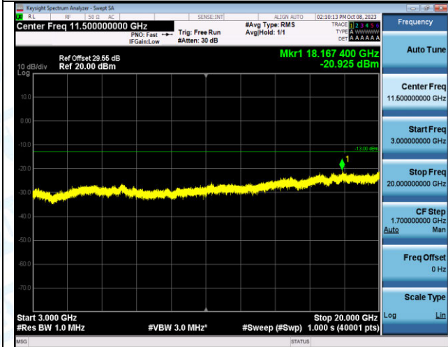
Band2_20MHz_QPSK_19100_1RB#0_3000~20000_3000~20000
