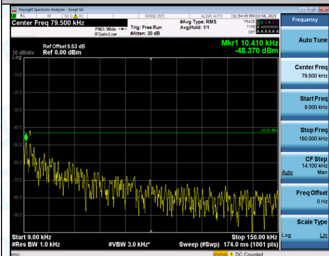
Band2_20MHz_QPSK_18700_1RB#99_0.009~0.15_0.009~0.15
