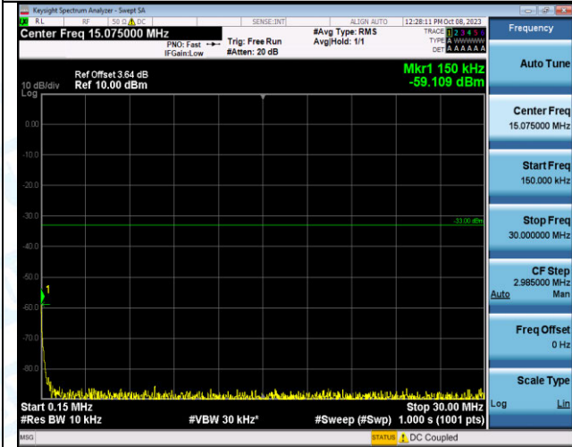
Band2_15MHz_QPSK_19125_75RB#0_0.15~30_0.15~30
