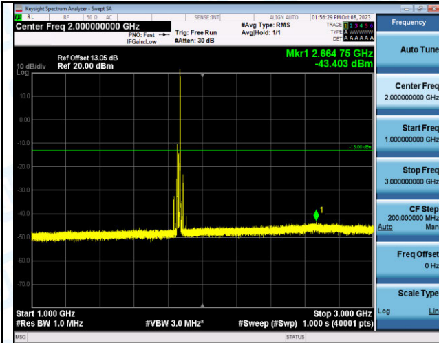
Band2_20MHz_16QAM_18700_1RB#99_1000~3000_100 0~3000
