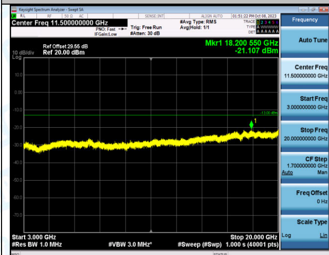
Band2_20MHz_QPSK_18700_1RB#0_3000~20000_3000~20000
