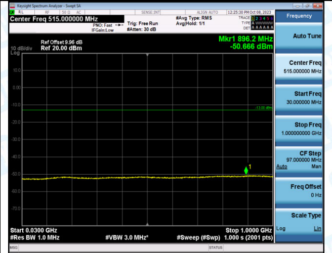
Band2_15MHz_QPSK_18675_75RB#0_30~1000_30~1000
