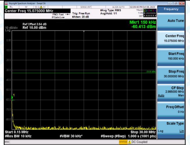
Band2_20MHz_QPSK_19100_1RB#0_0.15~30_0.15~30
