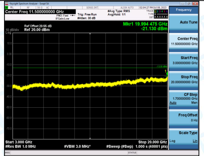
Band2_20MHz_16QAM_18900_1RB#99_3000~20000_30 00~20000
