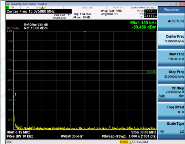
Band2_20MHz_16QAM_18700_1RB#99_0.15~30_0.15~30 0
