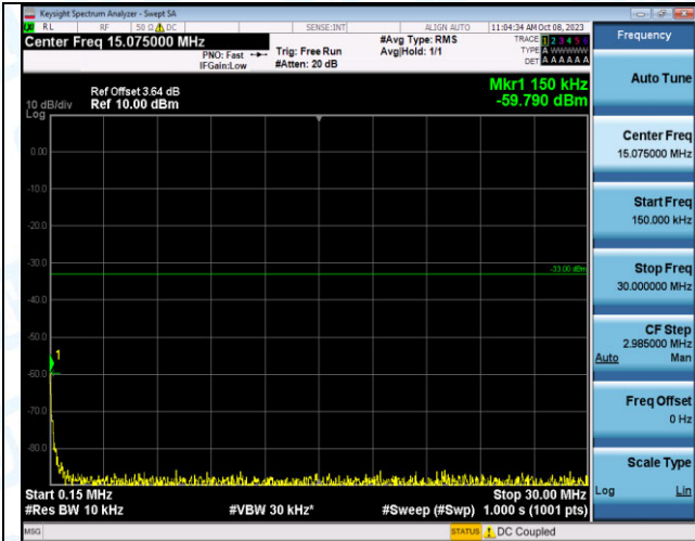
Band2_10MHz_16QAM_18900_1RB#49_0.15~30_0.15~3 0
