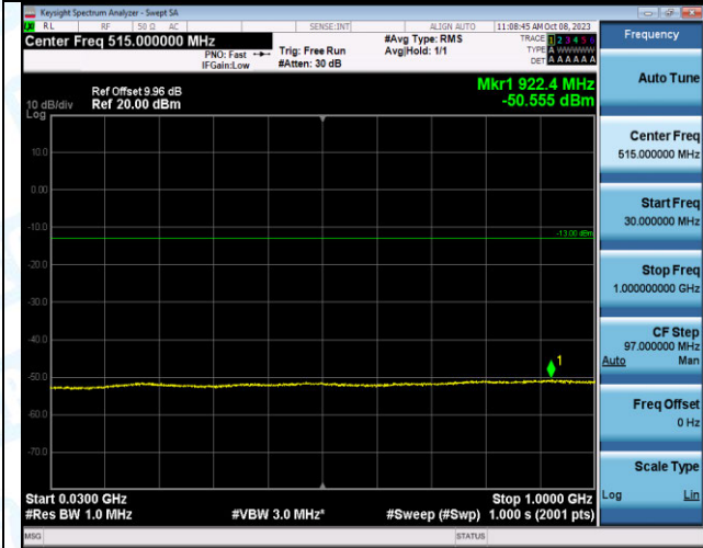
Band2_10MHz_QPSK_19150_1RB#49_30~1000_30~100 0
