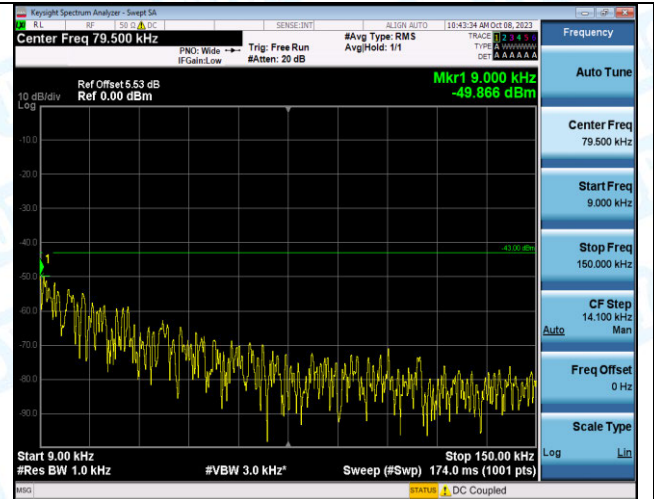
Band2_10MHz_16QAM_18900_1RB#0_0.009~0.15_0.009 ~0.15
