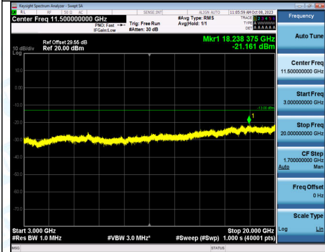
Band2_10MHz_QPSK_19150_1RB#0_3000~20000_3000~20000
