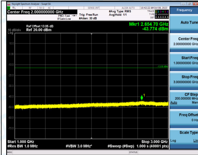
Band2_10MHz_16QAM_18650_1RB#49_1000~3000_100 0~3000
