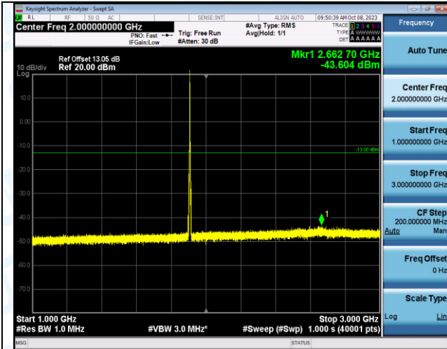
Band2_5MHz_16QAM_19175_1RB#0_1000~3000_1000~3000
