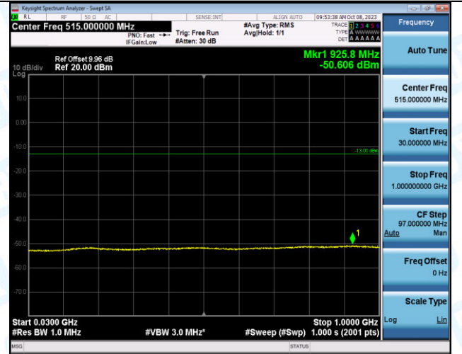
Band2_5MHz_16QAM_19175_25RB#0_30~1000_30~100 0
