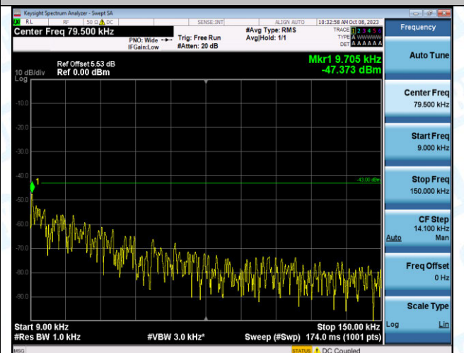
Band2_10MHz_16QAM_18650_1RB#0_0.009~0.15_0.009~0.15
