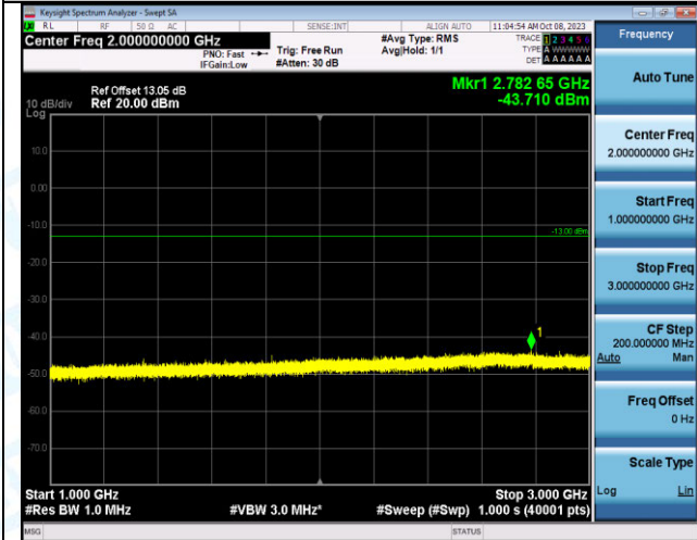
Band2_10MHz_16QAM_18900_1RB#49_1000~3000_100 0~3000
