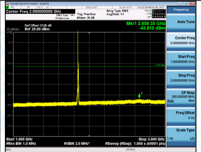
Band2_10MHz_QPSK_18650_1RB#0_1000~3000_1000~3000
