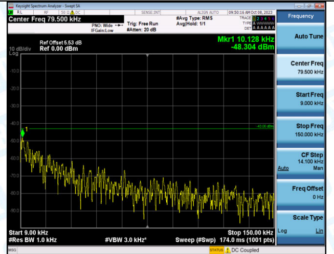
Band2_5MHz_16QAM_19175_1RB#0_0.009~0.15_0.009~0.15
