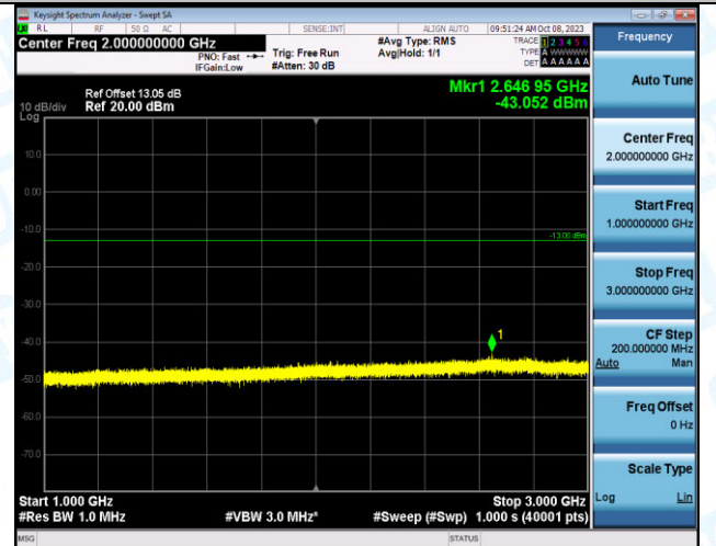
Band2_5MHz_QPSK_19175_25RB#0_1000~3000_1000~3000
