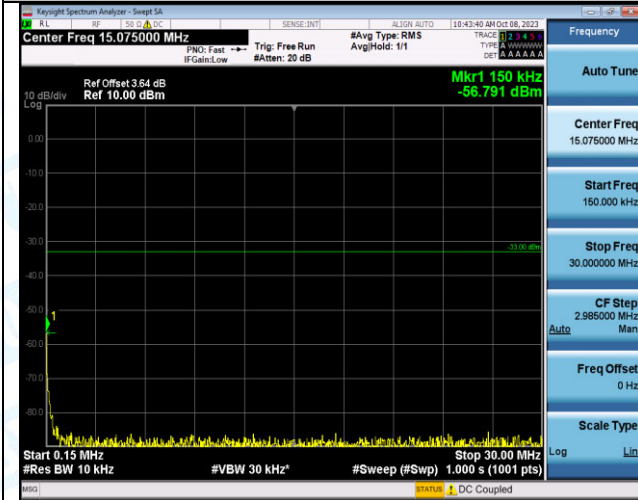
Band2_10MHz_16QAM_18900_1RB#0_0.15~30_0.15~30
