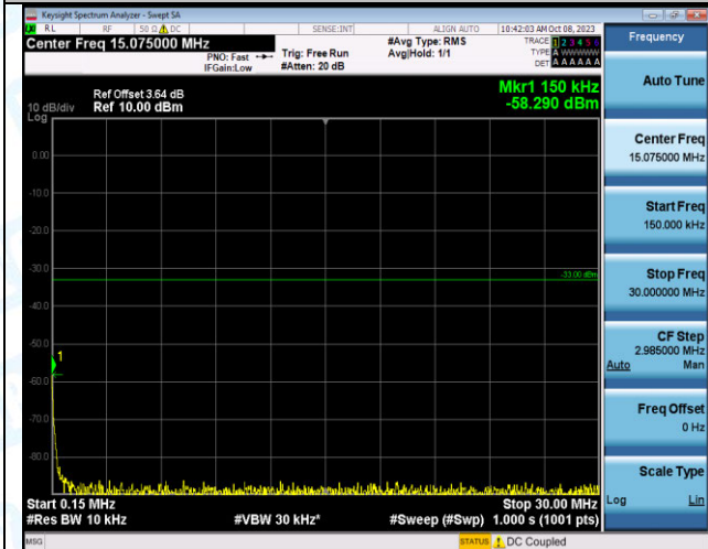
Band2_10MHz_16QAM_18650_1RB#49_0.15~30_0.15~30 0
