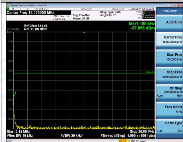
Band2_10MHz_16QAM_19150_1RB#0_0.15~30_0.15~30
