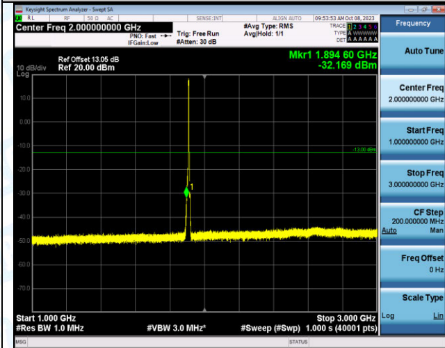
Band2_5MHz_16QAM_19175_25RB#0_1000~3000_1000 ~3000
