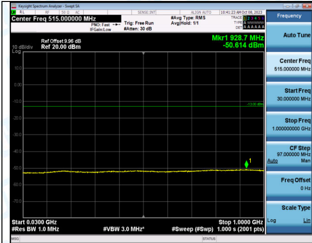
Band2_10MHz_QPSK_18650_1RB#49_30~1000_30~100 0
