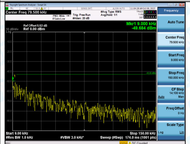
Band2_10MHz_16QAM_18900_1RB#49_0.009~0.15_0.00 9~0.15
