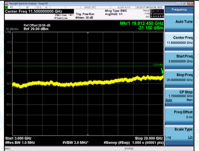
Band2_10MHz_16QAM_18650_1RB#0_3000~20000_3000~20000
