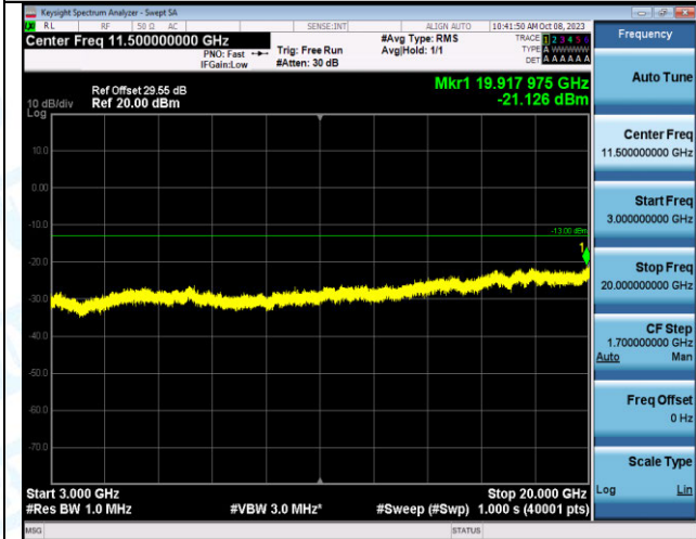
Band2_10MHz_QPSK_18650_1RB#49_3000~20000_3000~20000 0~20000
