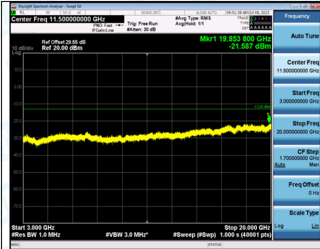
Band2_5MHz_QPSK_19175_25RB#0_3000~20000_3000 ~20000
