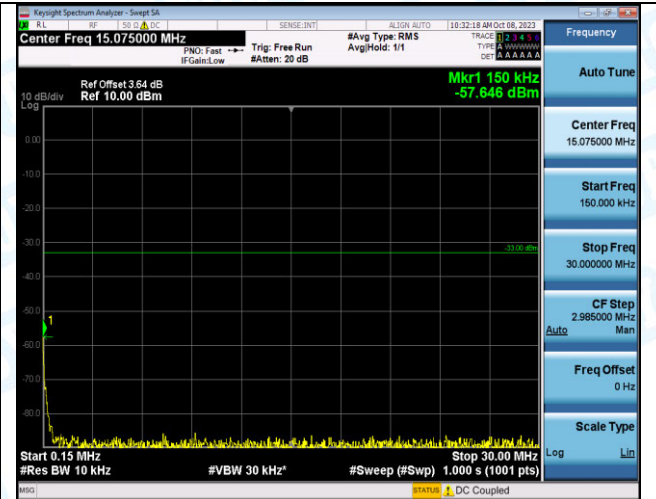
Band2_10MHz_QPSK_18650_1RB#0_0.15~30_0.15~30
