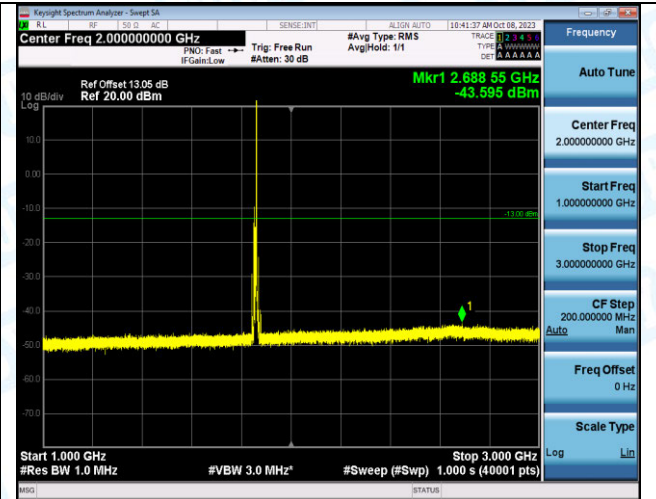
Band2_10MHz_QPSK_18650_1RB#49_1000~3000_1000~3000 ~3000
