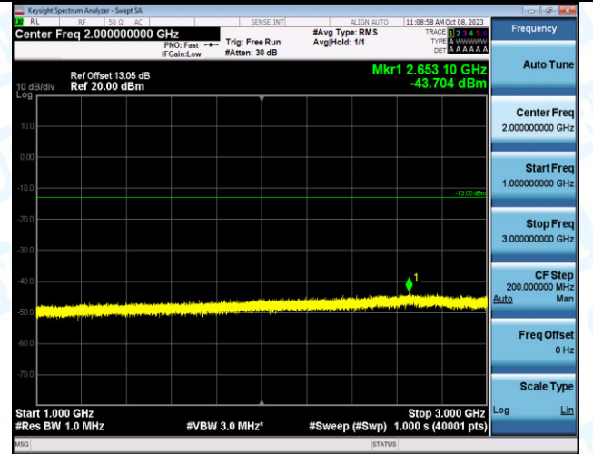
Band2_10MHz_QPSK_19150_1RB#49_1000~3000_1000 ~3000
