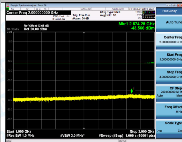
Band2_10MHz_16QAM_18900_1RB#0_1000~3000_1000 ~3000
