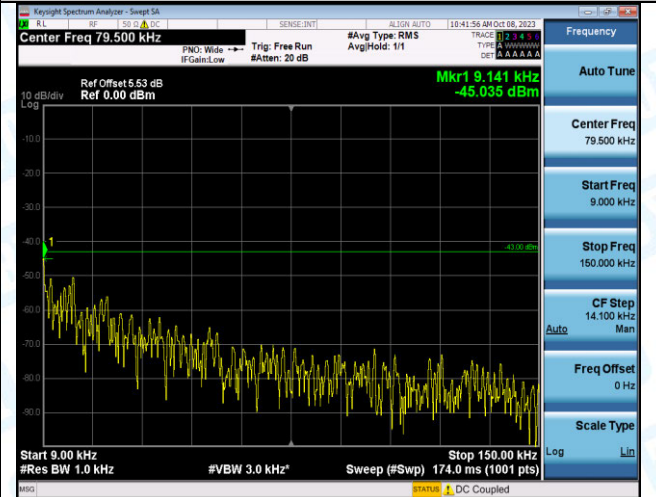
Band2_10MHz_16QAM_18650_1RB#49_0.009~0.15_0.009~0.15 9~0.15
