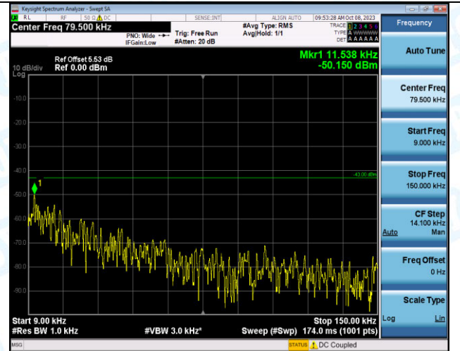
Band2_5MHz_16QAM_19175_25RB#0_0.009~0.15_0.009 ~0.15
