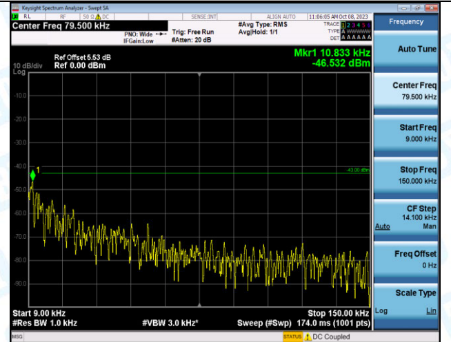
Band2_10MHz_16QAM_19150_1RB#0_0.009~0.15_0.009~0.15
