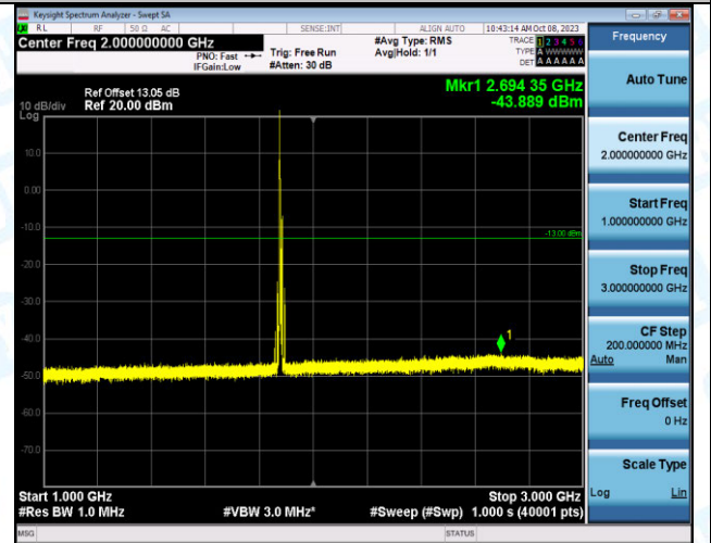
Band2_10MHz_QPSK_18900_1RB#0_1000~3000_1000~3000
