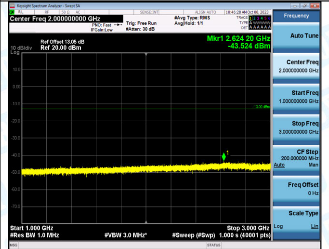
Band2_10MHz_QPSK_18900_1RB#49_1000~3000_1000 ~3000
