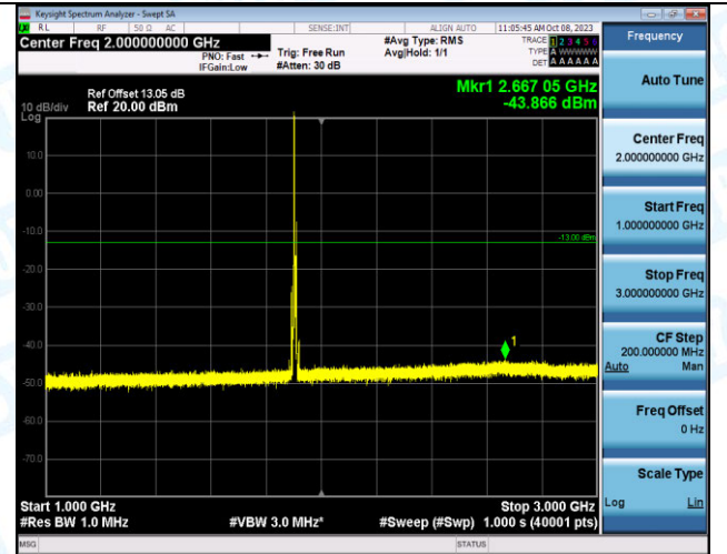
Band2_10MHz_QPSK_19150_1RB#0_1000~3000_1000~3000
