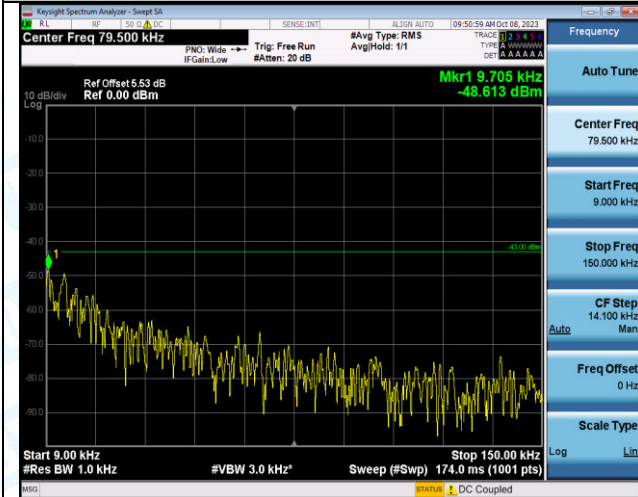
Band2_5MHz_QPSK_19175_25RB#0_0.009~0.15_0.009~0.15
