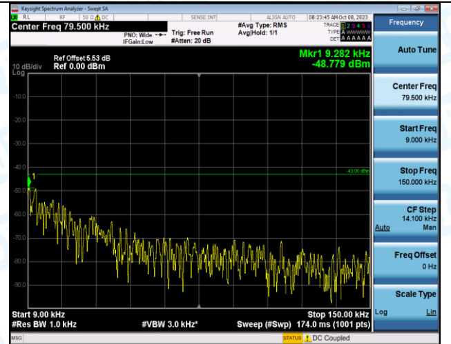
Band2_1.4MHz_16QAM_18900_1RB#0_0.009~0.15_0.00 9~0.15
