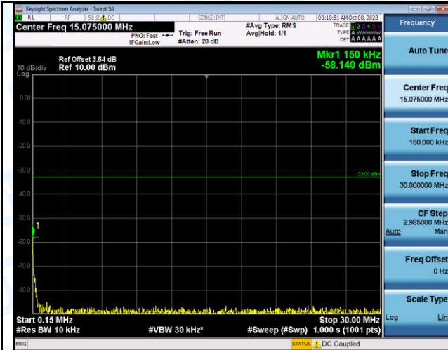
Band2_3MHz_16QAM_18615_1RB#0_0.15~30_0.15~30
