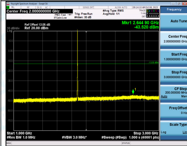
Band2_3MHz_16QAM_18900_1RB#0_1000~3000_1000~3000
