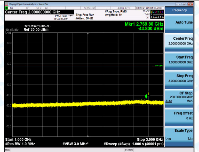
Band2_1.4MHz_QPSK_18900_1RB#0_1000~3000_1000~3000
