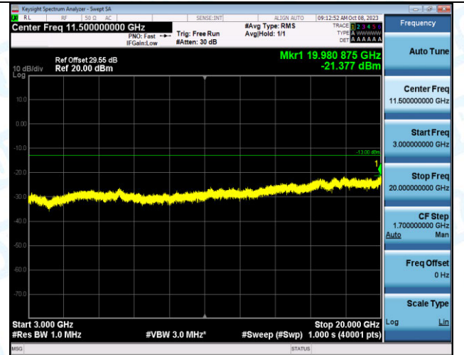
Band2_3MHz_16QAM_18615_15RB#0_3000~20000_300 0~20000
