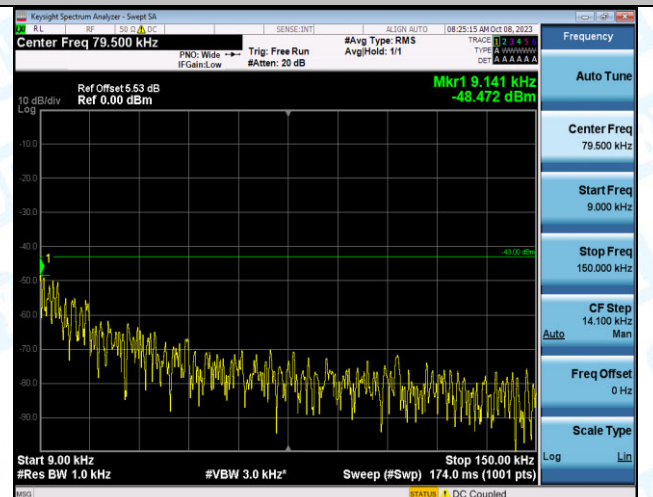
Band2_1.4MHz_16QAM_18900_6RB#0_0.009~0.15_0.00~9~0.15
