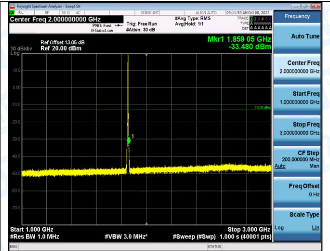
Band2_3MHz_QPSK_18615_15RB#0_1000~3000_1000~3000
