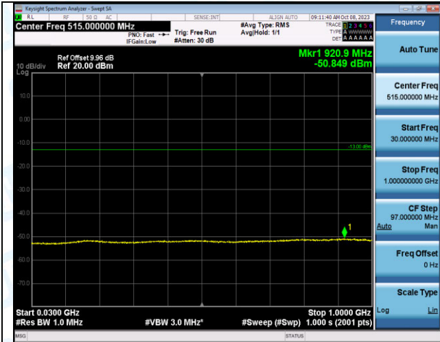
Band2_3MHz_QPSK_18615_15RB#0_30~1000_30~1000
