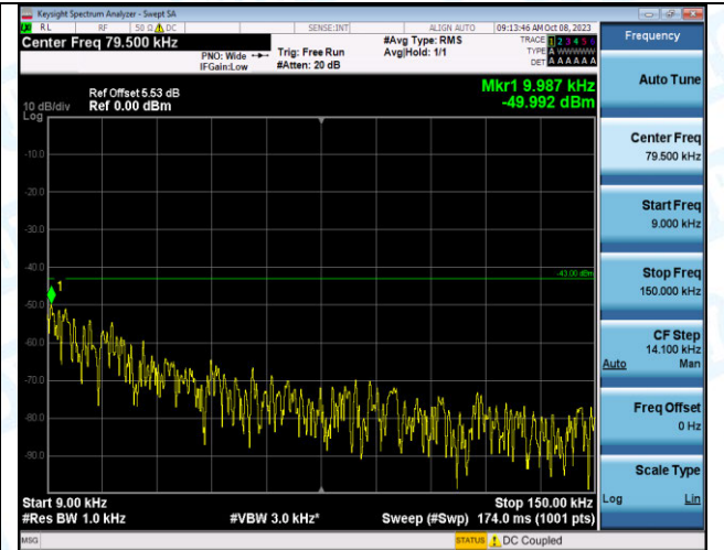
Band2_3MHz_16QAM_18900_1RB#0_0.009~0.15_0.009~0.15
