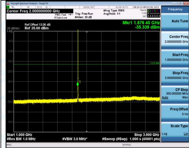
Band2_1.4MHz_16QAM_18900_1RB#0_1000~3000_1000 ~3000
