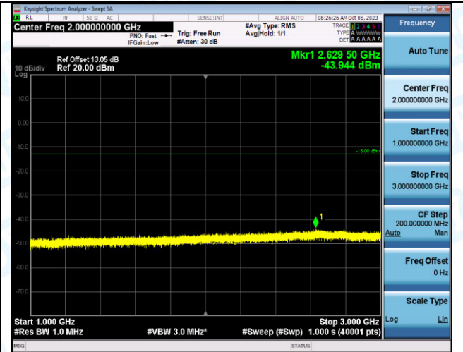
Band2_1.4MHz_QPSK_19193_1RB#0_1000~3000_1000~3000
