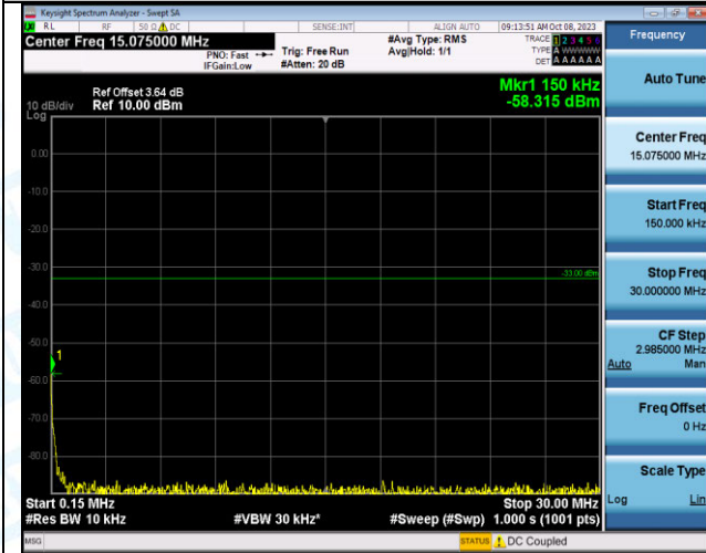
Band2_3MHz_16QAM_18900_1RB#0_0.15~30_0.15~30
