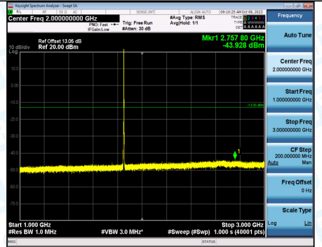
Band2_3MHz_QPSK_18615_1RB#0_1000~3000_1000~3000
