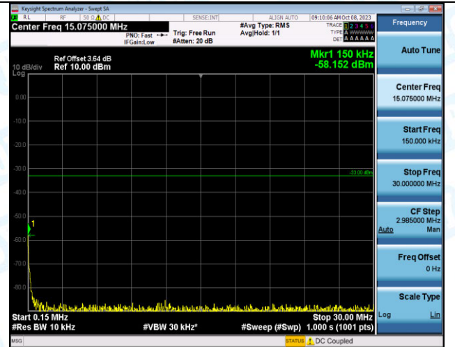
Band2_3MHz_QPSK_18615_1RB#0_0.15~30_0.15~30
