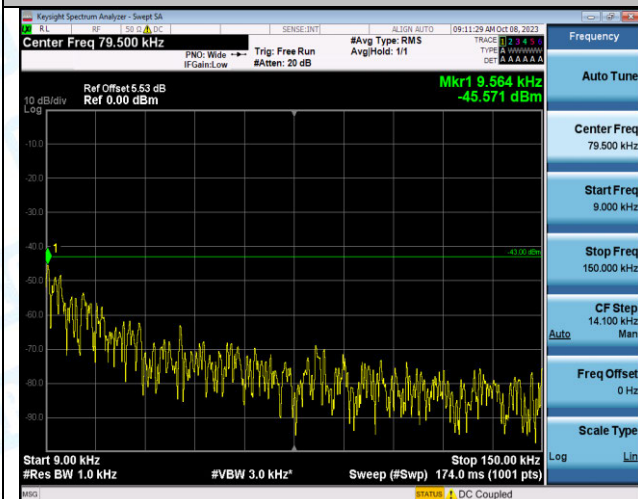
Band2_3MHz_QPSK_18615_15RB#0_0.009~0.15_0.009~0.15
