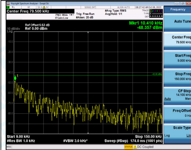
Band2_1.4MHz_QPSK_19193_6RB#0_0.009~0.15_0.009 ~0.15
