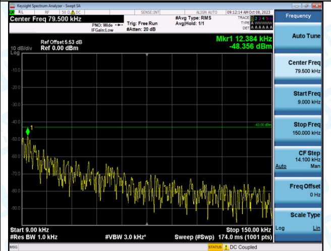
Band2_3MHz_16QAM_18615_15RB#0_0.009~0.15_0.009~0.15
