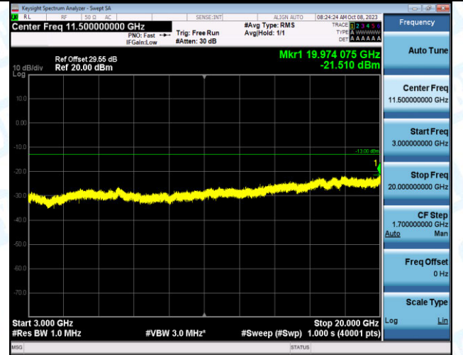
Band2_1.4MHz_16QAM_18900_1RB#0_3000~20000_300 0~20000
