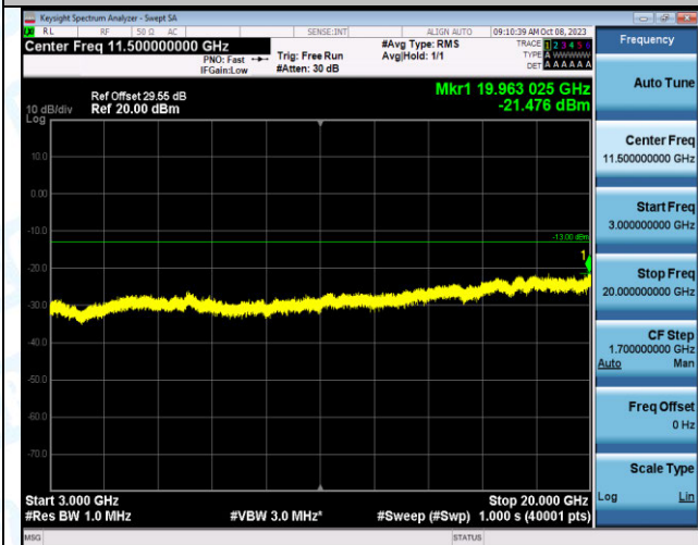
Band2_3MHz_QPSK_18615_1RB#0_3000~20000_3000~20000
