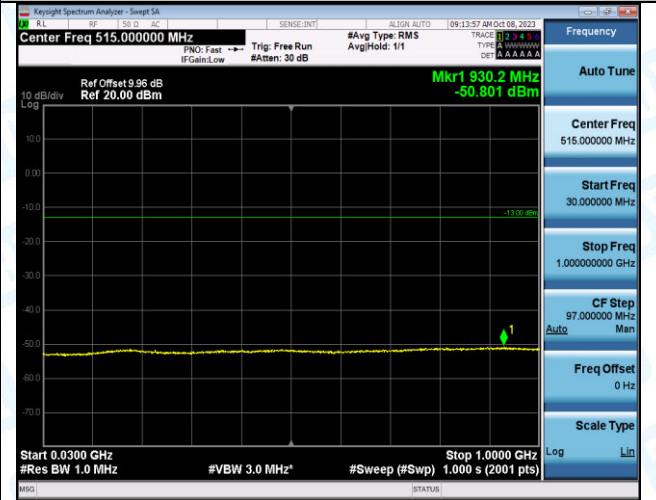
Band2_3MHz_16QAM_18900_1RB#0_30~1000_30~1000
