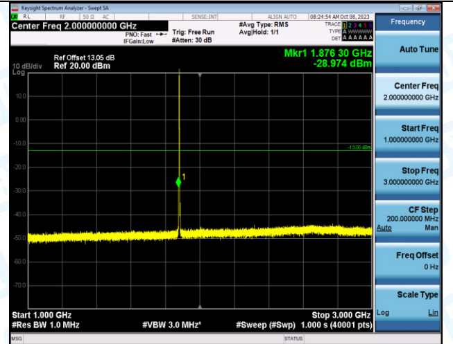
Band2_1.4MHz_QPSK_18900_6RB#0_1000~3000_1000~3000
