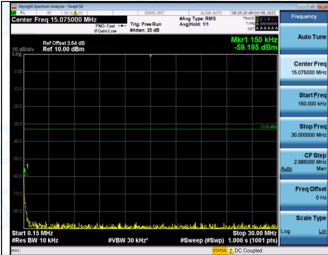
Band2_1.4MHz_16QAM_18900_6RB#0_0.15~30_0.15~3 0
