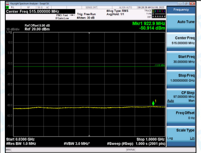
Band2_1.4MHz_16QAM_19193_6RB#0_30~1000_30~10 00
