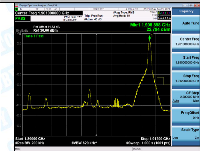
Band2_20MHz_16QAM_19100_1RB#99
