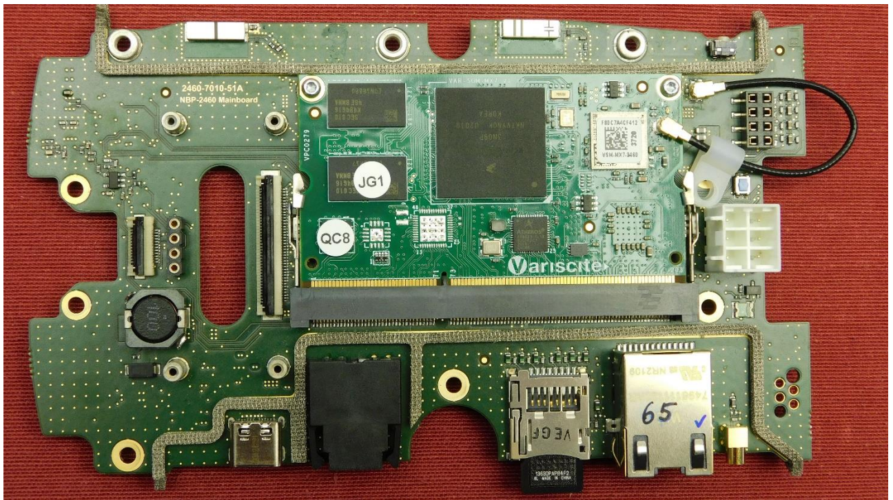
Picture 5: EUT module with RF module – front view
