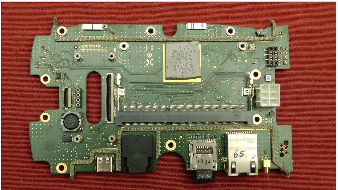
Picture 7: EUT module without RF module – front view
