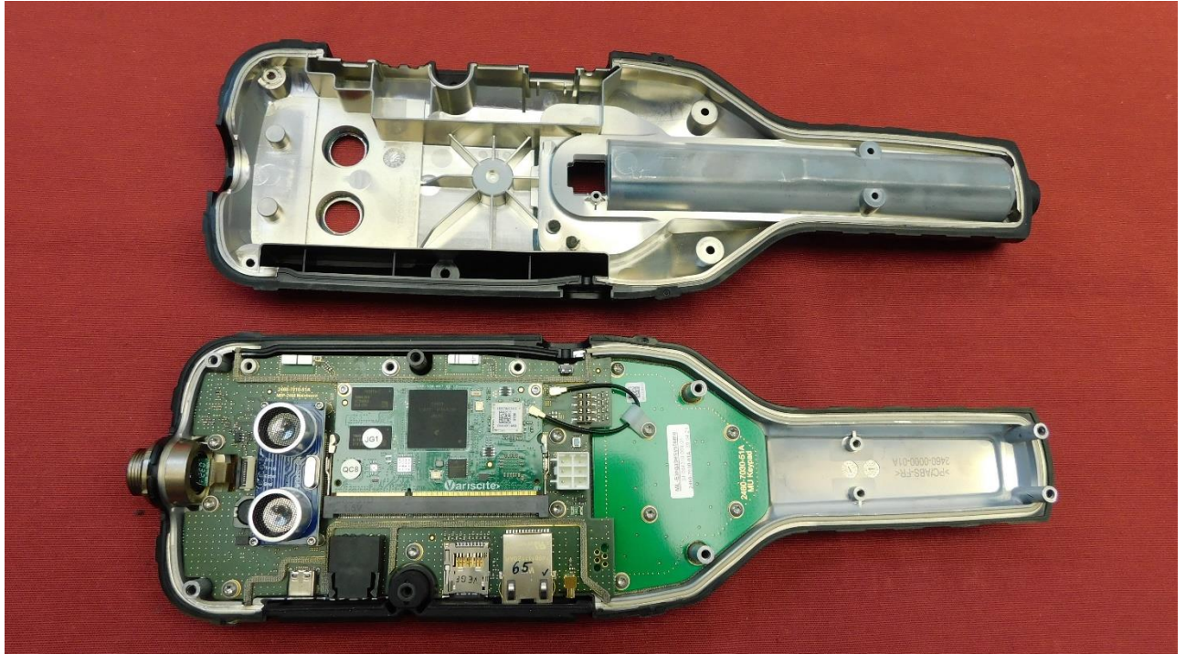
Picture 2: EUT – rear view, without housing
