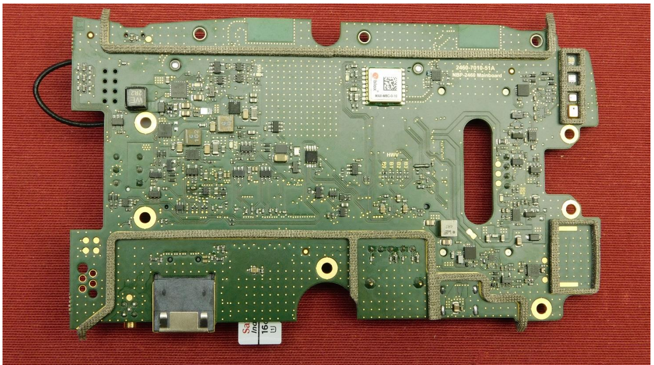
Picture 6: EUT module with RF module – rear view
