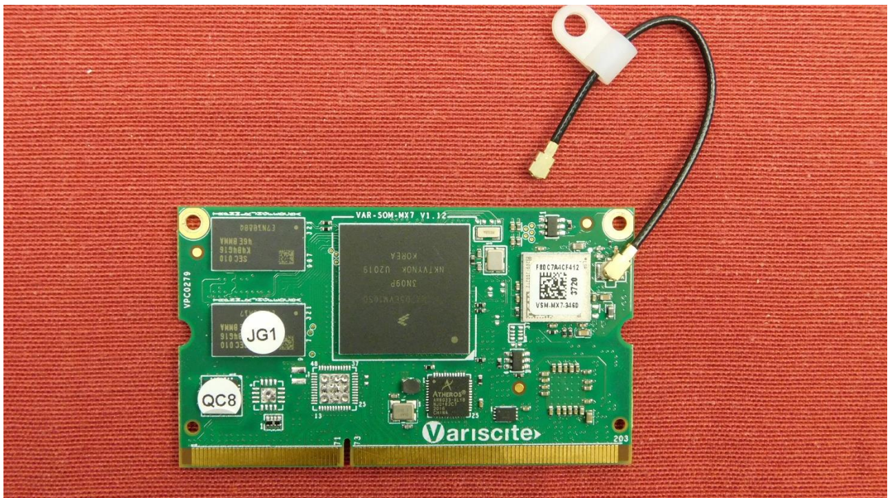
Picture 8: RF module – front view
