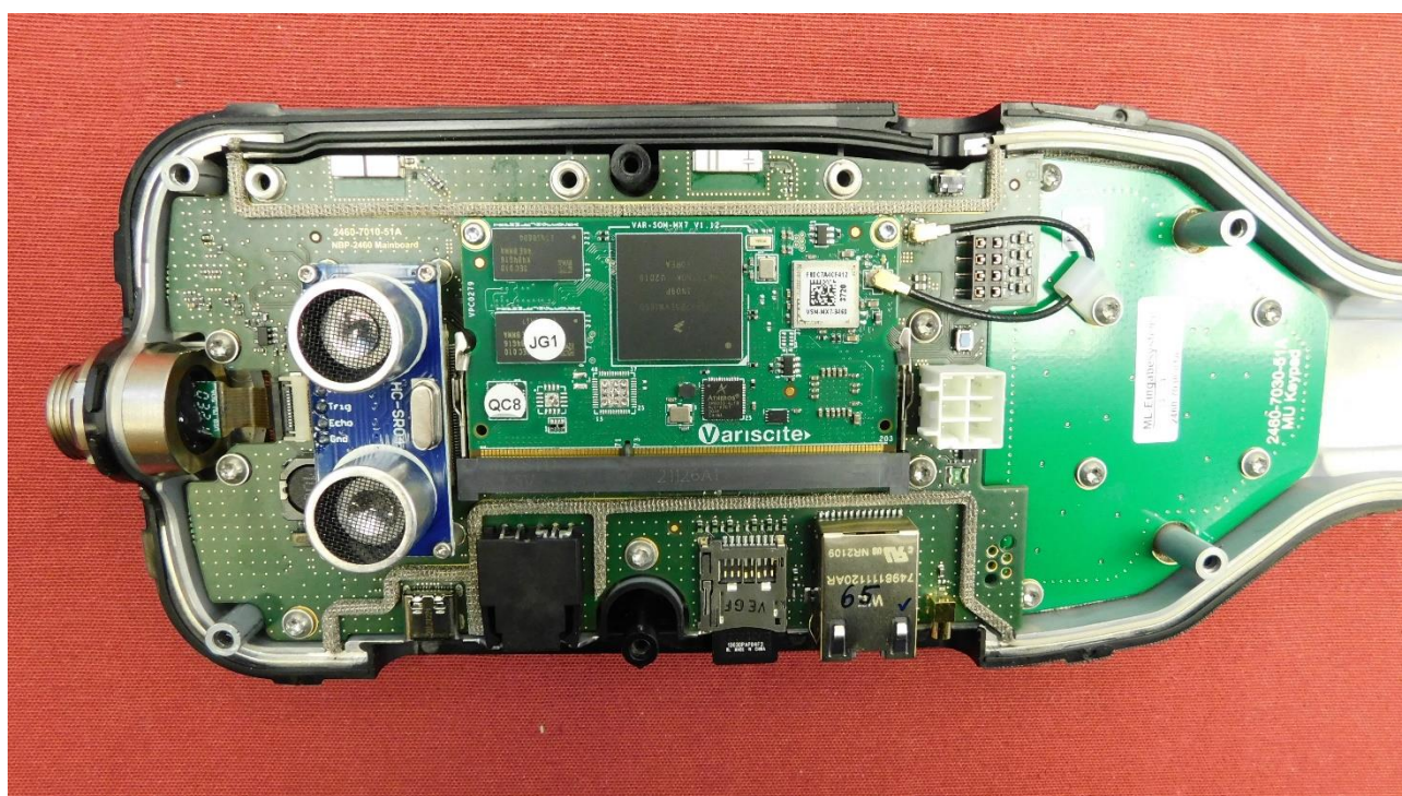
Picture 4: EUT – front view
