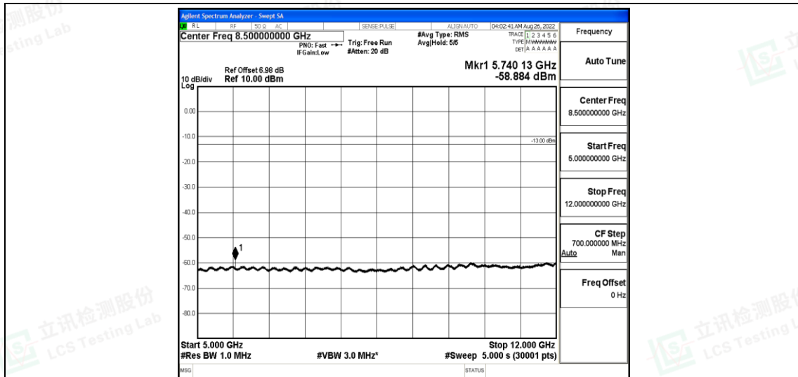
Band12-10MHz-16QAM-23130-1-0-High-5000-12000--58.88-PASS
