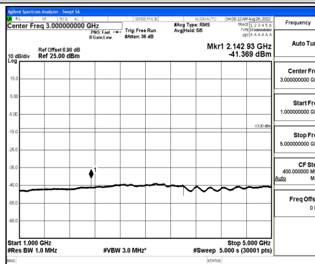
Band12-10MHz-QPSK-23130-1-0-High-1000-5000--41.37-PASS
