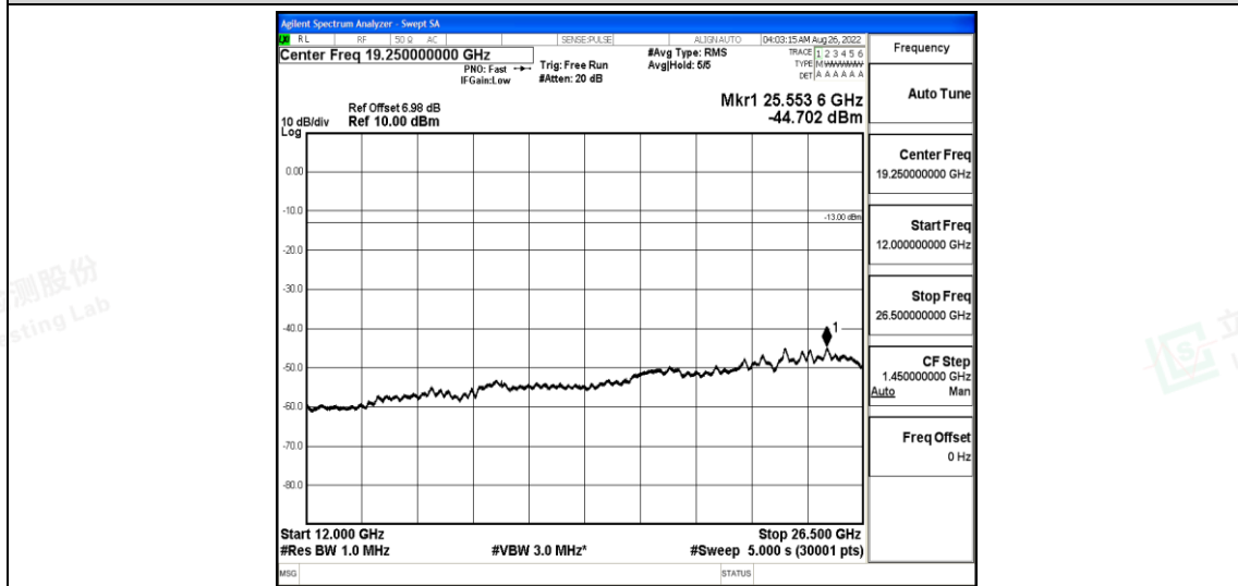
Band12-10MHz-16QAM-23130-1-0-High-12000-26500--44.7-PASS
