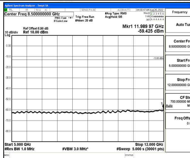
Band12-10MHz-QPSK-23130-1-0-High-5000-12000--59.43-PASS
