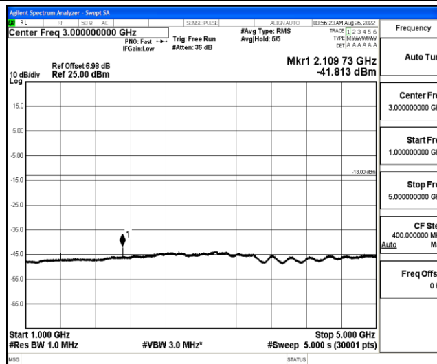
Band12-10MHz-QPSK-23095-1-0-Low-1000-5000--41.81-PASS
