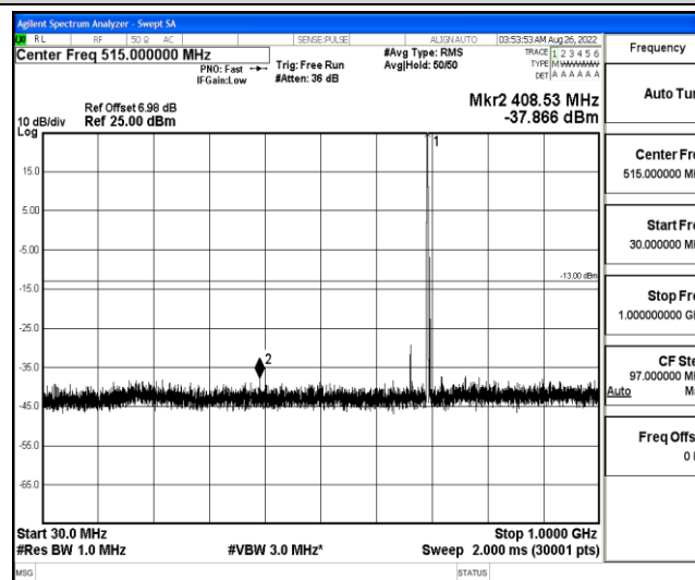
Band12-10MHz-16QAM-23060-1-0-Low-30-1000--37.87-PASS
