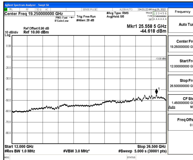
Band12-10MHz-QPSK-23130-1-0-High-12000-26500--44.62-PASS
