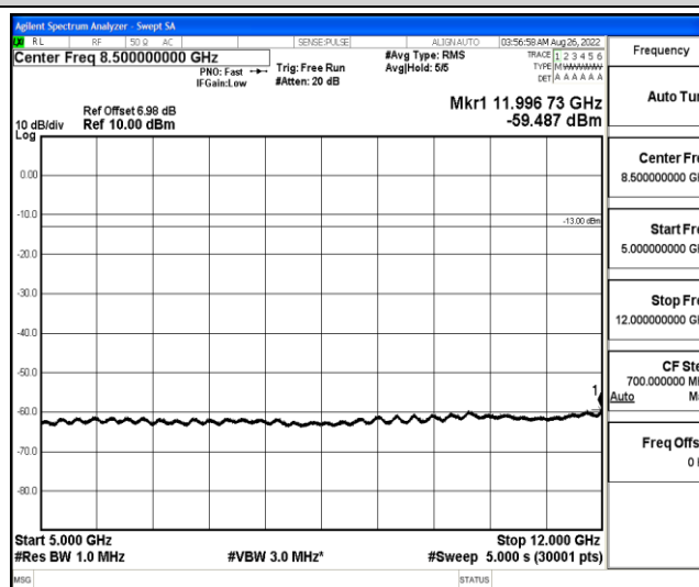
Band12-10MHz-QPSK-23095-1-0-Low-5000-12000--59.49-PASS
