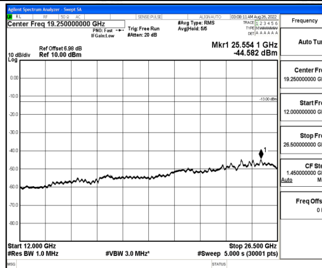
Band12-3MHz-16QAM-23095-1-0-Low-12000-26500--44.58-PASS
