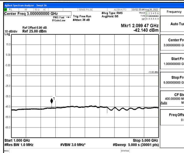
Band12-10MHz-QPSK-23060-1-0-Low-1000-5000--42.14-PASS
