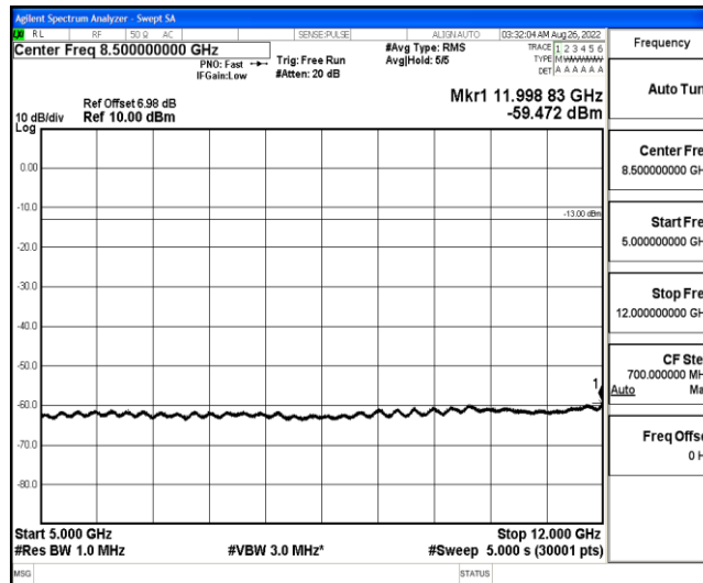
Band12-5MHz-QPSK-23035-1-0-Low-5000-12000--59.47-PASS
