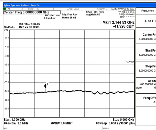
Band12-1.4MHz-QPSK-23173-1-0-High-1000-5000--41.93-PASS
