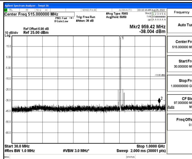
Band12-3MHz-16QAM-23165-1-0-High-30-1000--38-PASS
