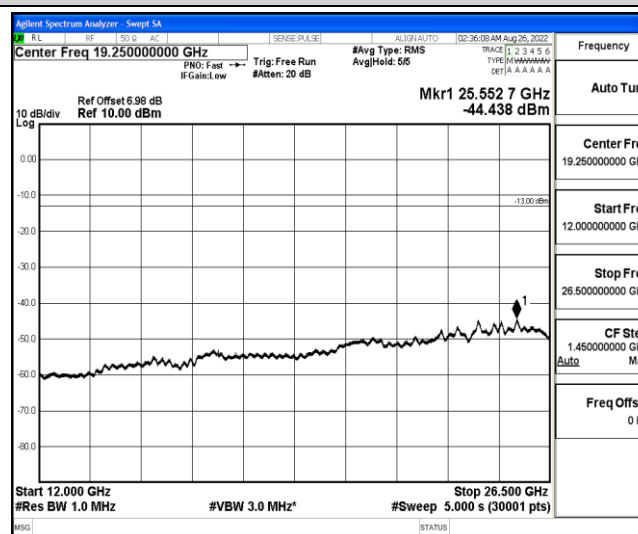
Band12-1.4MHz-QPSK-23017-1-0-Low-12000-26500--44.44-PASS
