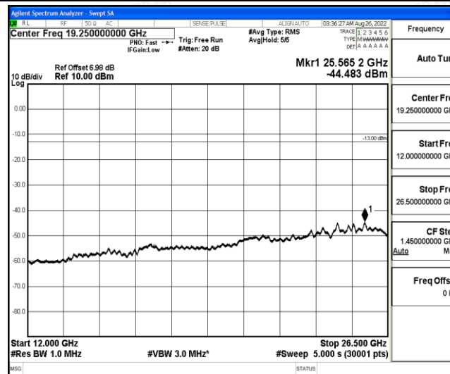
Band12-5MHz-QPSK-23095-1-0-Low-12000-26500--44.48-PASS
