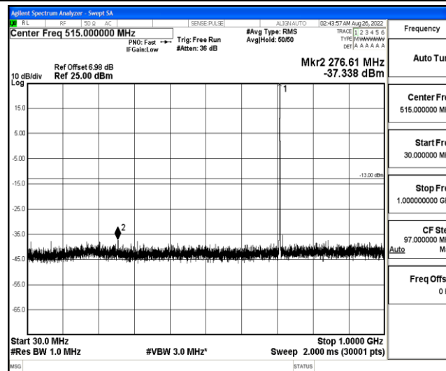
Band12-1.4MHz-16QAM-23173-1-0-High-30-1000--37.34-PASS
