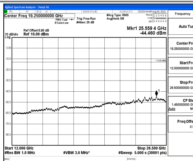
Band12-10MHz-QPSK-23060-1-0-Low-12000-26500--44.46-PASS
