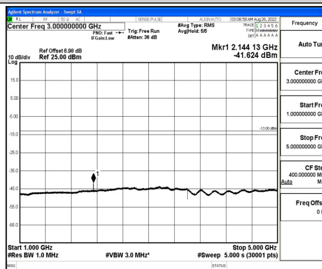
Band12-3MHz-QPSK-23165-1-0-High-1000-5000--41.62-PASS
