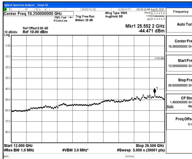
Band12-5MHz-QPSK-23155-1-0-High-12000-26500--44.47-PASS
