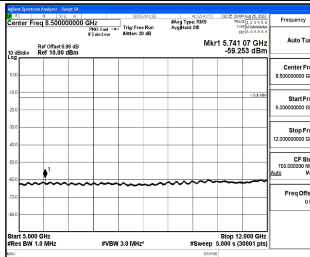
Band12-1.4MHz-QPSK-23017-1-0-Low-5000-12000--59.25-PASS
