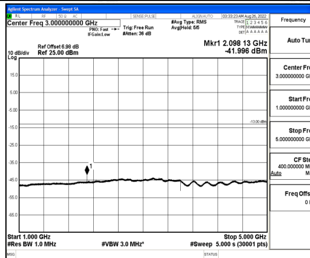
Band12-5MHz-16QAM-23035-1-0-Low-1000-5000--42-PASS
