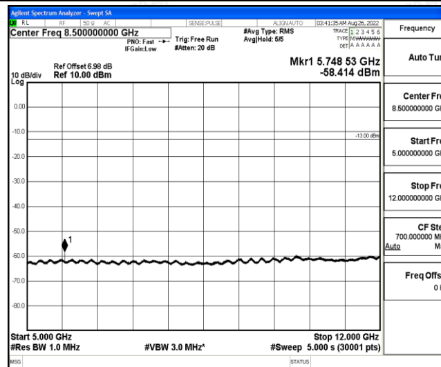
Band12-5MHz-16QAM-23155-1-0-High-5000-12000--58.41-PASS
