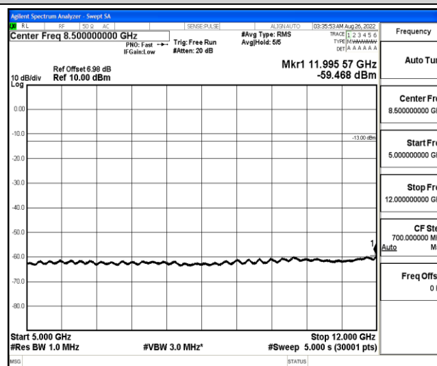
Band12-5MHz-QPSK-23095-1-0-Low-5000-12000--59.47-PASS
