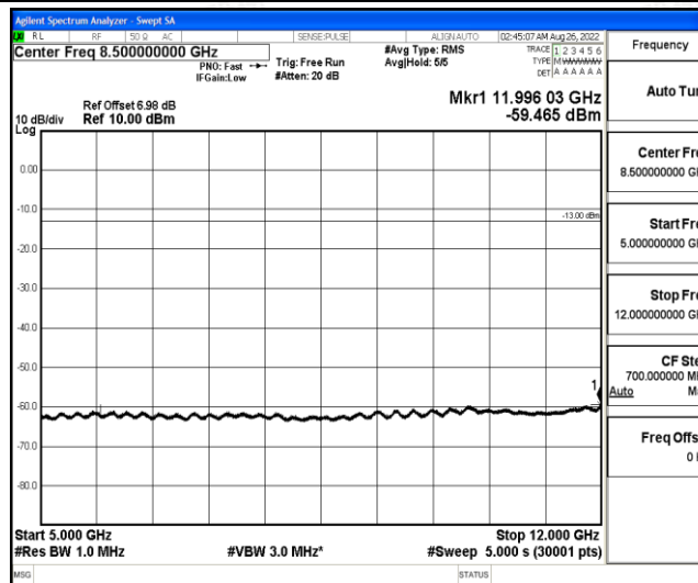
Band12-1.4MHz-16QAM-23173-1-0-High-5000-12000--59.47-PASS
