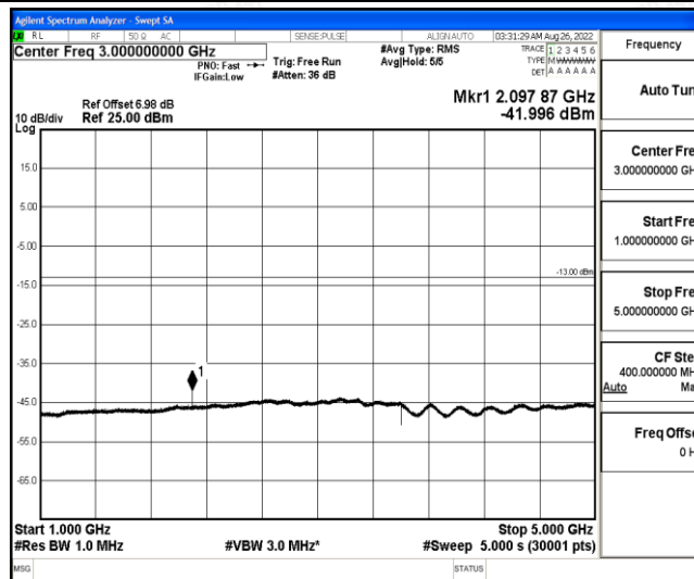
Band12-5MHz-QPSK-23035-1-0-Low-1000-5000--42-PASS
