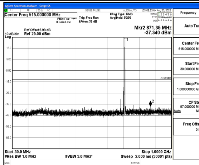
Band12-3MHz-QPSK-23165-1-0-High-30-1000--37.34-PASS
