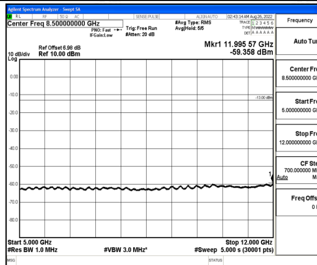
Band12-1.4MHz-QPSK-23173-1-0-High-5000-12000--59.36-PASS
