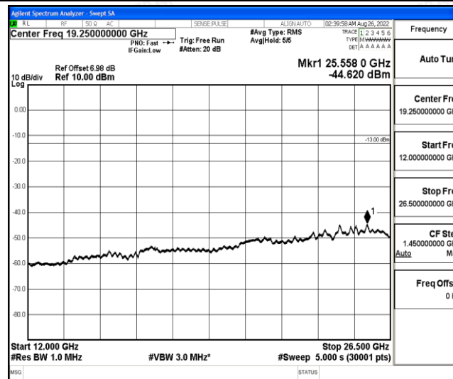
Band12-1.4MHz-QPSK-23095-1-0-Low-12000-26500--44.62-PASS
