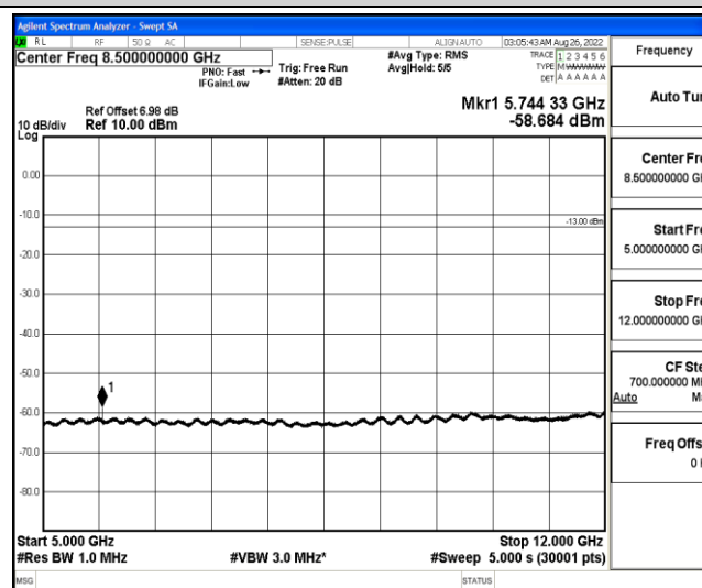
Band12-3MHz-QPSK-23095-1-0-Low-5000-12000--58.68-PASS
