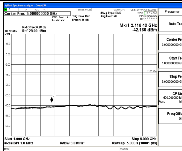
Band12-5MHz-QPSK-23095-1-0-Low-1000-5000--42.17-PASS
