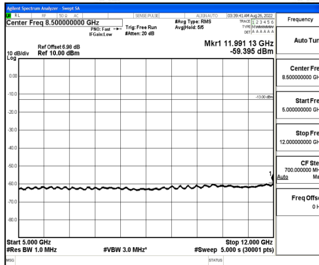
Band12-5MHz-QPSK-23155-1-0-High-5000-12000--59.4-PASS
