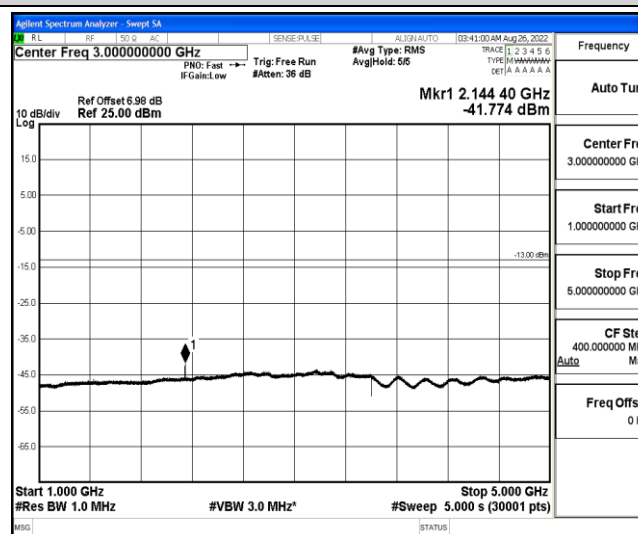
Band12-5MHz-16QAM-23155-1-0-High-1000-5000--41.77-PASS
