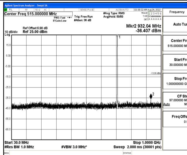
Band12-5MHz-QPSK-23155-1-0-High-30-1000--36.41-PASS
