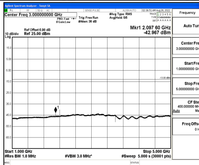
Band12-1.4MHz-16QAM-23017-1-0-Low-1000-5000--42.97-PASS
