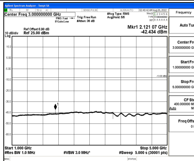
Band12-1.4MHz-16QAM-23095-1-0-Low-1000-5000--42.43-PASS
