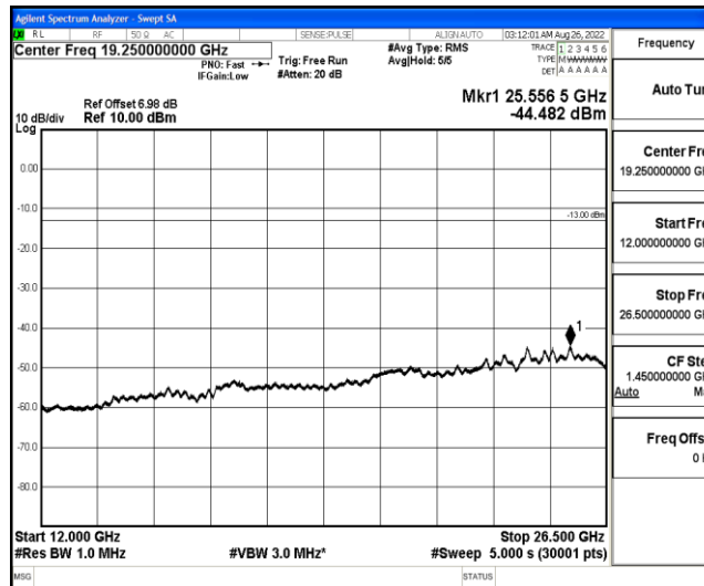
Band12-3MHz-16QAM-23165-1-0-High-12000-26500--44.48-PASS
