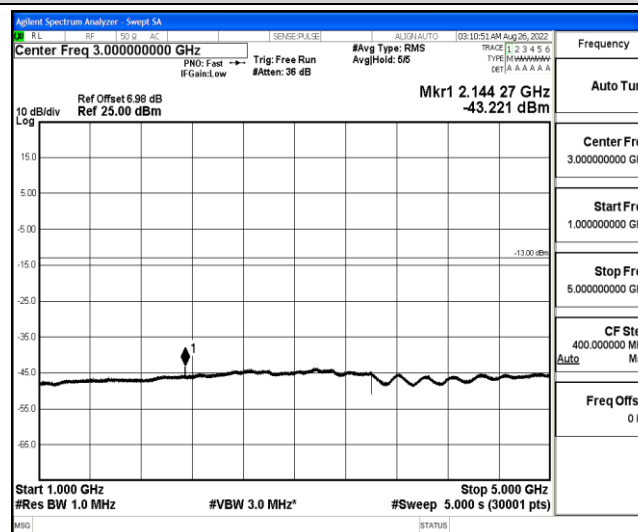
Band12-3MHz-16QAM-23165-1-0-High-1000-5000--43.22-PASS
