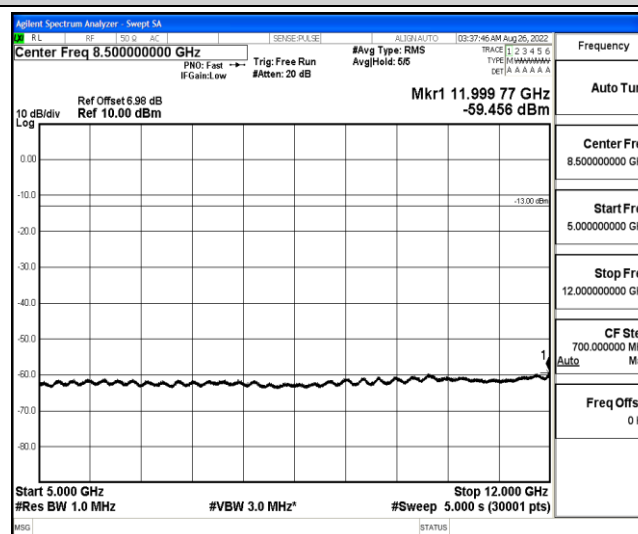
Band12-5MHz-16QAM-23095-1-0-Low-5000-12000--59.46-PASS
