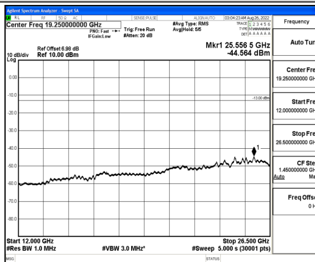
Band12-3MHz-16QAM-23025-1-0-Low-12000-26500--44.56-PASS
