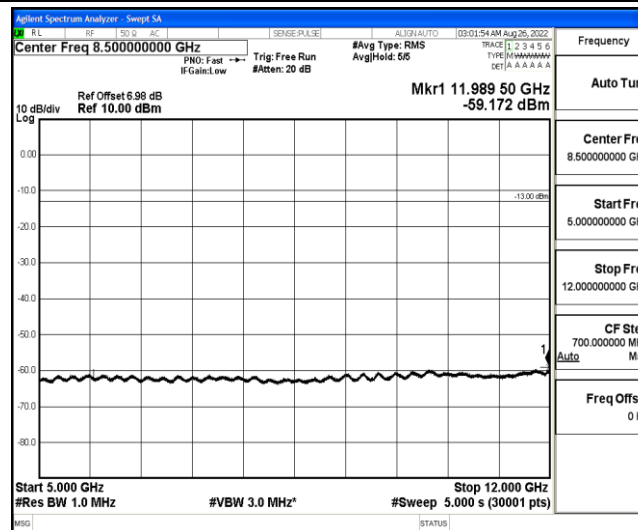
Band12-3MHz-QPSK-23025-1-0-Low-5000-12000--59.17-PASS
