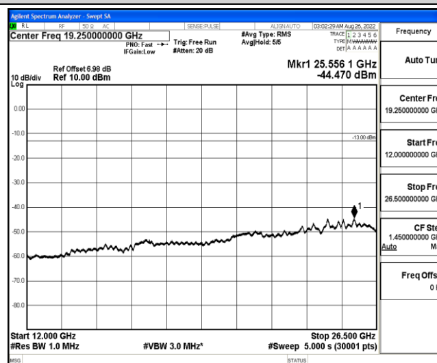
Band12-3MHz-QPSK-23025-1-0-Low-12000-26500--44.47-PASS
