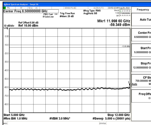
Band12-10MHz-QPSK-23060-1-0-Low-5000-12000--59.35-PASS
