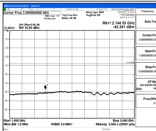
Band12-1.4MHz-16QAM-23173-1-0-High-1000-5000--42.24-PASS
