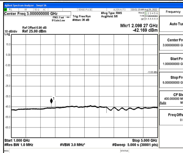
Band12-3MHz-QPSK-23025-1-0-Low-1000-5000--42.17-PASS
