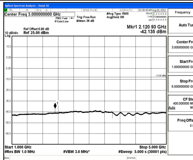
Band12-1.4MHz-QPSK-23095-1-0-Low-1000-5000--42.14-PASS
