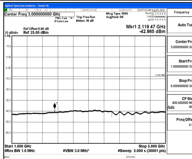
Band12-3MHz-16QAM-23095-1-0-Low-1000-5000--42.87-PASS
