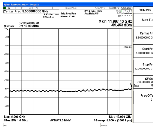
Band12-5MHz-16QAM-23035-1-0-Low-5000-12000--59.45-PASS
