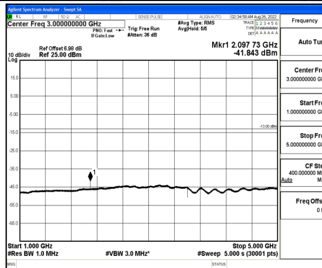
Band12-1.4MHz-QPSK-23017-1-0-Low-1000-5000--41.84-PASS
