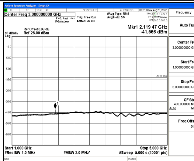
Band12-3MHz-QPSK-23095-1-0-Low-1000-5000--41.57-PASS
