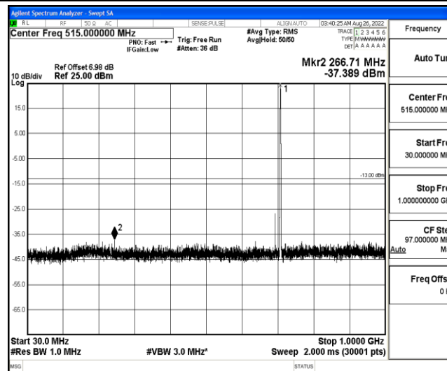
Band12-5MHz-16QAM-23155-1-0-High-30-1000--37.39-PASS
