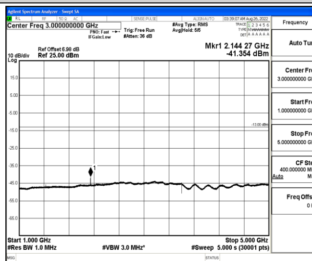
Band12-5MHz-QPSK-23155-1-0-High-1000-5000--41.35-PASS
