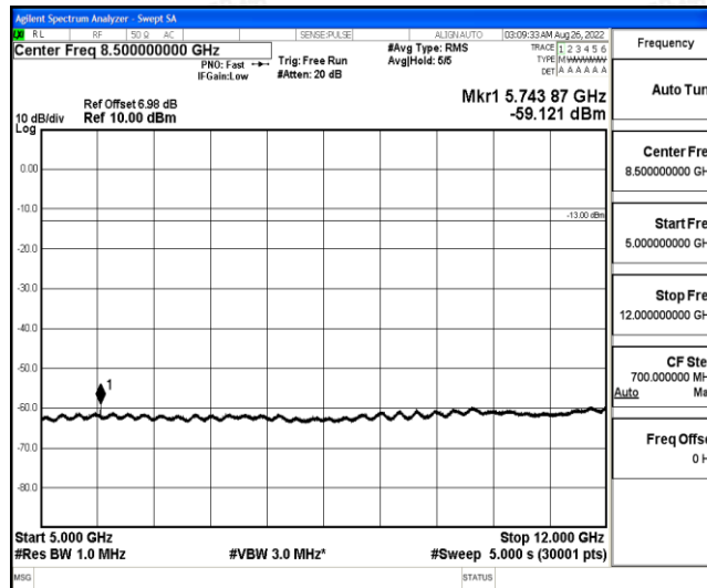
Band12-3MHz-QPSK-23165-1-0-High-5000-12000--59.12-PASS
