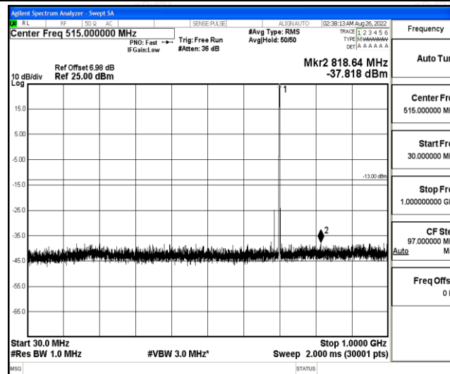
Band12-1.4MHz-QPSK-23095-1-0-Low-30-1000--37.82-PASS
