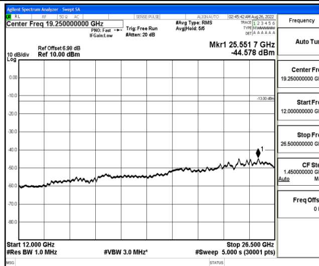
Band12-1.4MHz-16QAM-23173-1-0-High-12000-26500--44.58-PASS
