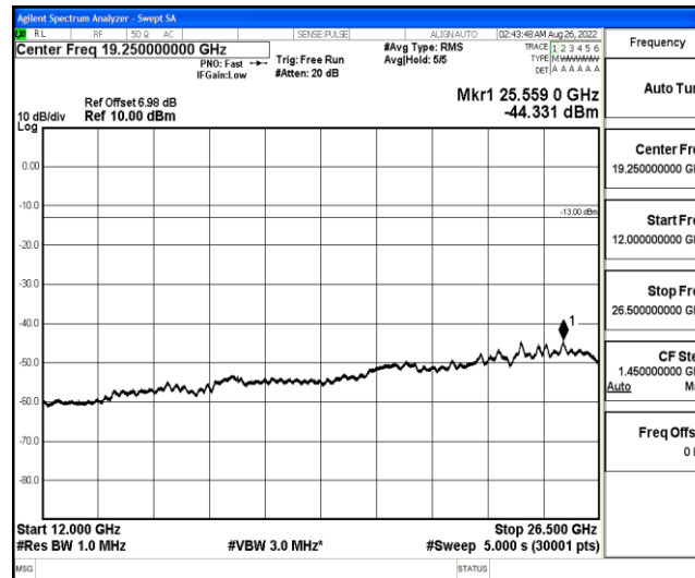
Band12-1.4MHz-QPSK-23173-1-0-High-12000-26500--44.33-PASS
