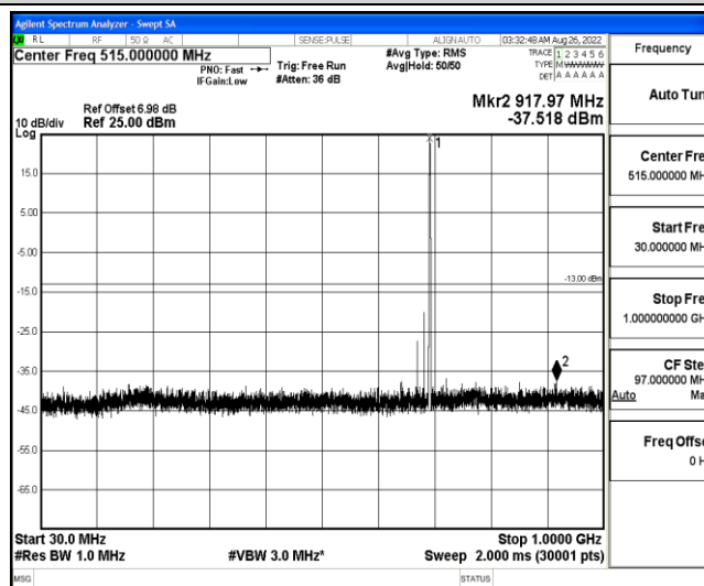
Band12-5MHz-16QAM-23035-1-0-Low-30-1000--37.52-PASS
