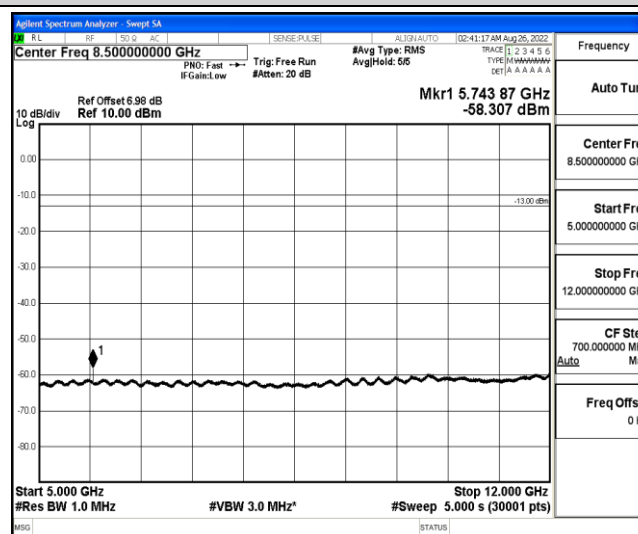
Band12-1.4MHz-16QAM-23095-1-0-Low-5000-12000--58.31-PASS
