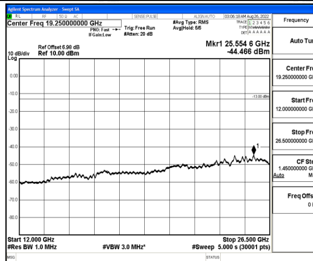
Band12-3MHz-QPSK-23095-1-0-Low-12000-26500--44.47-PASS
