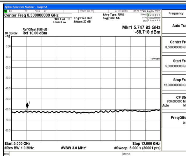
Band12-3MHz-16QAM-23095-1-0-Low-5000-12000--58.72-PASS
