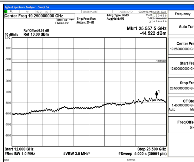
Band12-1.4MHz-16QAM-23017-1-0-Low-12000-26500--44.52-PASS
