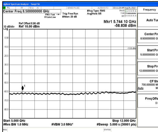
Band12-3MHz-16QAM-23165-1-0-High-5000-12000--58.84-PASS
