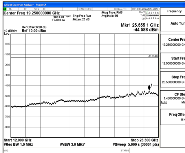
Band12-3MHz-QPSK-23165-1-0-High-12000-26500--44.59-PASS
