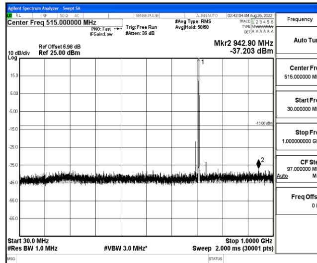
Band12-1.4MHz-QPSK-23173-1-0-High-30-1000--37.2-PASS
