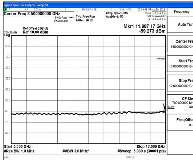
Band12-3MHz-16QAM-23025-1-0-Low-5000-12000--59.27-PASS
