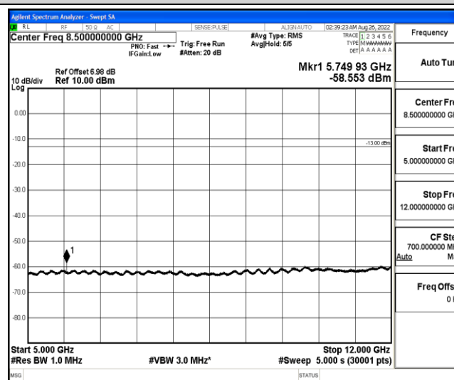
Band12-1.4MHz-QPSK-23095-1-0-Low-5000-12000--58.55-PASS
