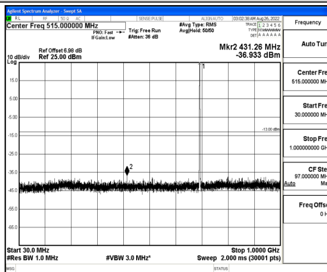
Band12-3MHz-16QAM-23025-1-0-Low-30-1000--36.93-PASS
