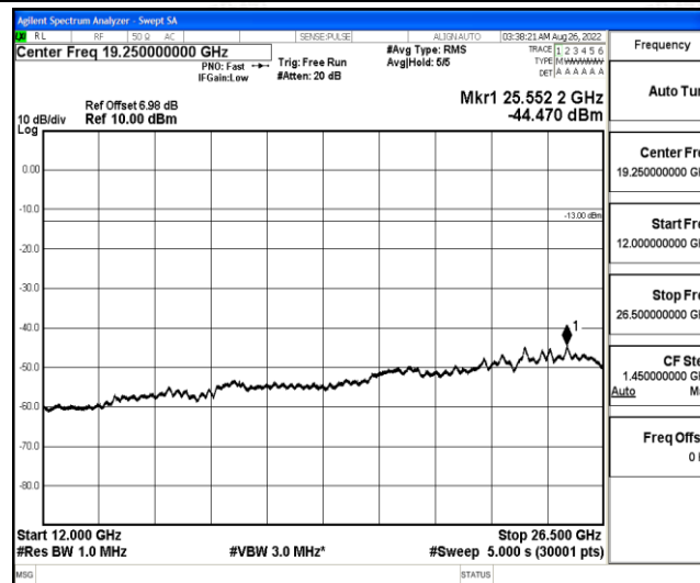
Band12-5MHz-16QAM-23095-1-0-Low-12000-26500--44.47-PASS
