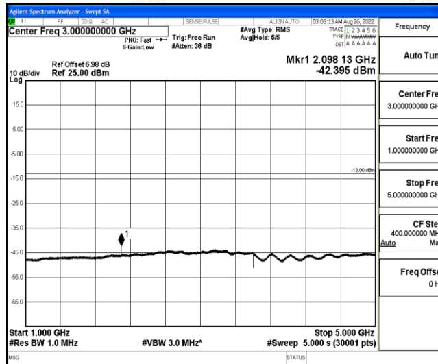
Band12-3MHz-16QAM-23025-1-0-Low-1000-5000--42.4-PASS
