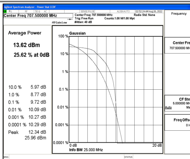
Band12-3MHz-QPSK-23095-6-0-Low-9.72-13-PASS
