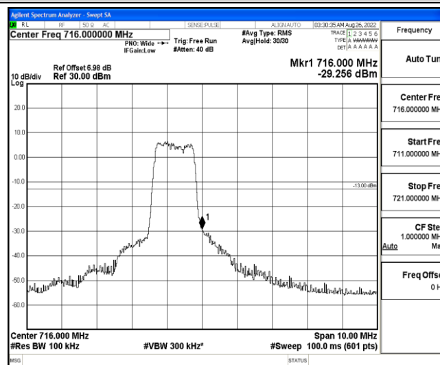
Band12-5MHz-QPSK-23155-6-0-High--29.26-PASS
