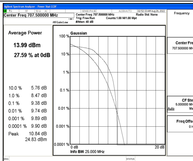
Band12-3MHz-16QAM-23095-6-0-Low-9.38-13-PASS
