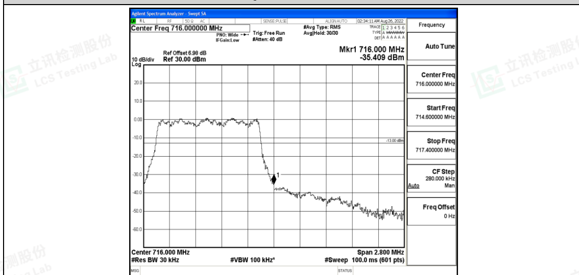
Band12-1.4MHz-16QAM-23173-6-0-High--35.41-PASS
