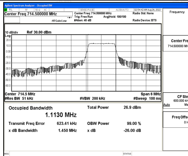
Band12-3MHz-16QAM-23165-6-0-High-1.1130-1.450-PASS
