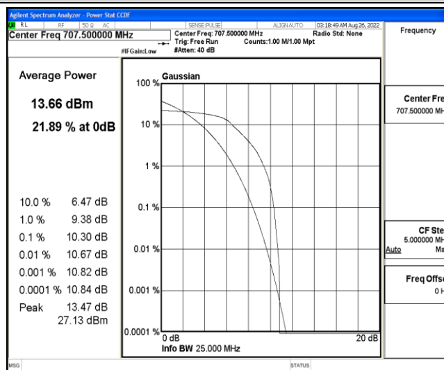
Band12-5MHz-16QAM-23095-6-0-Low-10.30-&lt;=13-PASS
