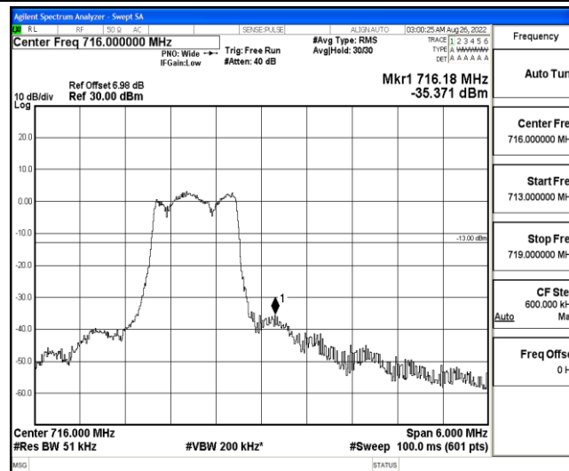
Band12-3MHz-QPSK-23165-6-0-High--35.37-PASS
