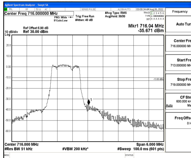
Band12-3MHz-16QAM-23165-6-0-High--35.67-PASS
