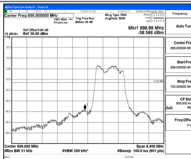
Band12-3MHz-16QAM-23025-6-0-Low--38.57-PASS
