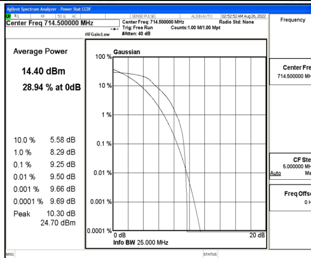
Band12-3MHz-16QAM-23165-6-0-High-9.25-&lt;=13-PASS
