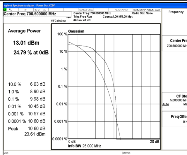
Band12-3MHz-QPSK-23025-6-0-Low-9.98-13-PASS
