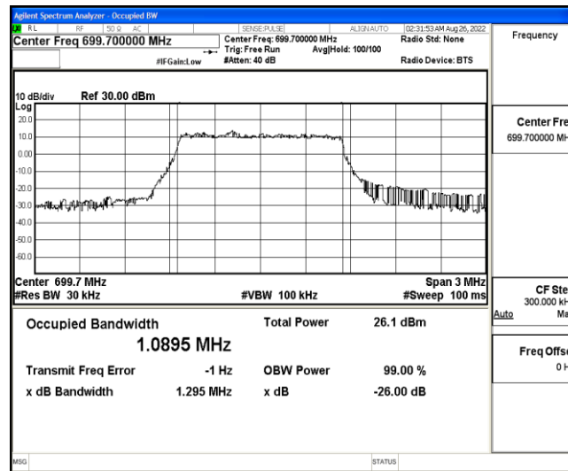
Band12-1.4MHz-QPSK-23017-6-0-Low-1.0895-1.295-PASS
