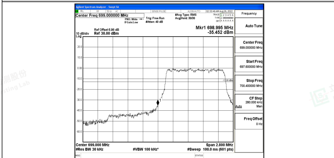
Band12-1.4MHz-16QAM-23017-6-0-Low--35.45-PASS
