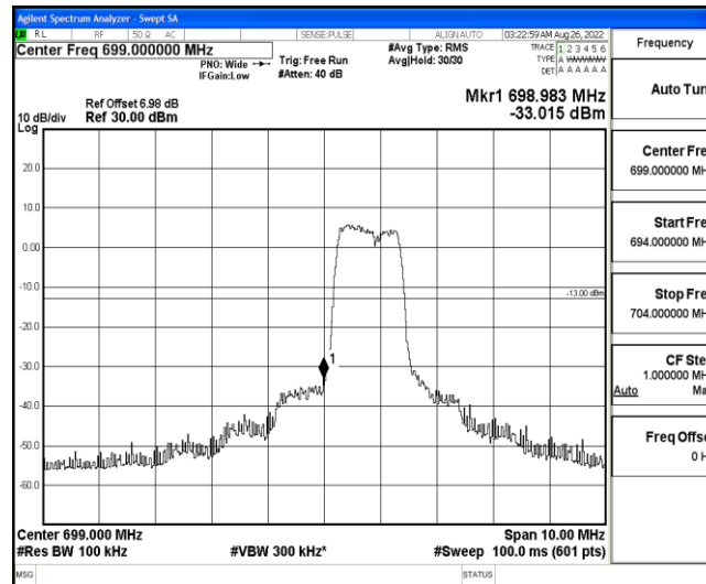
Band12-5MHz-QPSK-23035-6-0-Low--33.01-PASS
