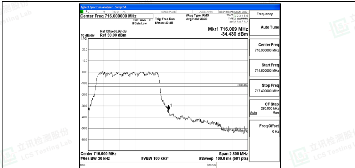
Band12-1.4MHz-QPSK-23173-6-0-High--34.43-PASS
