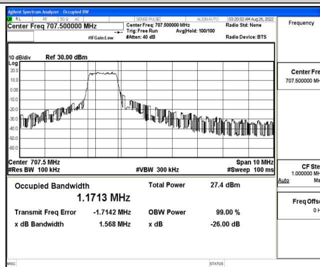
Band12-5MHz-QPSK-23095-6-0-Low-1.1713-1.568-PASS
