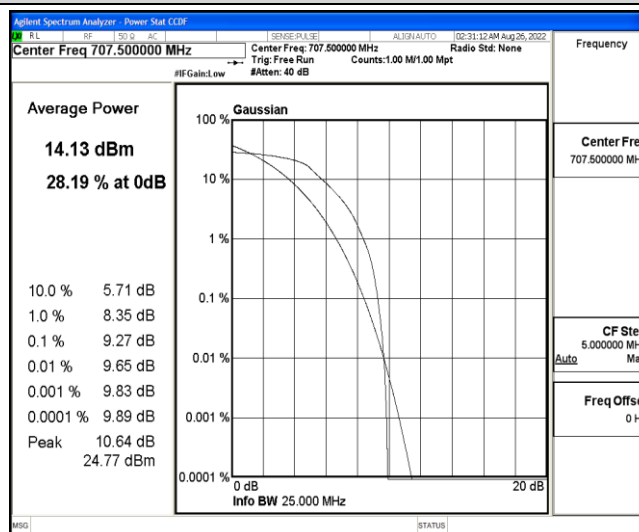
Band12-1.4MHz-16QAM-23095-6-0-Low-9.27-&lt;=13-PASS
