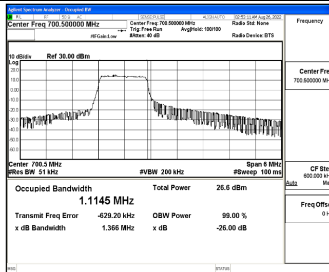
Band12-3MHz-QPSK-23025-6-0-Low-1.1145-1.366-PASS
