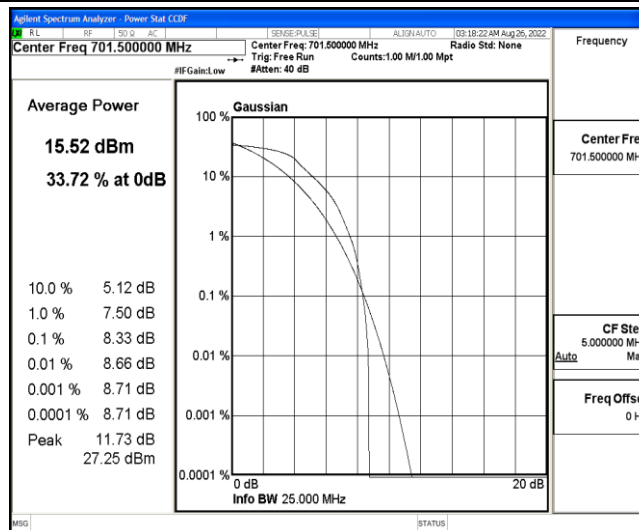
Band12-5MHz-QPSK-23035-6-0-Low-8.33-&lt;=13-PASS
