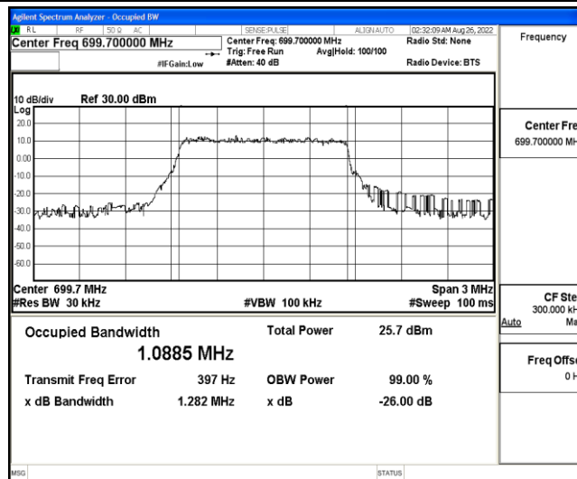
Band12-1.4MHz-16QAM-23017-6-0-Low-1.0885-1.282-PASS
