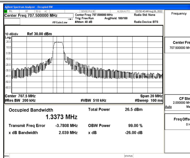
Band12-10MHz-16QAM-23095-6-0-Low-1.3373-2.039-PASS
