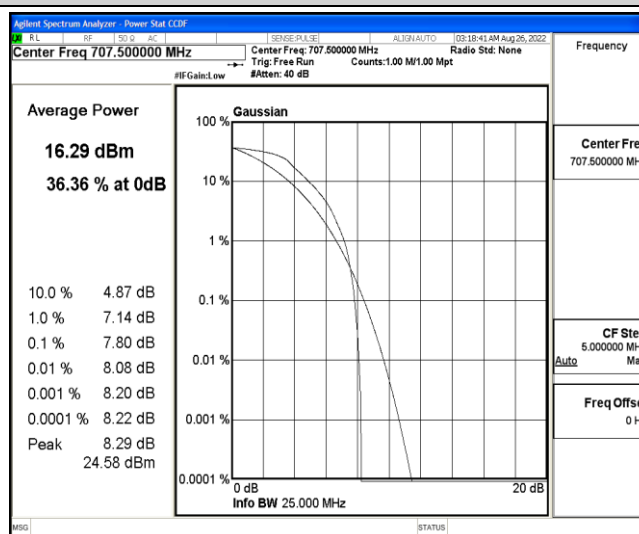
Band12-5MHz-QPSK-23095-6-0-Low-7.80-&lt;=13-PASS
