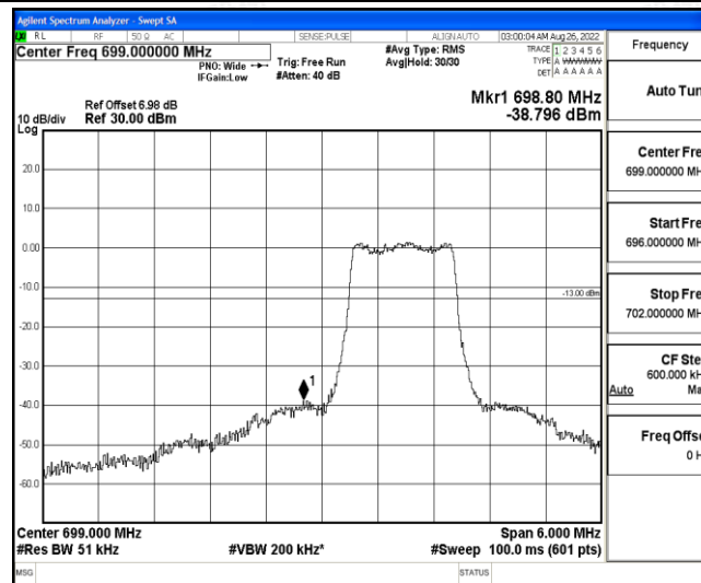
Band12-3MHz-QPSK-23025-6-0-Low--38.80-PASS
