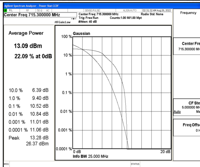
Band12-1.4MHz-16QAM-23173-6-0-High-10.52-13-PASS
