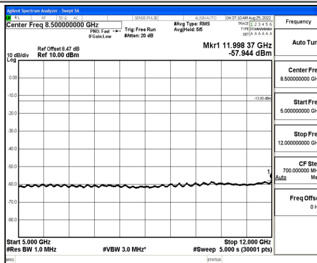
Band4-20MHz-16QAM-20300-1-0-High-5000-12000--57.94-PASS
