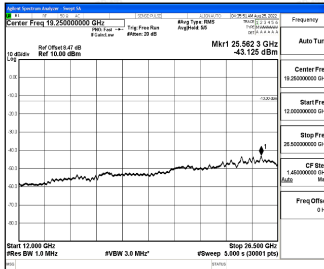
Band4-20MHz-QPSK-20300-1-0-High-12000-26500--43.13-PASS
