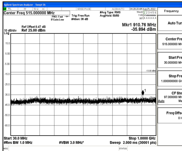
Band4-20MHz-16QAM-20050-1-0-Low-30-1000--35.89-PASS
