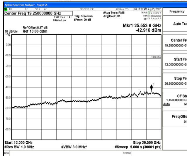
Band4-15MHz-16QAM-20325-1-0-High-12000-26500--42.92-PASS
