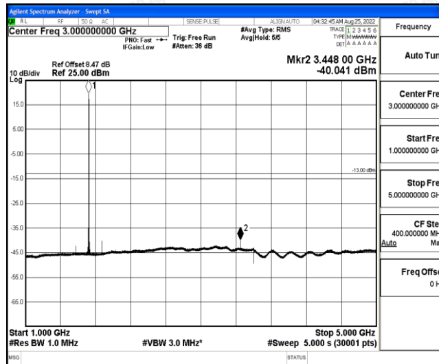
Band4-20MHz-16QAM-20175-1-0-Low-1000-5000--40.04-PASS
