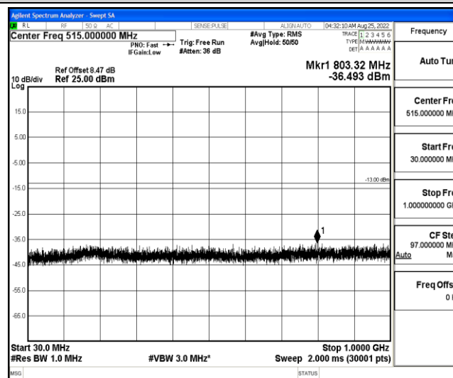
Band4-20MHz-16QAM-20175-1-0-Low-30-1000--36.49-PASS
