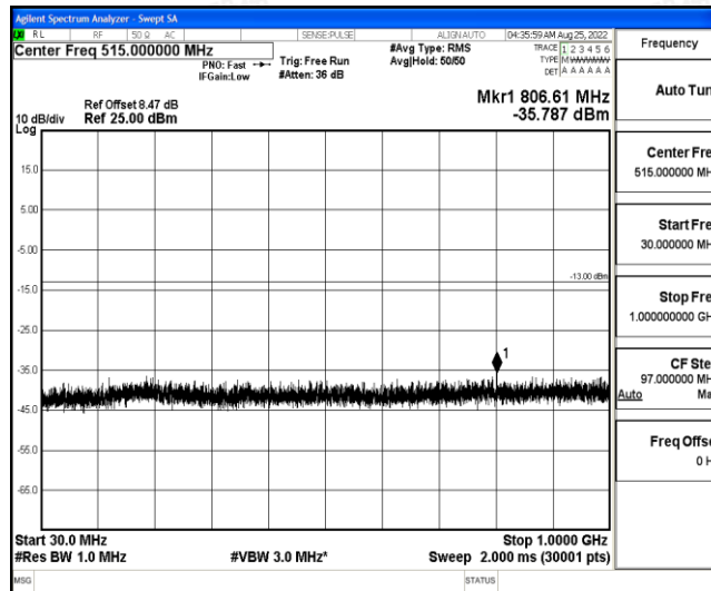
Band4-20MHz-16QAM-20300-1-0-High-30-1000--35.79-PASS
