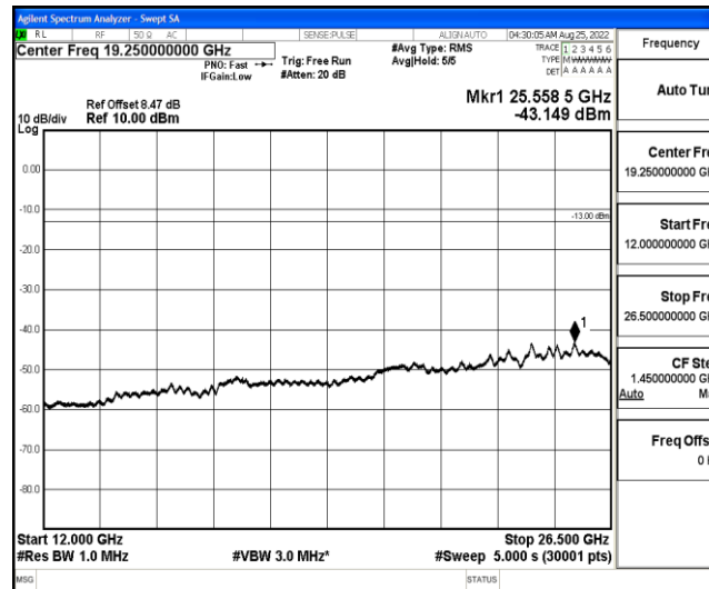
Band4-20MHz-16QAM-20050-1-0-Low-12000-26500--43.15-PASS
