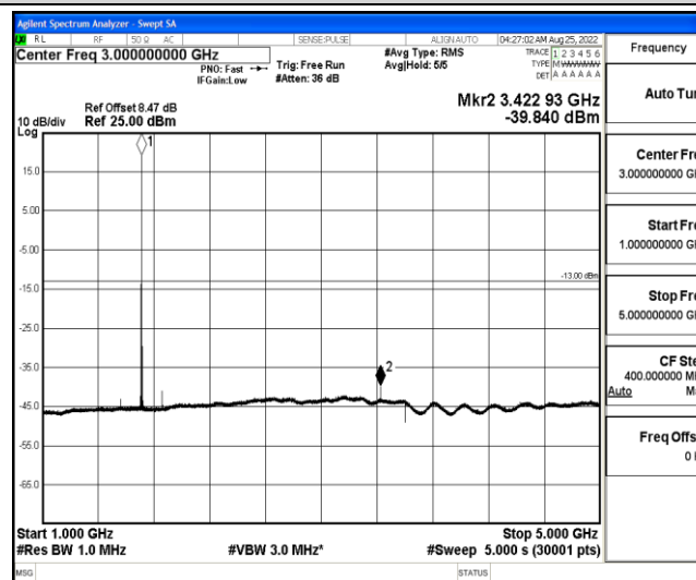
Band4-20MHz-QPSK-20050-1-0-Low-1000-5000--39.84-PASS
