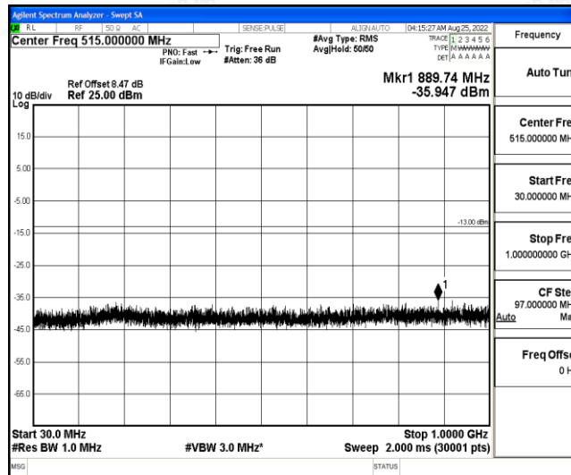
Band4-15MHz-16QAM-20325-1-0-High-30-1000--35.95-PASS
