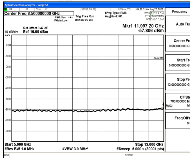
Band4-20MHz-16QAM-20050-1-0-Low-5000-12000--57.81-PASS
