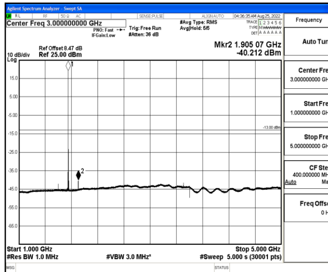
Band4-20MHz-16QAM-20300-1-0-High-1000-5000--40.21-PASS
