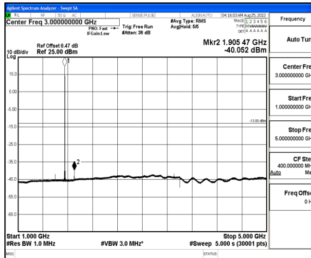
Band4-15MHz-16QAM-20325-1-0-High-1000-5000--40.05-PASS
