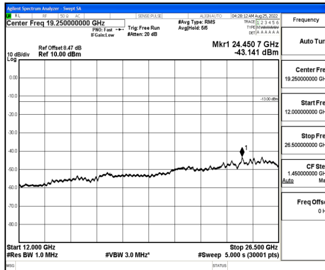
Band4-20MHz-QPSK-20050-1-0-Low-12000-26500--43.14-PASS
