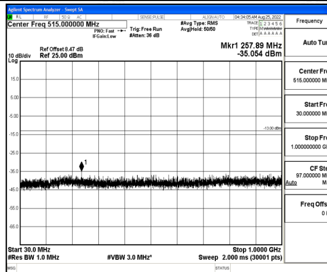
Band4-20MHz-QPSK-20300-1-0-High-30-1000--35.05-PASS
