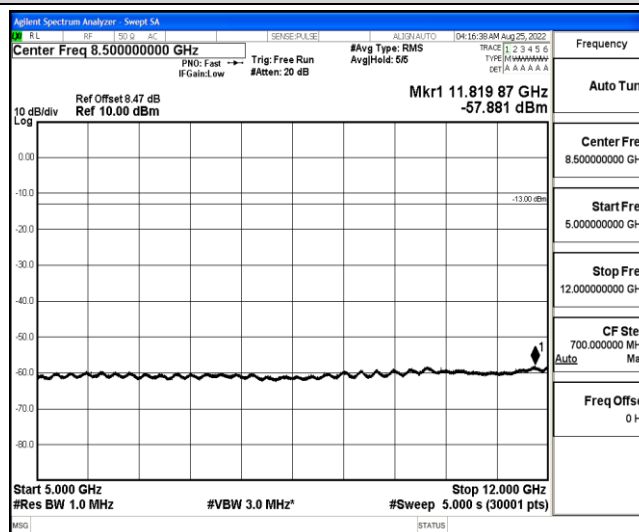
Band4-15MHz-16QAM-20325-1-0-High-5000-12000--57.88-PASS
