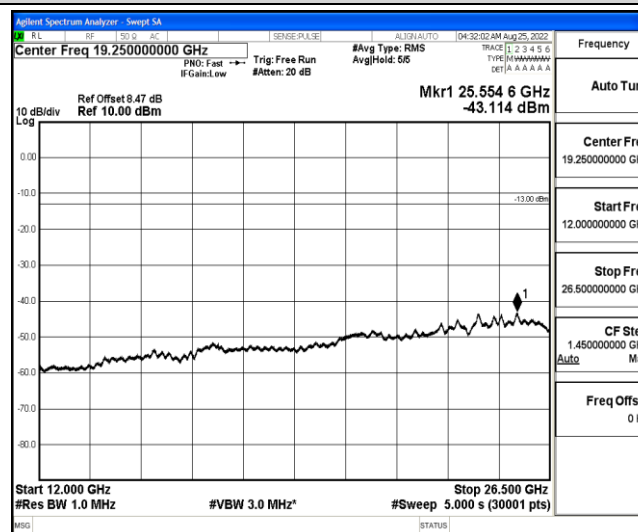
Band4-20MHz-QPSK-20175-1-0-Low-12000-26500--43.11-PASS
