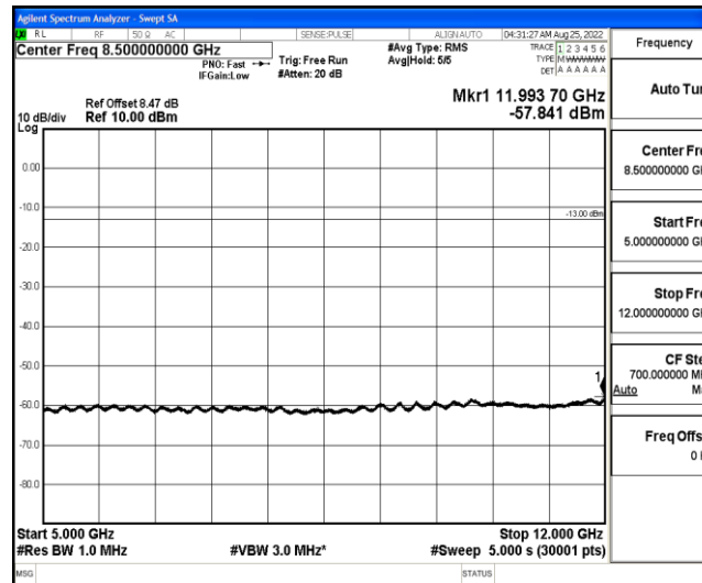
Band4-20MHz-QPSK-20175-1-0-Low-5000-12000--57.84-PASS
