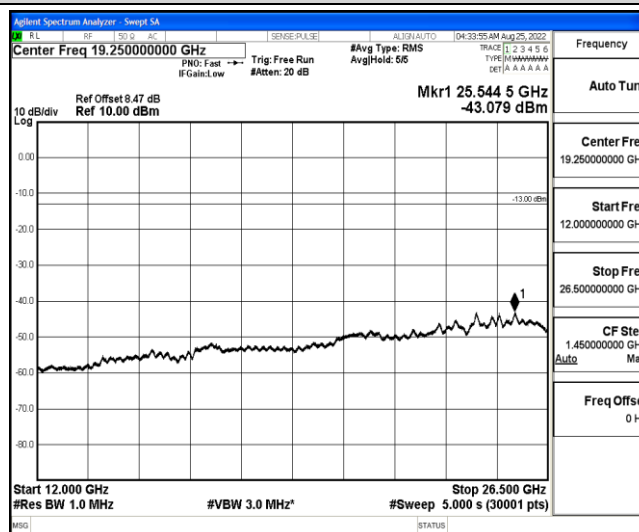
Band4-20MHz-16QAM-20175-1-0-Low-12000-26500--43.08-PASS
