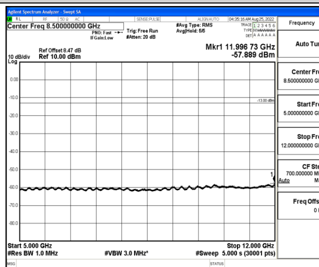
Band4-20MHz-QPSK-20300-1-0-High-5000-12000--57.89-PASS
