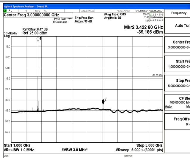
Band4-20MHz-16QAM-20050-1-0-Low-1000-5000--39.19-PASS
