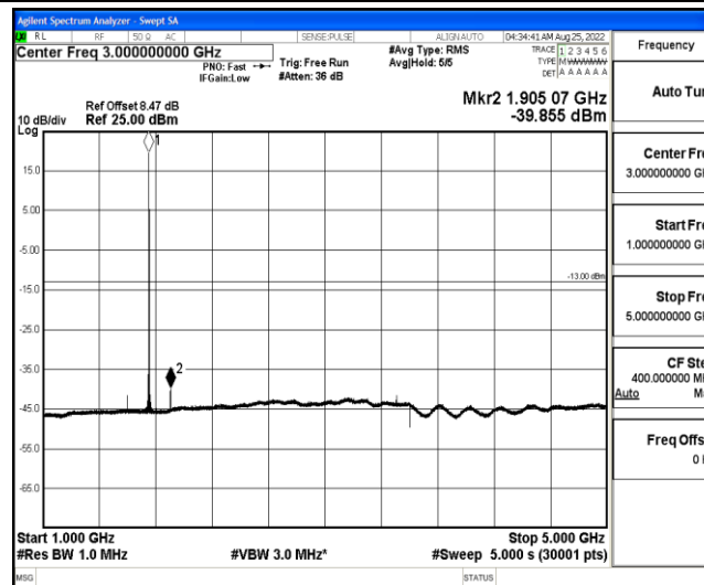
Band4-20MHz-QPSK-20300-1-0-High-1000-5000--39.86-PASS
