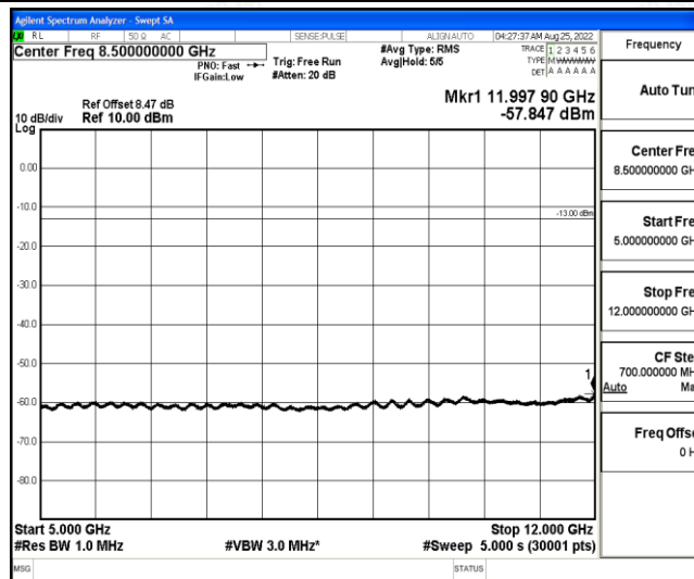
Band4-20MHz-QPSK-20050-1-0-Low-5000-12000--57.85-PASS
