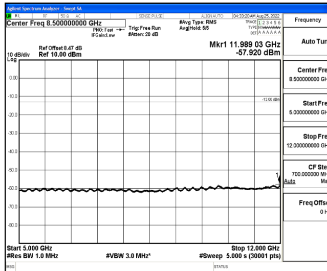
Band4-20MHz-16QAM-20175-1-0-Low-5000-12000--57.92-PASS
