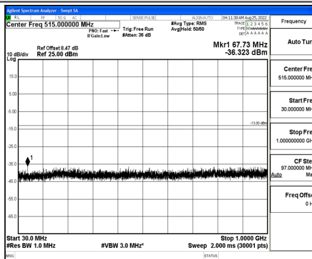
Band4-15MHz-16QAM-20175-1-0-Low-30-1000--36.32-PASS
