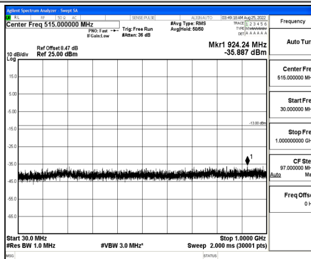
Band4-10MHz-QPSK-20175-1-0-Low-30-1000--35.89-PASS
