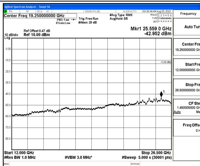
Band4-5MHz-QPSK-20175-1-0-Low-12000-26500--42.95-PASS
