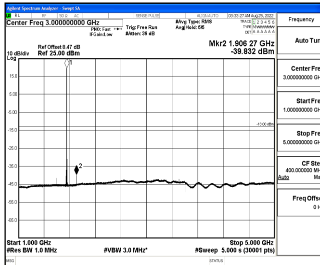
Band4-5MHz-QPSK-20375-1-0-High-1000-5000--39.83-PASS
