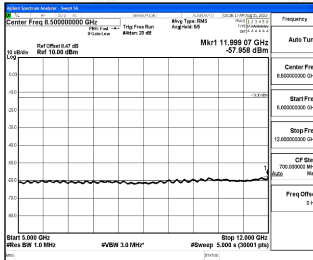
Band4-5MHz-16QAM-19975-1-0-Low-5000-12000--57.96-PASS
