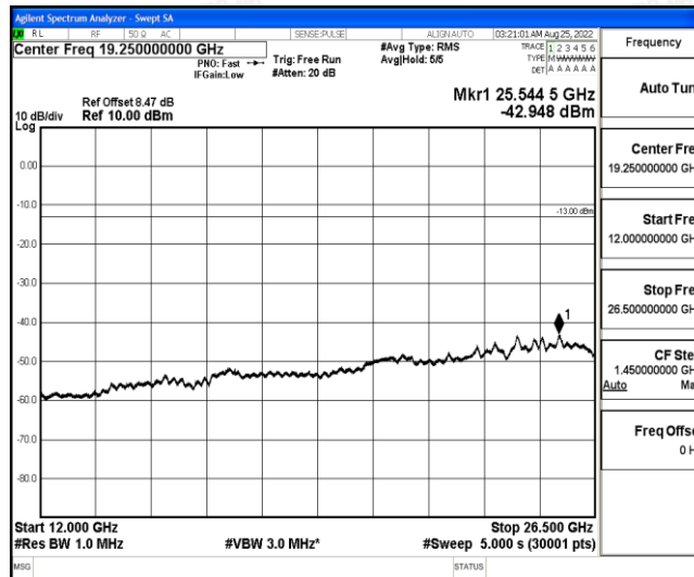
Band4-3MHz-16QAM-20385-1-0-High-12000-26500--42.95-PASS
