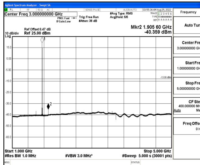
Band4-10MHz-16QAM-20350-1-0-High-1000-5000--40.36-PASS
