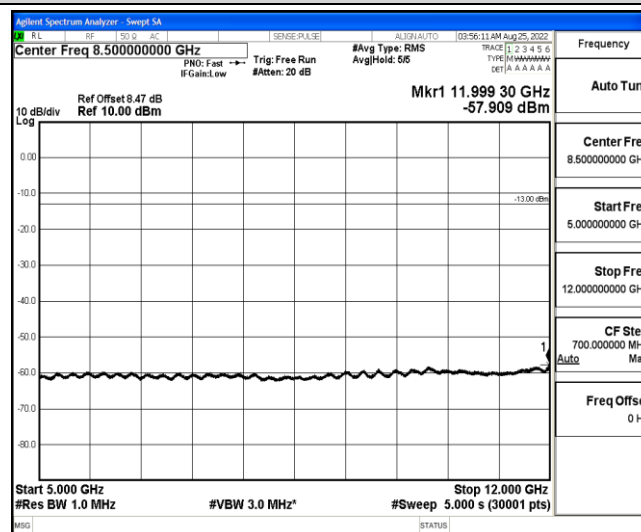
Band4-10MHz-16QAM-20350-1-0-High-5000-12000--57.91-PASS
