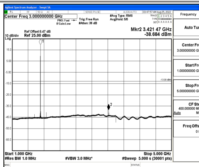
Band4-10MHz-16QAM-20000-1-0-Low-1000-5000--38.68-PASS
