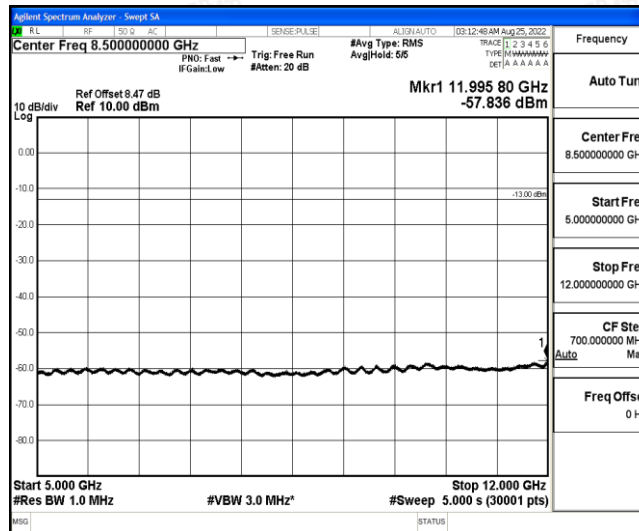
Band4-3MHz-16QAM-19965-1-0-Low-5000-12000--57.84-PASS
