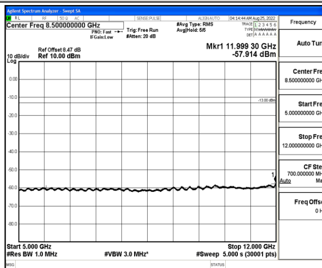
Band4-15MHz-QPSK-20325-1-0-High-5000-12000--57.91-PASS
