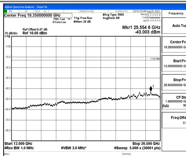
Band4-10MHz-QPSK-20175-1-0-Low-12000-26500--43-PASS
