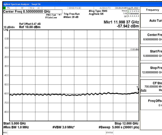
Band4-5MHz-QPSK-19975-1-0-Low-5000-12000--57.94-PASS
