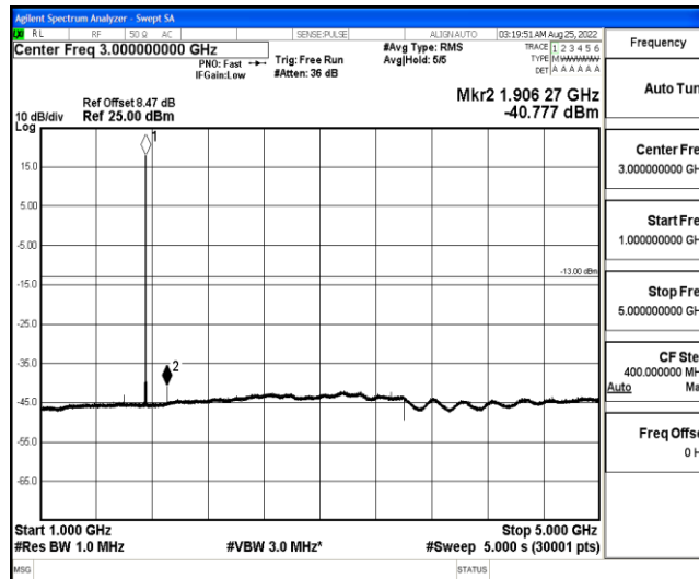
Band4-3MHz-16QAM-20385-1-0-High-1000-5000--40.78-PASS
