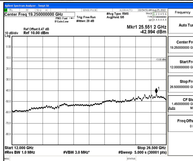
Band4-10MHz-QPSK-20350-1-0-High-12000-26500--42.99-PASS
