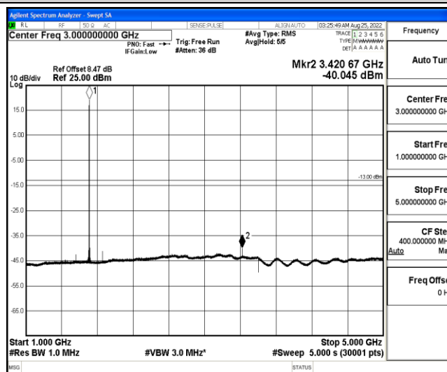
Band4-5MHz-QPSK-19975-1-0-Low-1000-5000--40.05-PASS
