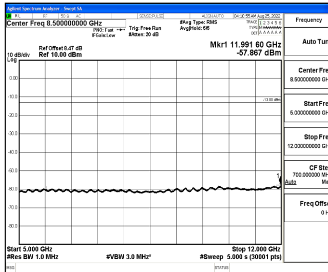
Band4-15MHz-QPSK-20175-1-0-Low-5000-12000--57.87-PASS
