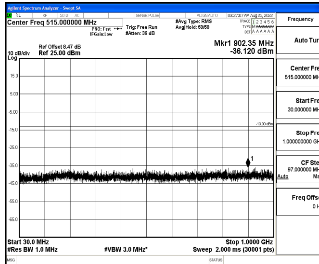
Band4-5MHz-16QAM-19975-1-0-Low-30-1000--36.12-PASS
