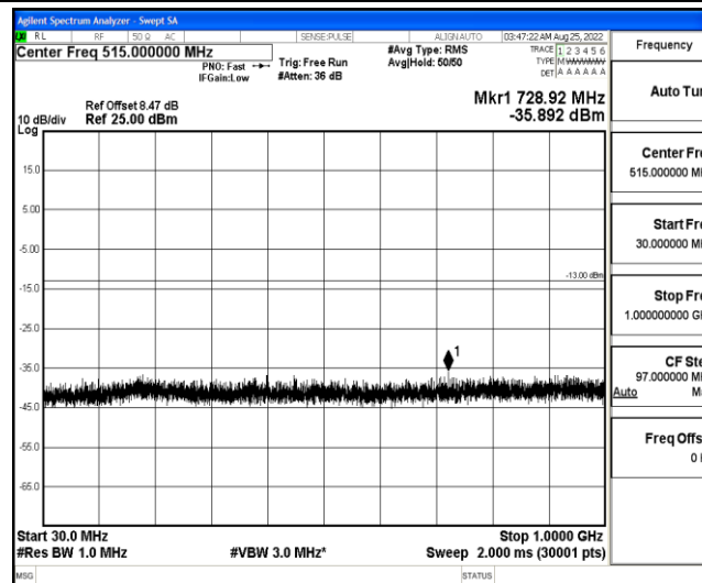
Band4-10MHz-16QAM-20000-1-0-Low-30-1000--35.89-PASS
