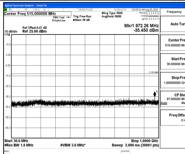
Band4-10MHz-16QAM-20350-1-0-High-30-1000--35.45-PASS
