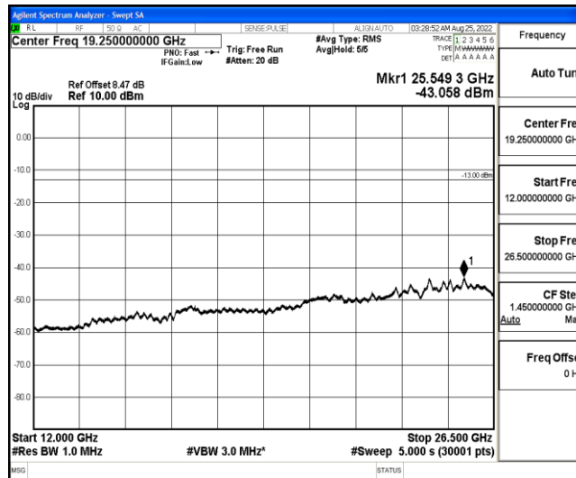
Band4-5MHz-16QAM-19975-1-0-Low-12000-26500--43.06-PASS
