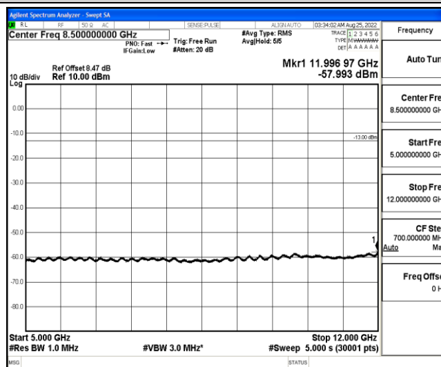
Band4-5MHz-QPSK-20375-1-0-High-5000-12000--57.99-PASS
