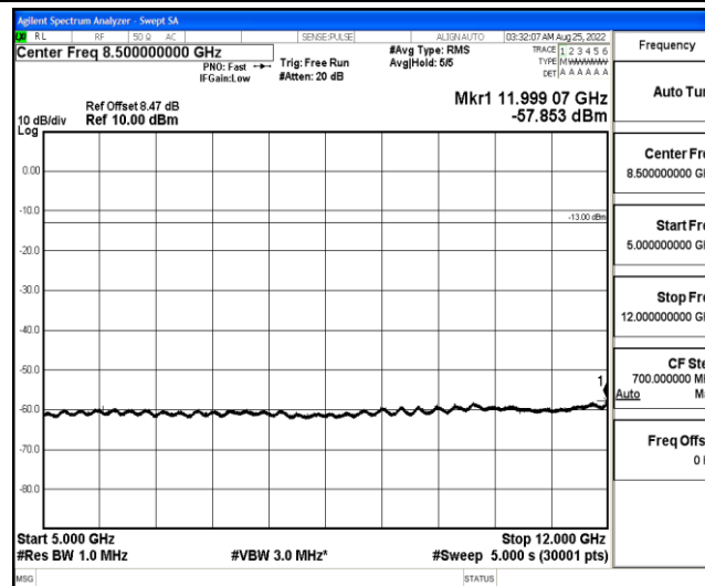
Band4-5MHz-16QAM-20175-1-0-Low-5000-12000--57.85-PASS
