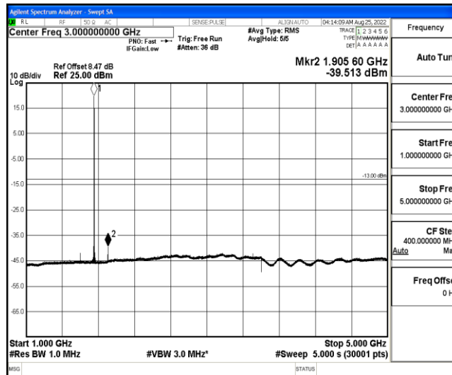
Band4-15MHz-QPSK-20325-1-0-High-1000-5000--39.51-PASS
