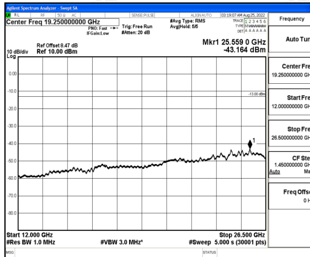
Band4-3MHz-QPSK-20385-1-0-High-12000-26500--43.16-PASS
