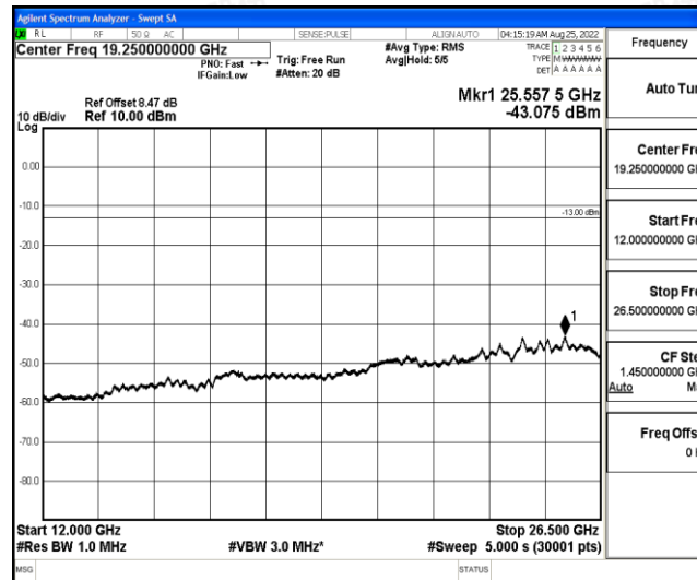
Band4-15MHz-QPSK-20325-1-0-High-12000-26500--43.08-PASS
