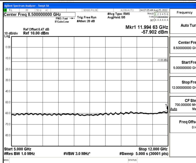
Band4-15MHz-QPSK-20025-1-0-Low-5000-12000--57.9-PASS
