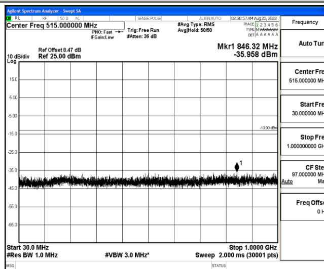
Band4-5MHz-16QAM-20175-1-0-Low-30-1000--35.96-PASS
