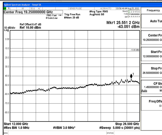
Band4-10MHz-16QAM-20350-1-0-High-12000-26500--43.05-PASS
