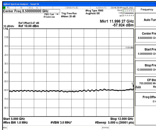
Band4-10MHz-QPSK-20000-1-0-Low-5000-12000--57.92-PASS
