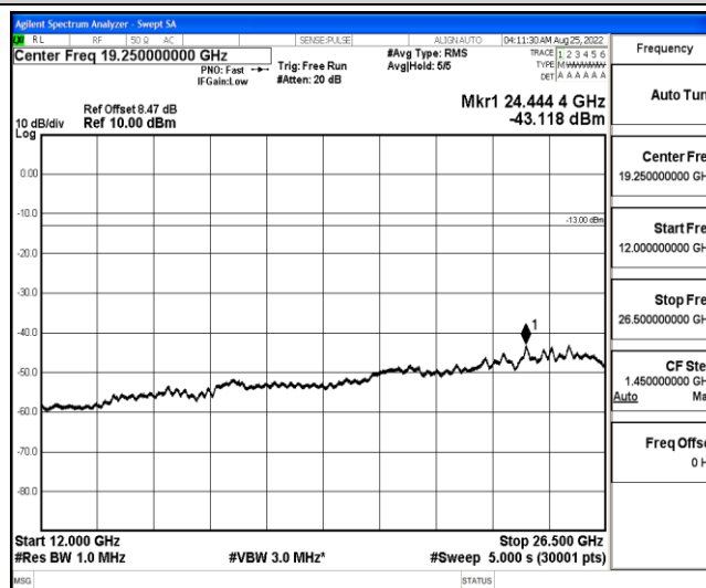
Band4-15MHz-QPSK-20175-1-0-Low-12000-26500--43.12-PASS
