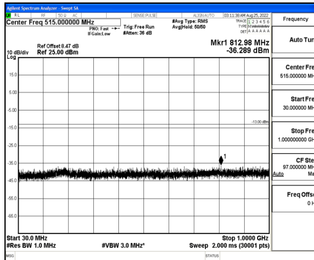
Band4-3MHz-16QAM-19965-1-0-Low-30-1000--36.29-PASS
