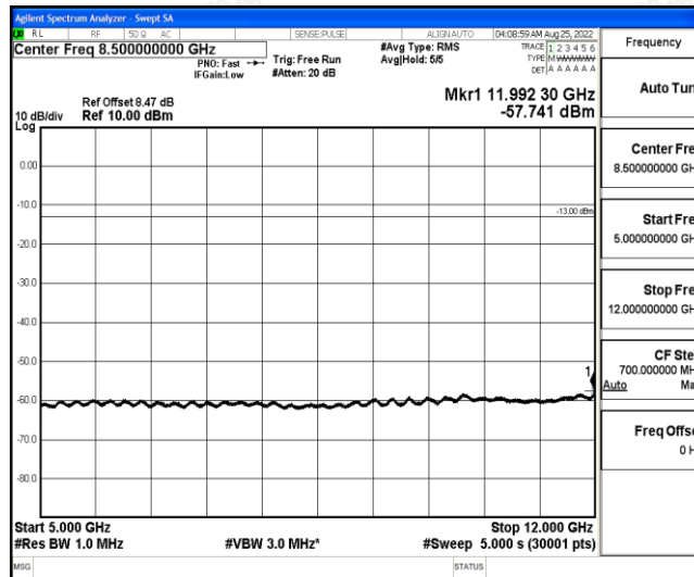
Band4-15MHz-16QAM-20025-1-0-Low-5000-12000--57.74-PASS
