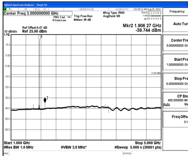
Band4-5MHz-16QAM-20375-1-0-High-1000-5000--39.74-PASS
