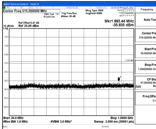
Band4-3MHz-16QAM-20385-1-0-High-30-1000--35.84-PASS
