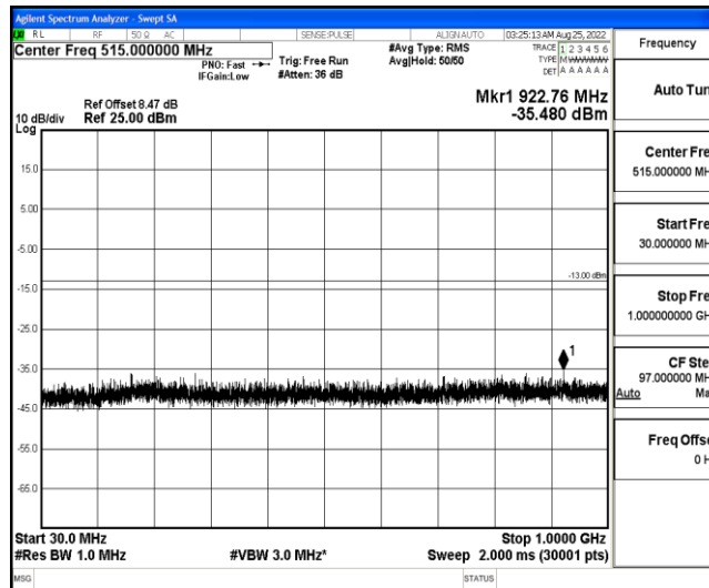
Band4-5MHz-QPSK-19975-1-0-Low-30-1000--35.48-PASS
