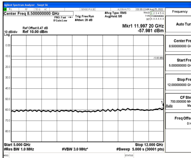
Band4-5MHz-QPSK-20175-1-0-Low-5000-12000--57.98-PASS
