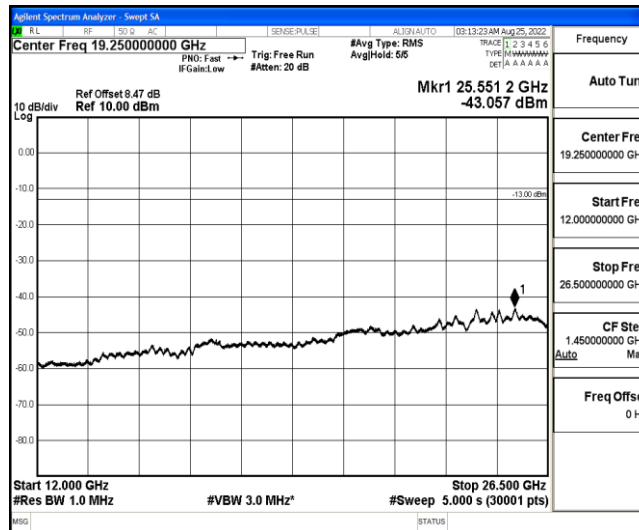
Band4-3MHz-16QAM-19965-1-0-Low-12000-26500--43.06-PASS
