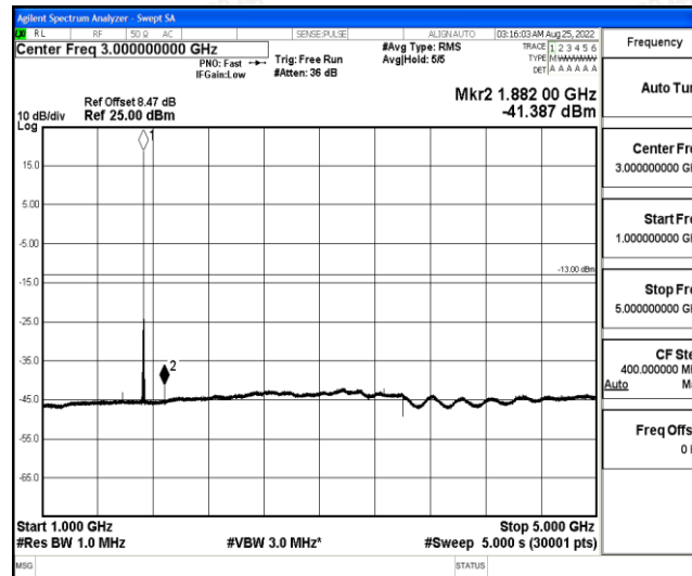
Band4-3MHz-16QAM-20175-1-0-Low-1000-5000--41.39-PASS
