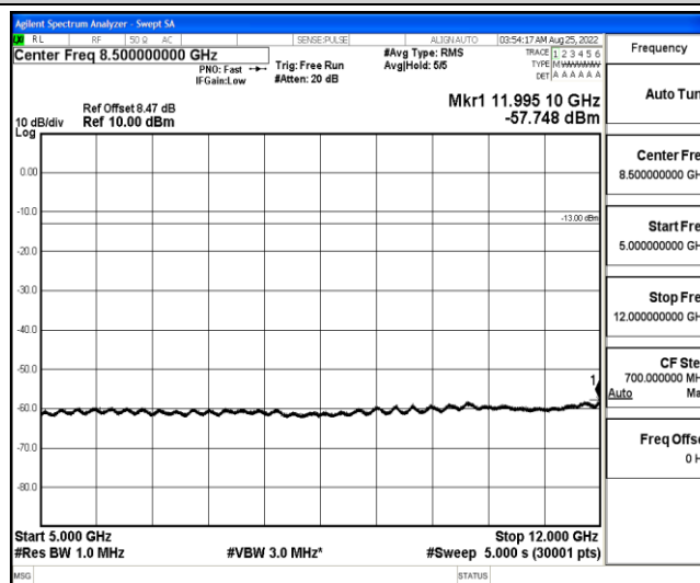
Band4-10MHz-QPSK-20350-1-0-High-5000-12000--57.75-PASS
