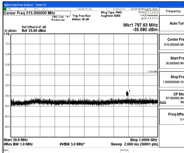
Band4-5MHz-16QAM-20375-1-0-High-30-1000--35.58-PASS
