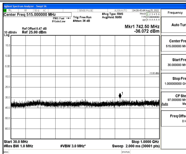
Band4-15MHz-QPSK-20175-1-0-Low-30-1000--36.07-PASS
