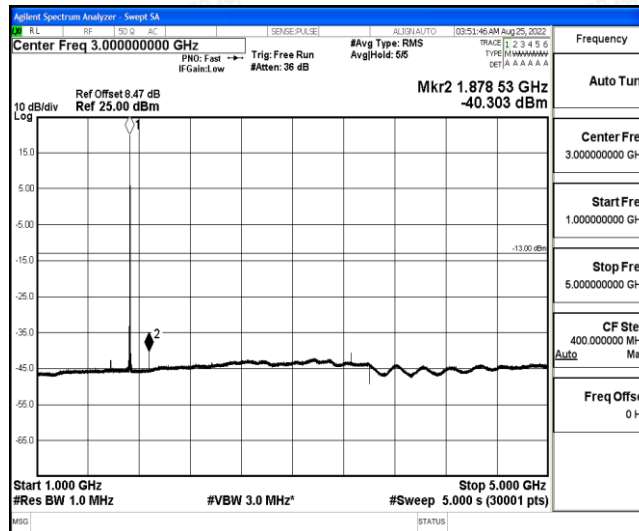
Band4-10MHz-16QAM-20175-1-0-Low-1000-5000--40.3-PASS
