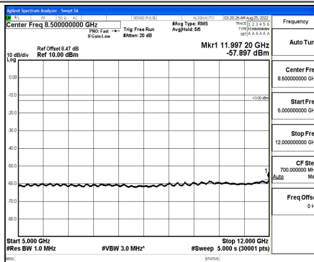
Band4-3MHz-16QAM-20385-1-0-High-5000-12000--57.9-PASS
