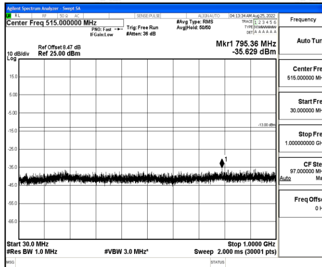
Band4-15MHz-QPSK-20325-1-0-High-30-1000--35.63-PASS
