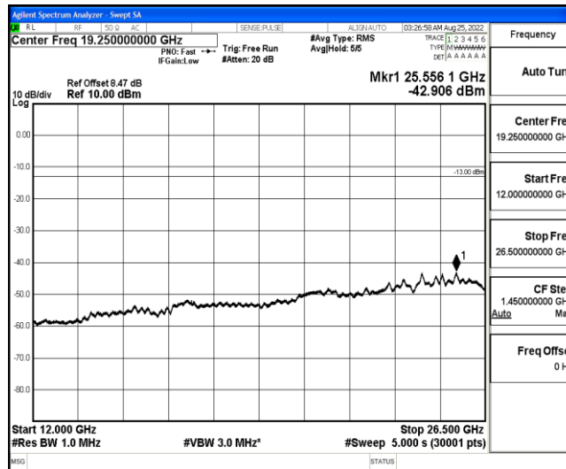
Band4-5MHz-QPSK-19975-1-0-Low-12000-26500--42.91-PASS
