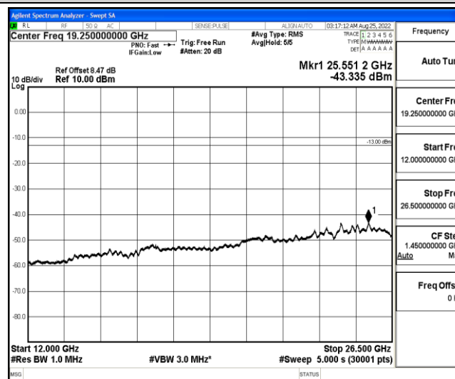
Band4-3MHz-16QAM-20175-1-0-Low-12000-26500--43.34-PASS
