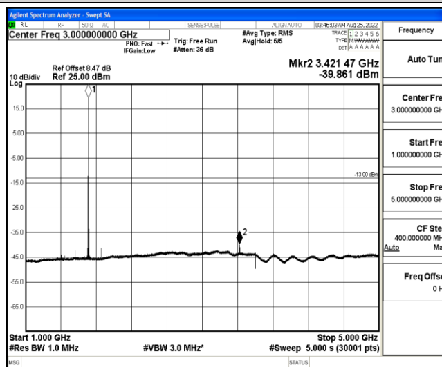
Band4-10MHz-QPSK-20000-1-0-Low-1000-5000--39.86-PASS
