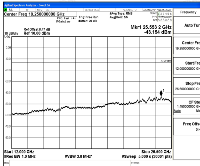
Band4-5MHz-16QAM-20375-1-0-High-12000-26500--43.15-PASS
