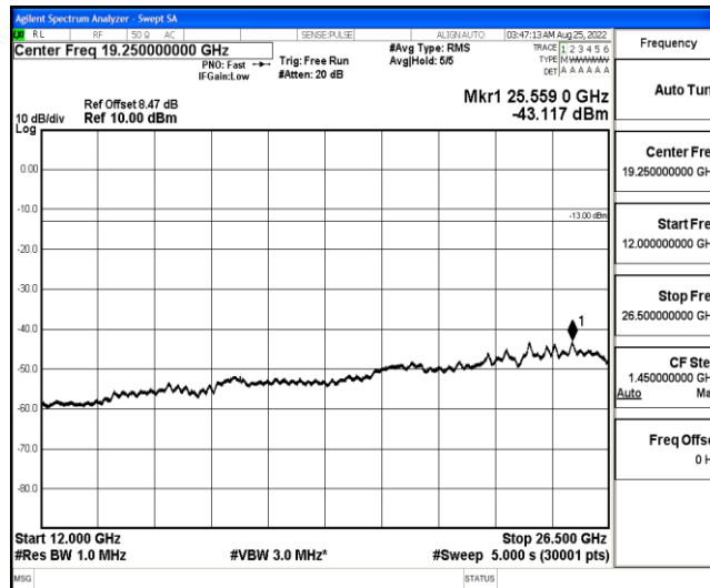
Band4-10MHz-QPSK-20000-1-0-Low-12000-26500--43.12-PASS
