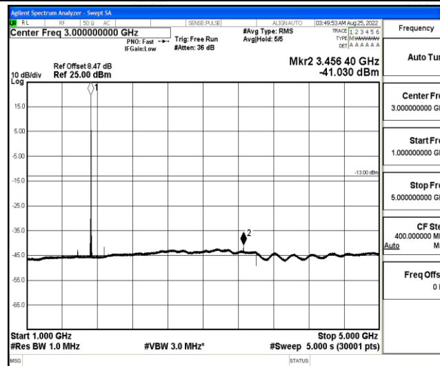
Band4-10MHz-QPSK-20175-1-0-Low-1000-5000--41.03-PASS
