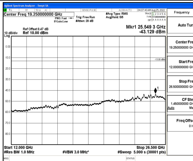
Band4-15MHz-QPSK-20025-1-0-Low-12000-26500--43.13-PASS
