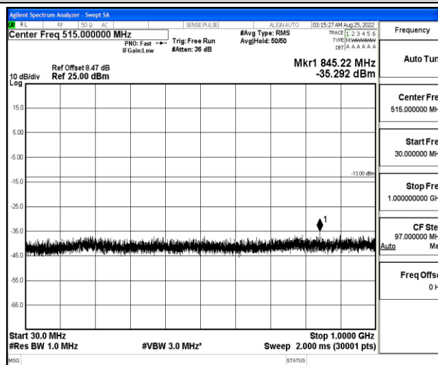
Band4-3MHz-16QAM-20175-1-0-Low-30-1000--35.29-PASS
