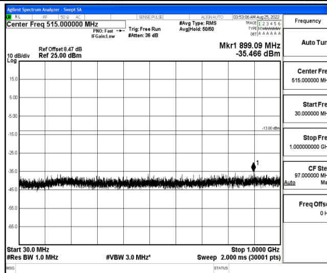
Band4-10MHz-QPSK-20350-1-0-High-30-1000--35.47-PASS
