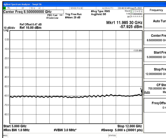
Band4-10MHz-16QAM-20000-1-0-Low-5000-12000--57.93-PASS
