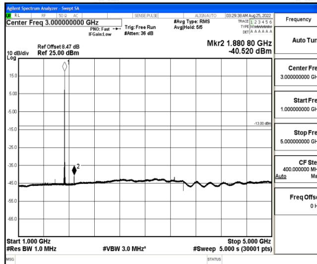
Band4-5MHz-QPSK-20175-1-0-Low-1000-5000--40.52-PASS
