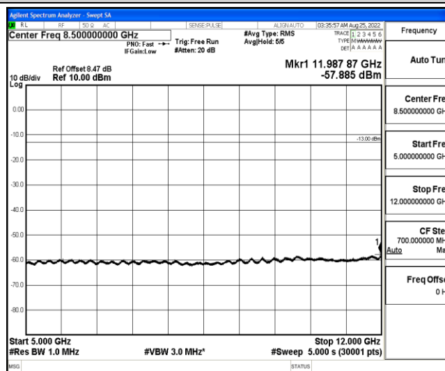
Band4-5MHz-16QAM-20375-1-0-High-5000-12000--57.89-PASS
