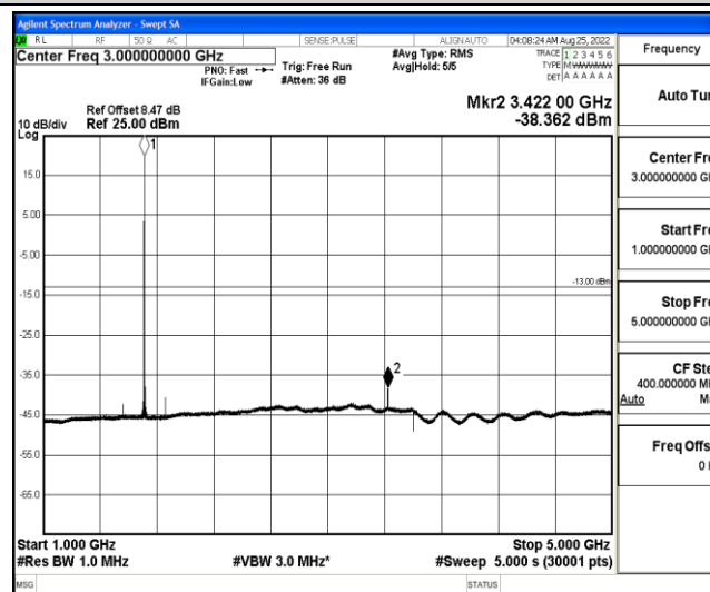
Band4-15MHz-16QAM-20025-1-0-Low-1000-5000--38.36-PASS
