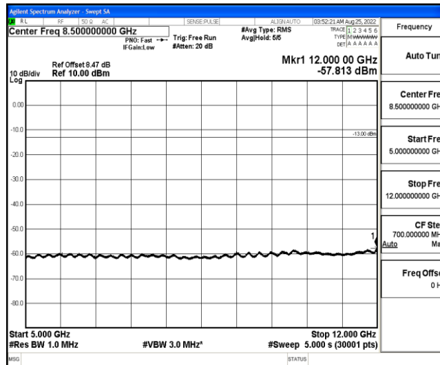
Band4-10MHz-16QAM-20175-1-0-Low-5000-12000--57.81-PASS
