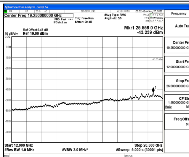
Band4-5MHz-16QAM-20175-1-0-Low-12000-26500--43.24-PASS
