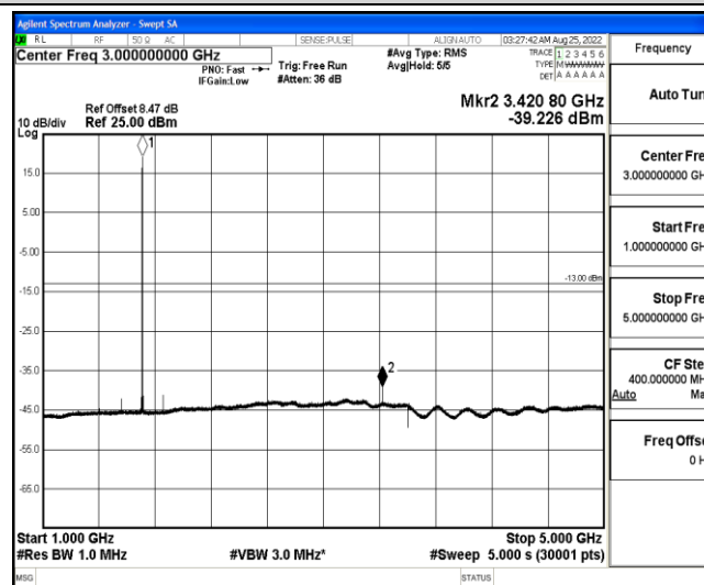
Band4-5MHz-16QAM-19975-1-0-Low-1000-5000--39.23-PASS
