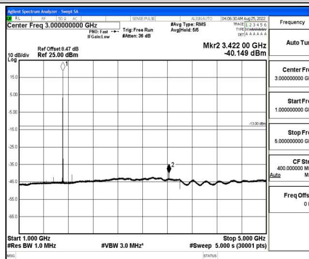
Band4-15MHz-QPSK-20025-1-0-Low-1000-5000--40.15-PASS
