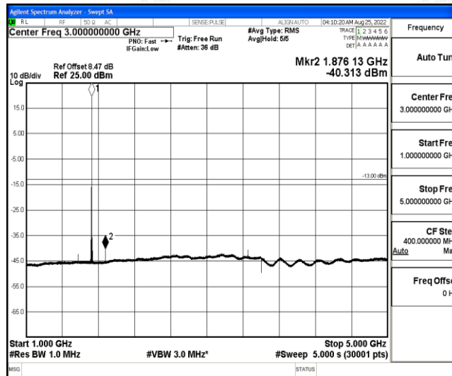
Band4-15MHz-QPSK-20175-1-0-Low-1000-5000--40.31-PASS
