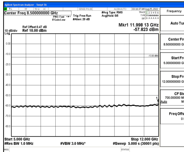
Band4-3MHz-16QAM-20175-1-0-Low-5000-12000--57.82-PASS
