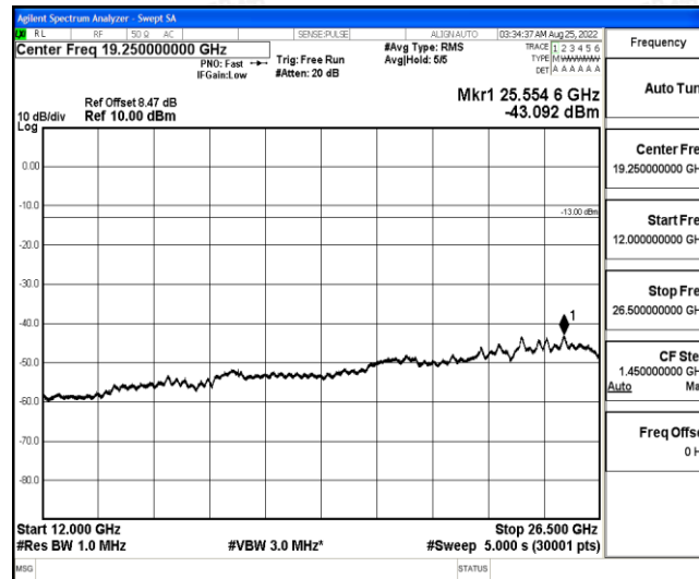
Band4-5MHz-QPSK-20375-1-0-High-12000-26500--43.09-PASS
