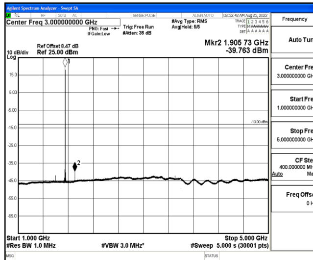
Band4-10MHz-QPSK-20350-1-0-High-1000-5000--39.76-PASS
