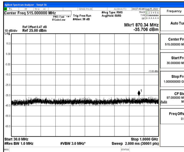
Band4-15MHz-16QAM-20025-1-0-Low-30-1000--35.71-PASS
