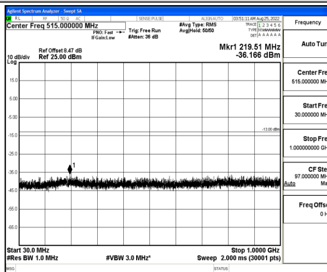
Band4-10MHz-16QAM-20175-1-0-Low-30-1000--36.17-PASS
