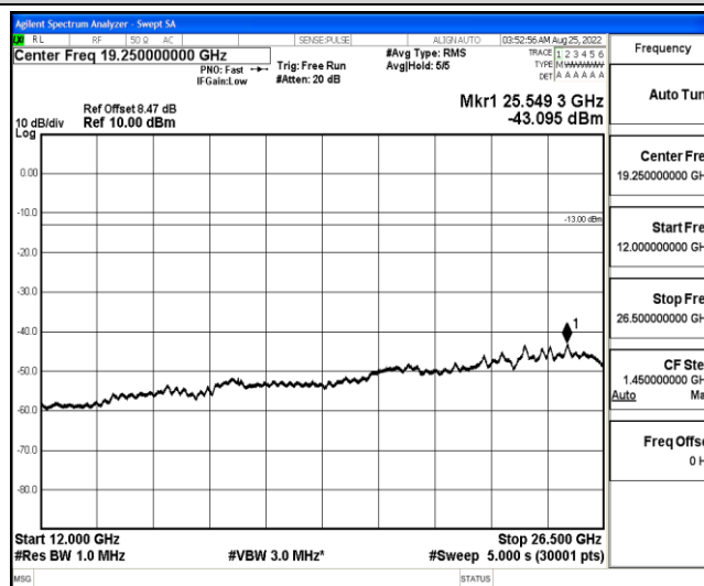
Band4-10MHz-16QAM-20175-1-0-Low-12000-26500--43.1-PASS
