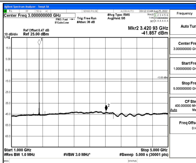
Band4-3MHz-16QAM-19965-1-0-Low-1000-5000--41.86-PASS
