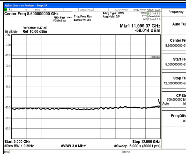
Band4-15MHz-16QAM-20175-1-0-Low-5000-12000--58.01-PASS
