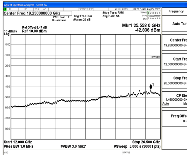
Band4-15MHz-16QAM-20025-1-0-Low-12000-26500--42.84-PASS
