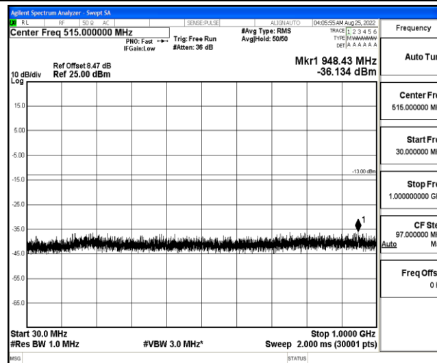
Band4-15MHz-QPSK-20025-1-0-Low-30-1000--36.13-PASS
