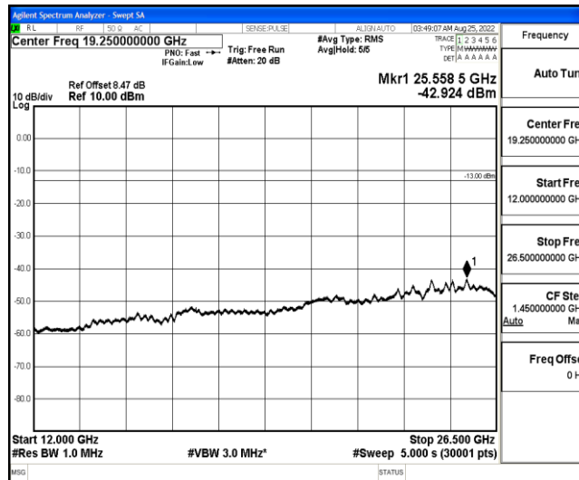
Band4-10MHz-16QAM-20000-1-0-Low-12000-26500--42.92-PASS
