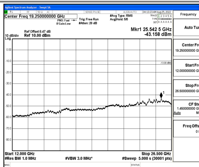
Band4-15MHz-16QAM-20175-1-0-Low-12000-26500--43.16-PASS
