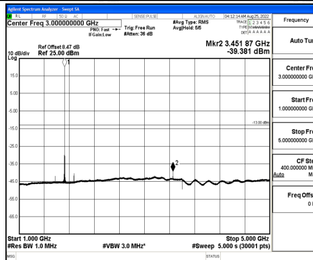
Band4-15MHz-16QAM-20175-1-0-Low-1000-5000--39.38-PASS
