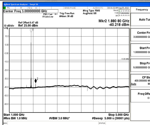
Band4-5MHz-16QAM-20175-1-0-Low-1000-5000--40.22-PASS
