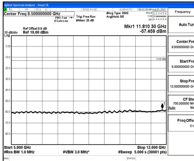
Band2-15MHz-16QAM-18900-1-0-Low-5000-12000--57.46-PASS
