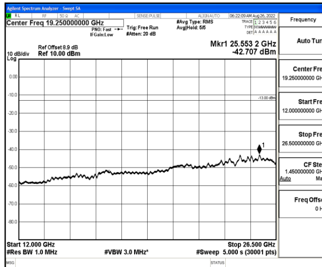
Band2-20MHz-16QAM-18700-1-0-Low-12000-26500--42.71-PASS
