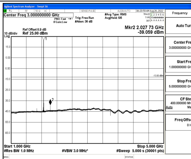
Band2-20MHz-16QAM-18700-1-0-Low-1000-5000--39.06-PASS
