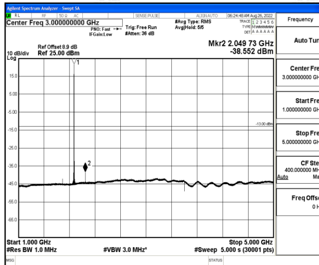
Band2-20MHz-16QAM-18900-1-0-Low-1000-5000--38.55-PASS
