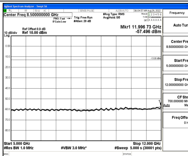
Band2-15MHz-16QAM-19125-1-0-High-5000-12000--57.5-PASS
