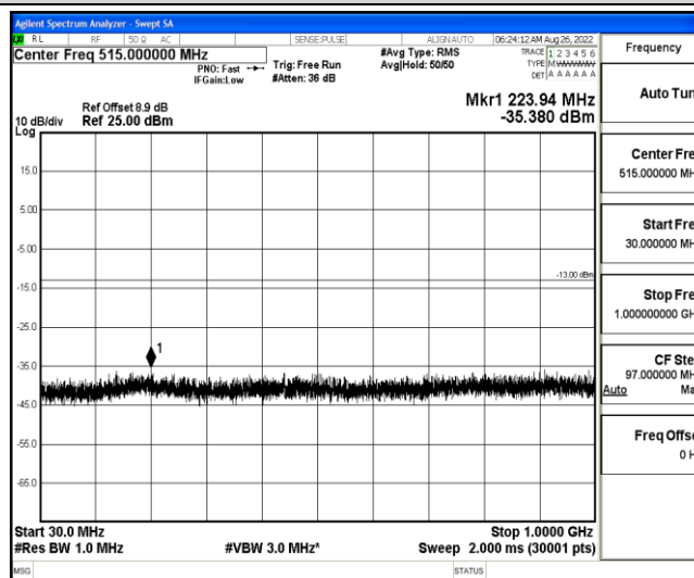
Band2-20MHz-16QAM-18900-1-0-Low-30-1000--35.38-PASS
