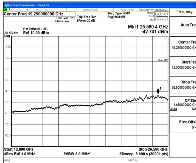
Band2-20MHz-QPSK-18700-1-0-Low-12000-26500--42.74-PASS
