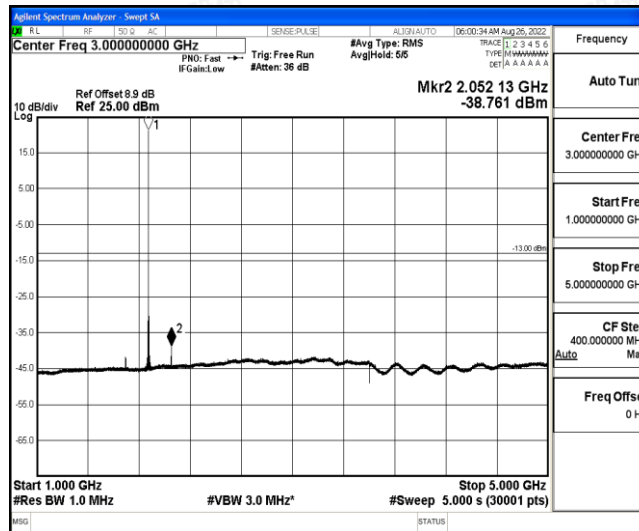
Band2-15MHz-16QAM-18900-1-0-Low-1000-5000--38.76-PASS
