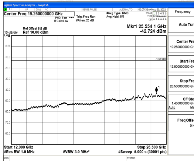
Band2-15MHz-16QAM-19125-1-0-High-12000-26500--42.72-PASS
