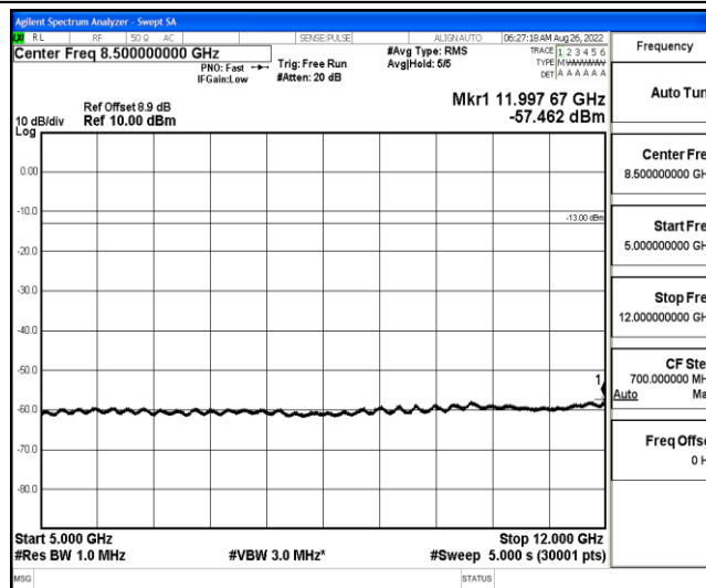
Band2-20MHz-QPSK-19100-1-0-High-5000-12000--57.46-PASS
