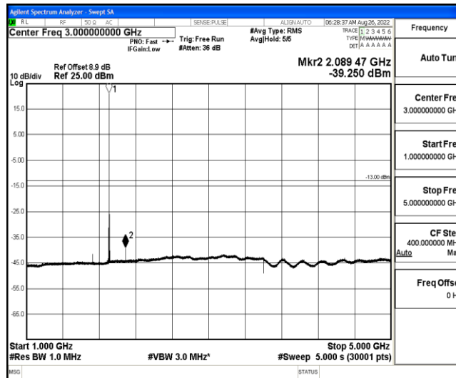
Band2-20MHz-16QAM-19100-1-0-High-1000-5000--39.25-PASS
