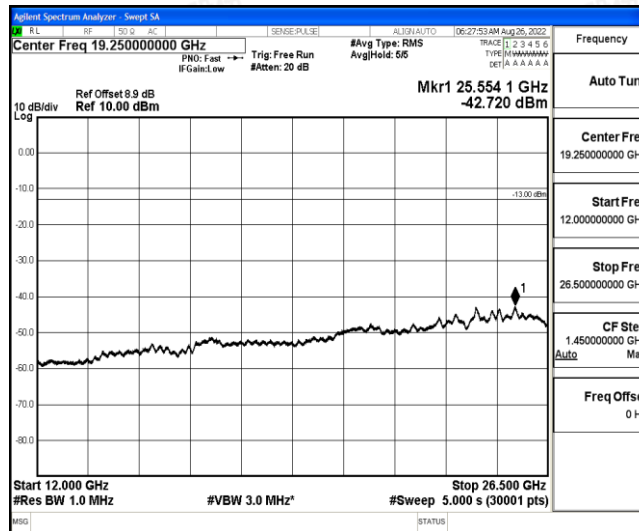
Band2-20MHz-QPSK-19100-1-0-High-12000-26500--42.72-PASS
