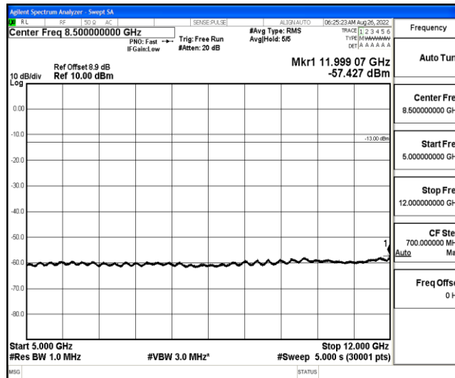
Band2-20MHz-16QAM-18900-1-0-Low-5000-12000--57.43-PASS
