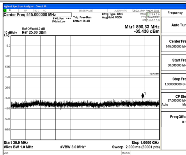
Band2-20MHz-QPSK-18900-1-0-Low-30-1000--35.44-PASS
