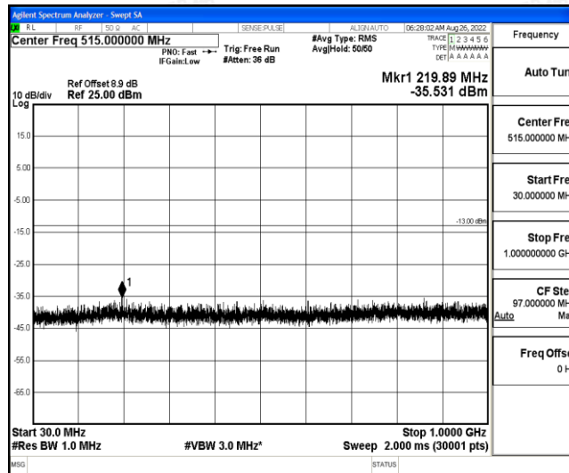
Band2-20MHz-16QAM-19100-1-0-High-30-1000--35.53-PASS
