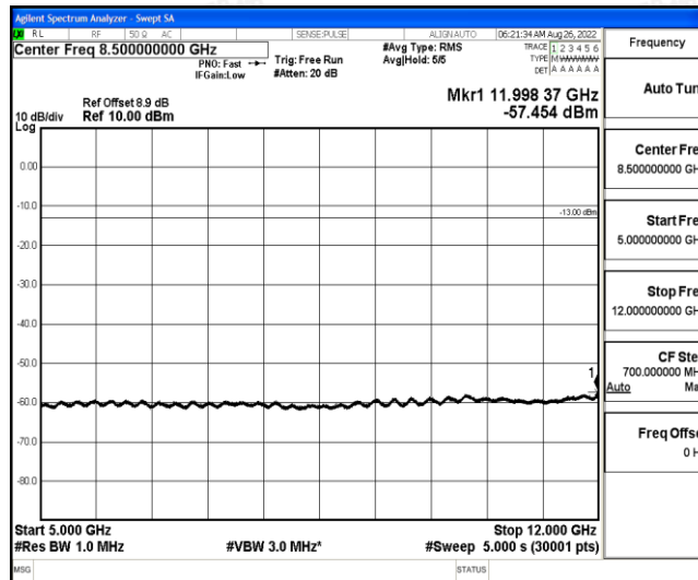
Band2-20MHz-16QAM-18700-1-0-Low-5000-12000--57.45-PASS
