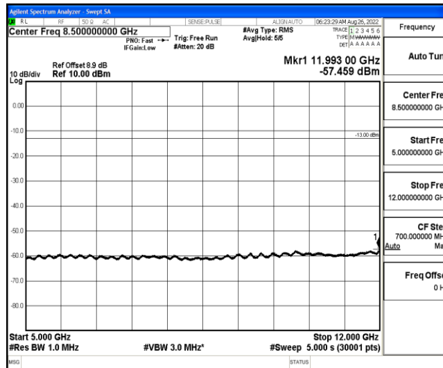
Band2-20MHz-QPSK-18900-1-0-Low-5000-12000--57.46-PASS
