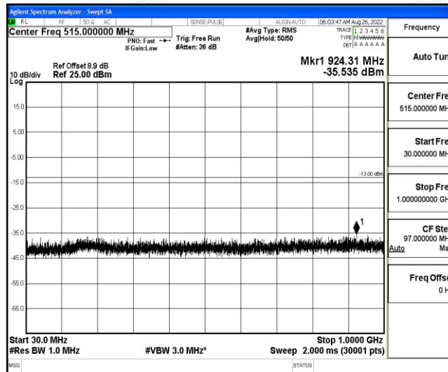
Band2-15MHz-16QAM-19125-1-0-High-30-1000--35.54-PASS
