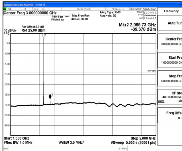
Band2-15MHz-16QAM-19125-1-0-High-1000-5000--39.37-PASS
