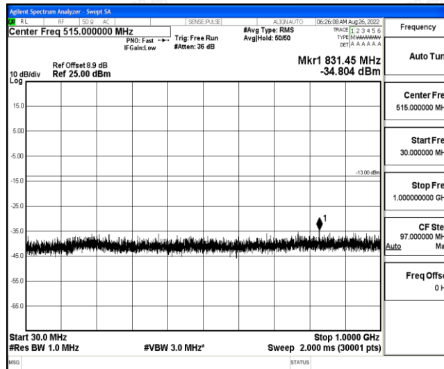
Band2-20MHz-QPSK-19100-1-0-High-30-1000--34.8-PASS
