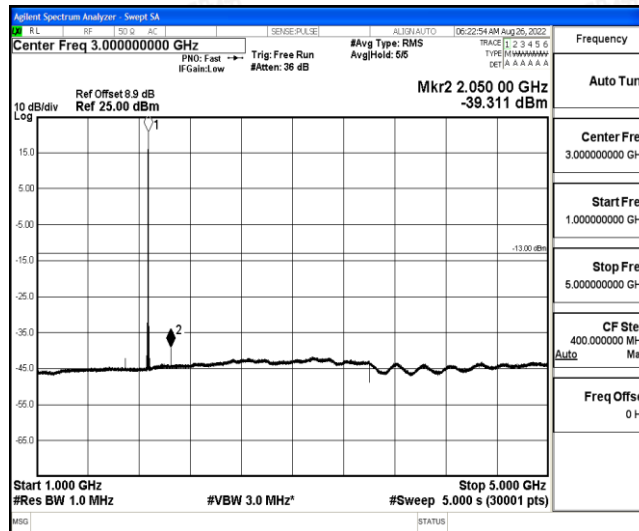
Band2-20MHz-QPSK-18900-1-0-Low-1000-5000--39.31-PASS
