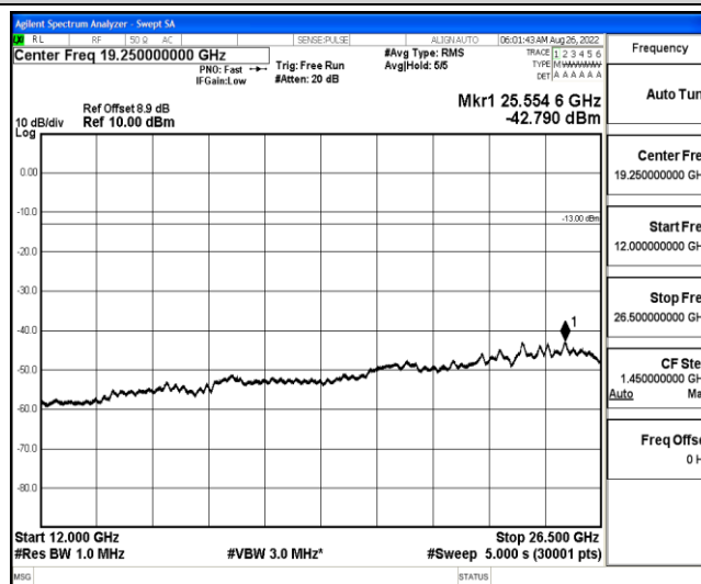
Band2-15MHz-16QAM-18900-1-0-Low-12000-26500--42.79-PASS
