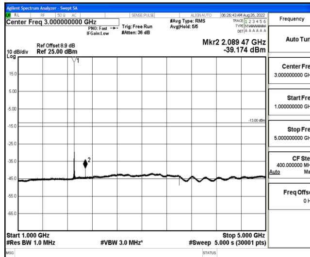
Band2-20MHz-QPSK-19100-1-0-High-1000-5000--39.17-PASS
