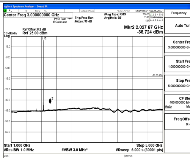
Band2-20MHz-QPSK-18700-1-0-Low-1000-5000--38.72-PASS
