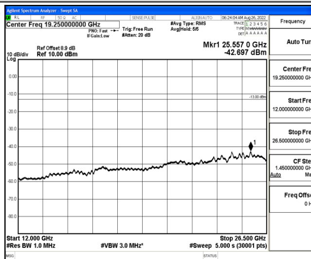
Band2-20MHz-QPSK-18900-1-0-Low-12000-26500--42.7-PASS
