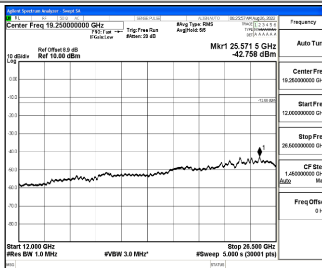
Band2-20MHz-16QAM-18900-1-0-Low-12000-26500--42.76-PASS
