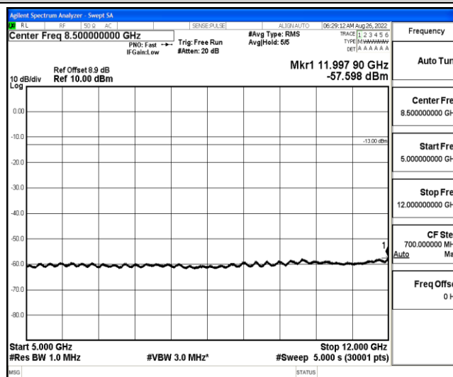
Band2-20MHz-16QAM-19100-1-0-High-5000-12000--57.6-PASS
