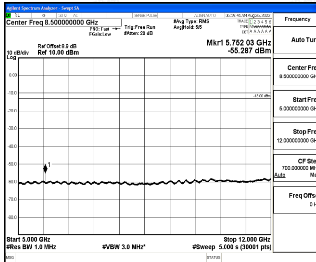
Band2-20MHz-QPSK-18700-1-0-Low-5000-12000--55.29-PASS
