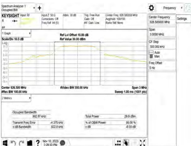
OFDM_1M_HighCH-926.5
