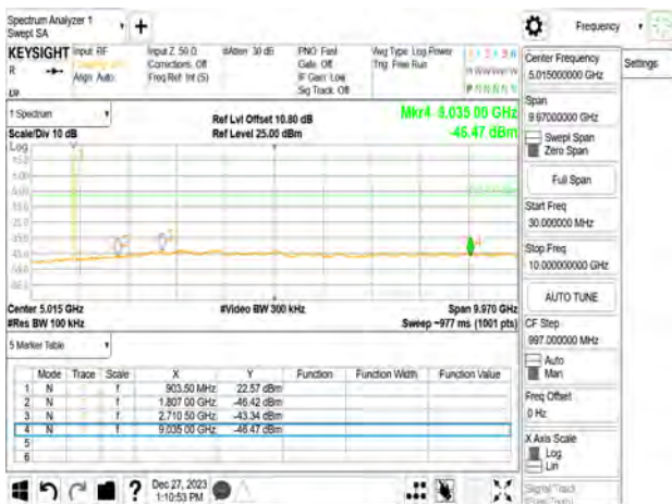
OFDM_1M_LowCH-903.5
