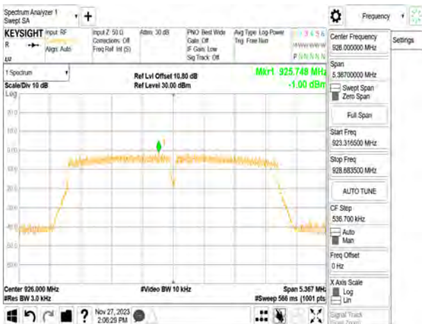
OFDM_4M_HighCH-926
