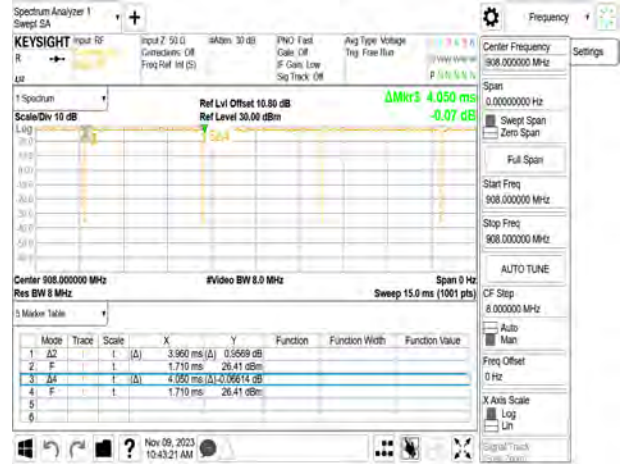
OFDM_8M_LowCH-908
