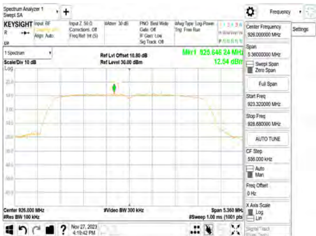
OFDM_4M_HighCH-926
