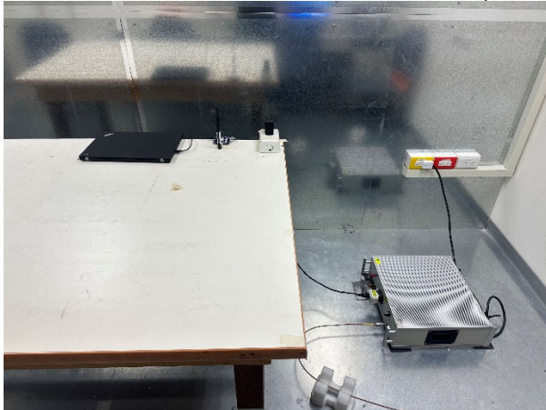
FCC_15_247_902~928MHz_OFDM_Conduction_Setup
