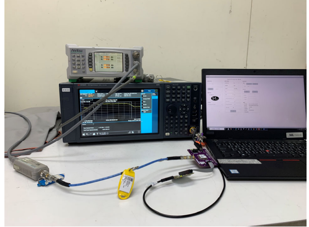
FCC_15_247_902~928MHz_OFDM_Conducted_Setup
