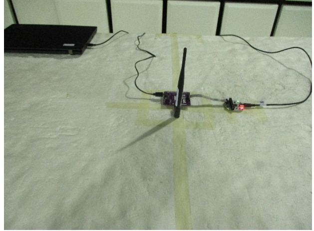
FCC_15_247_902~928MHz_OFDM_Conducted_Setup
