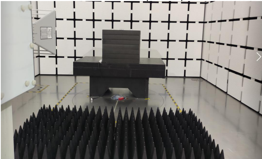
Radiated Emission (Above 1G)
