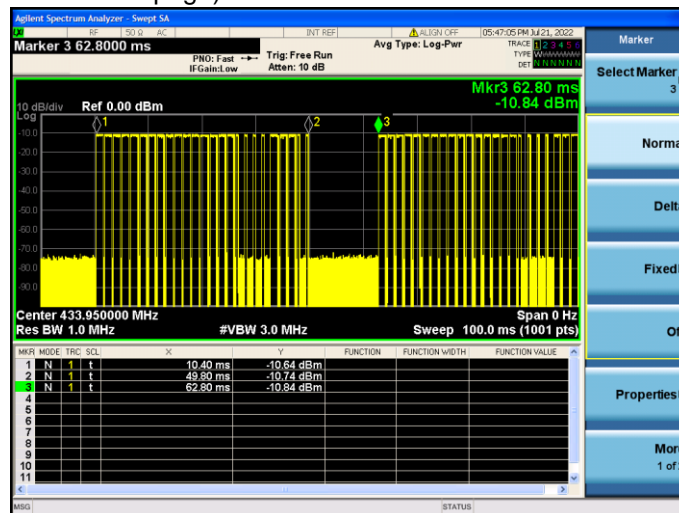
(Transmit cycle 52.40ms)
