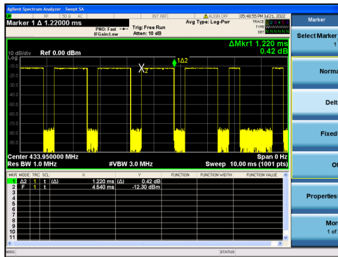
(Time per burst: 1.220ms*19pcs)
