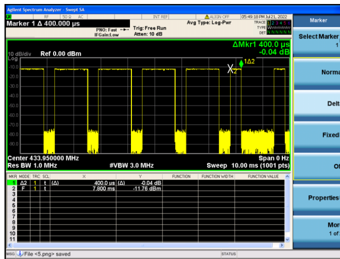
(Time per burst: 0.400ms*6pcs)
