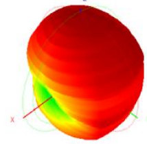
2470.0MHz HHV, Eff: 24.1%
