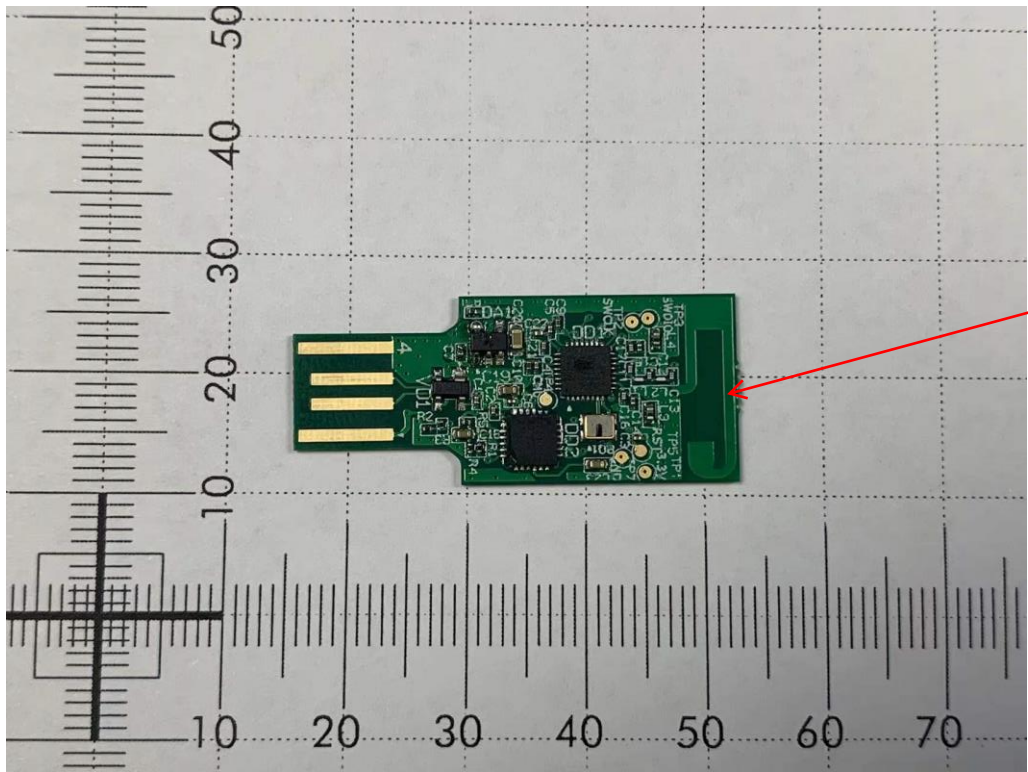
PCB Antenna
