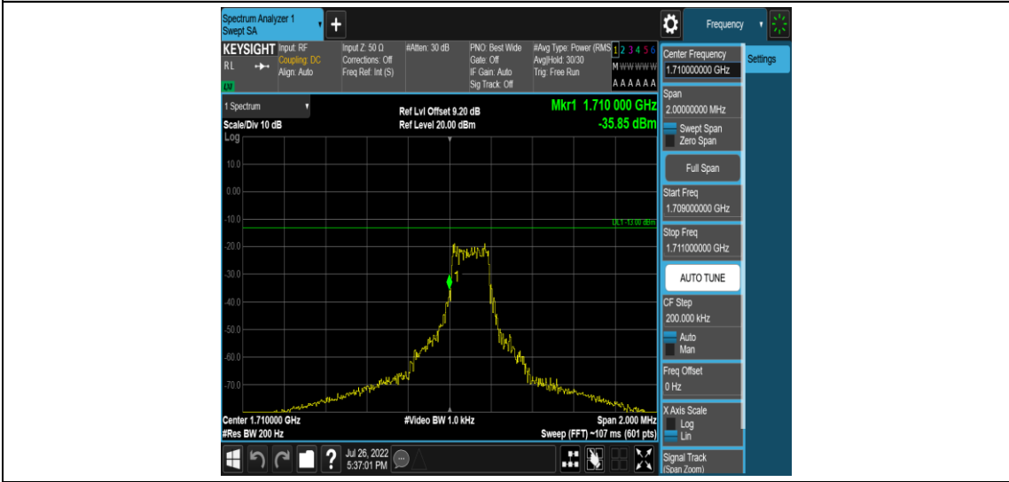
Band4-Stand-Alone-NaN-BPSK-19951-12 @ 0-15kHz--35.85-PASS
