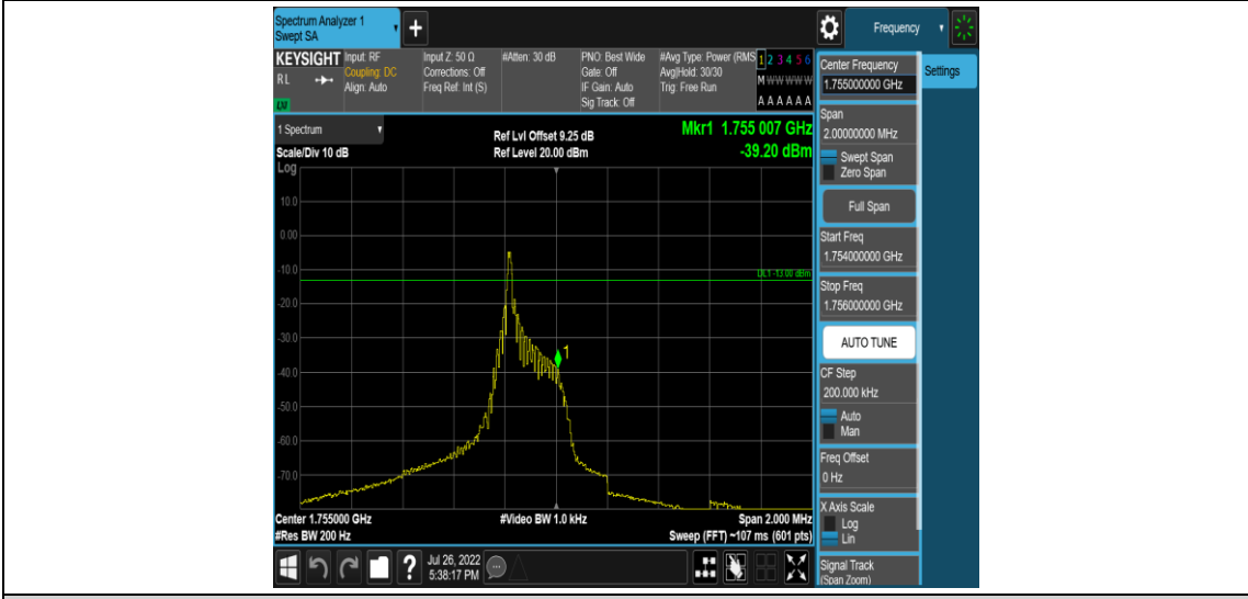
Band4-Stand-Alone-NaN-BPSK-20399-1 @ 0-15kHz--39.20-PASS
