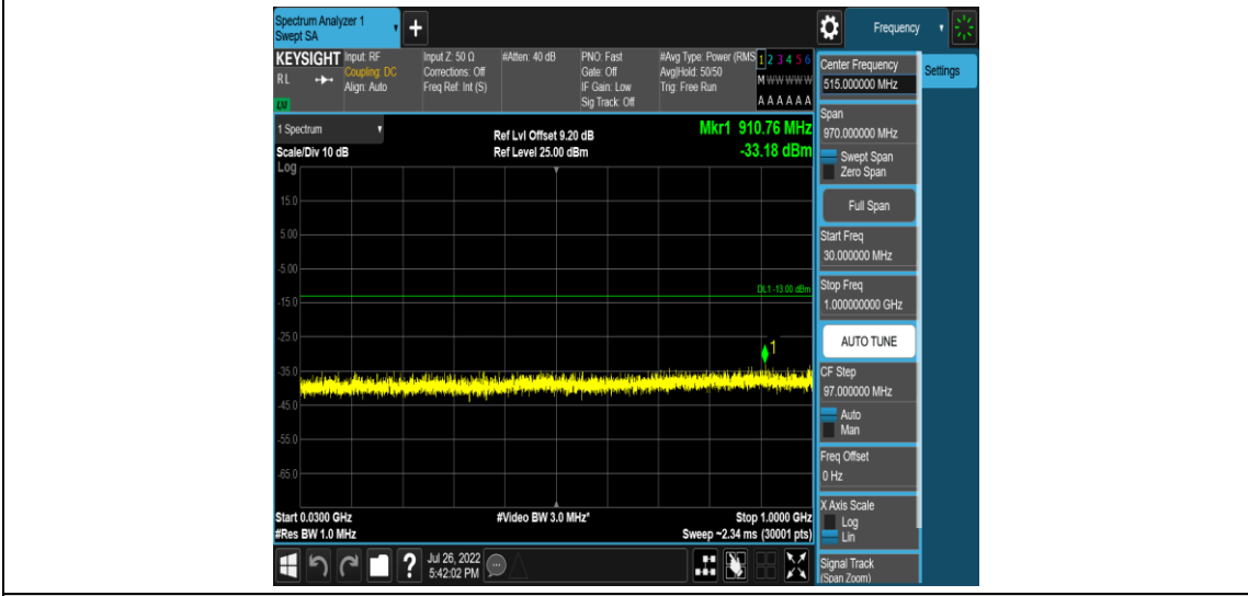
Band4-Stand-Alone-NaN-QPSK-19951-1 @0-3.75kHz-30-1000-30~1000MHz@-33.18dBm--1-3-PASS
