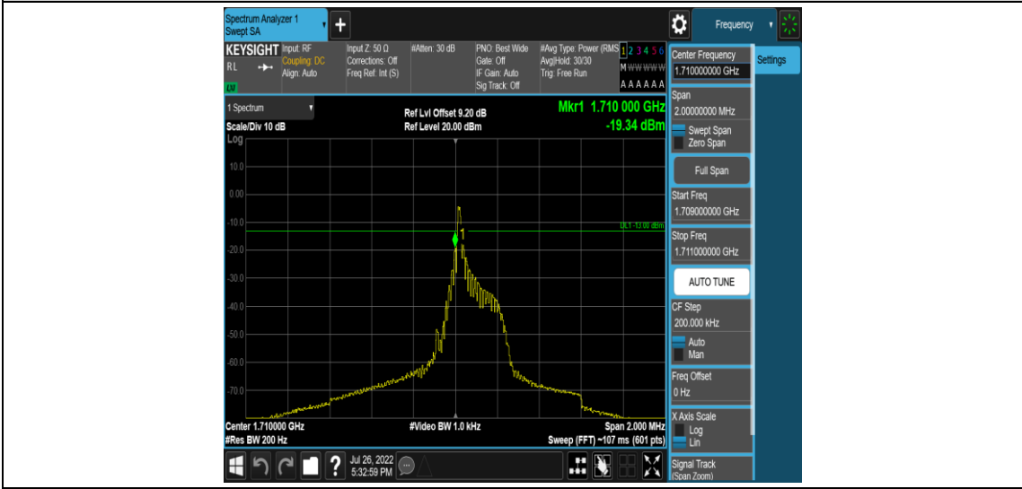
Band4-Stand-Alone-NaN-BPSK-19951-1 @0-15kHz--19.34-PASS
