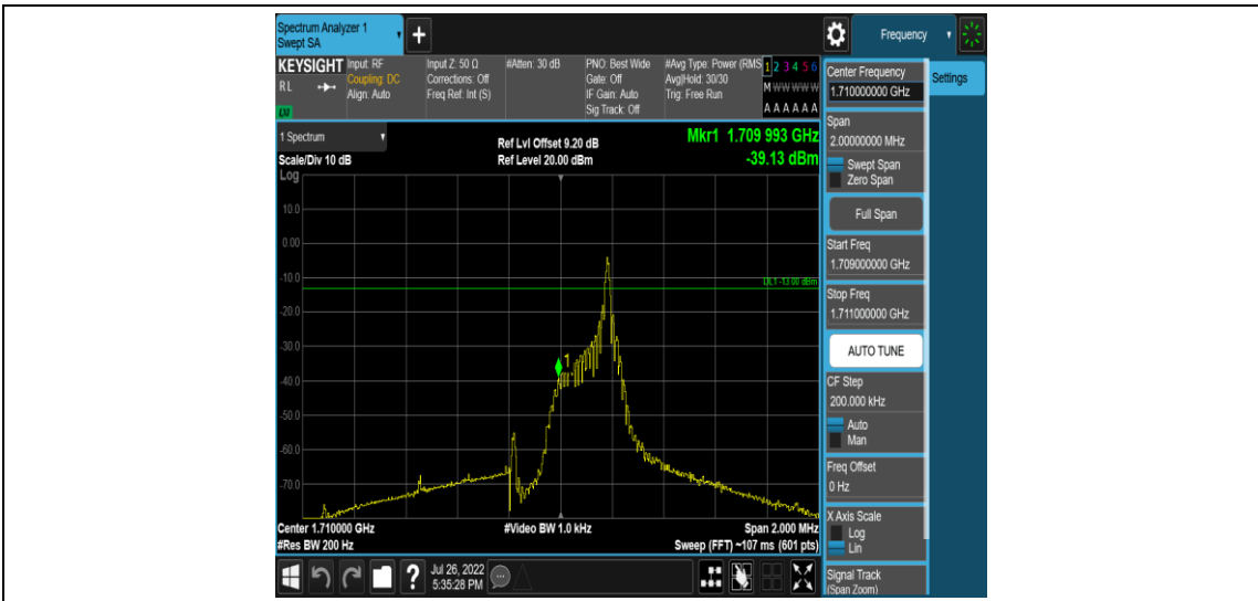
Band4-Stand-Alone-NaN-BPSK-19951-1 @ 11-15kHz--39.13-PASS
