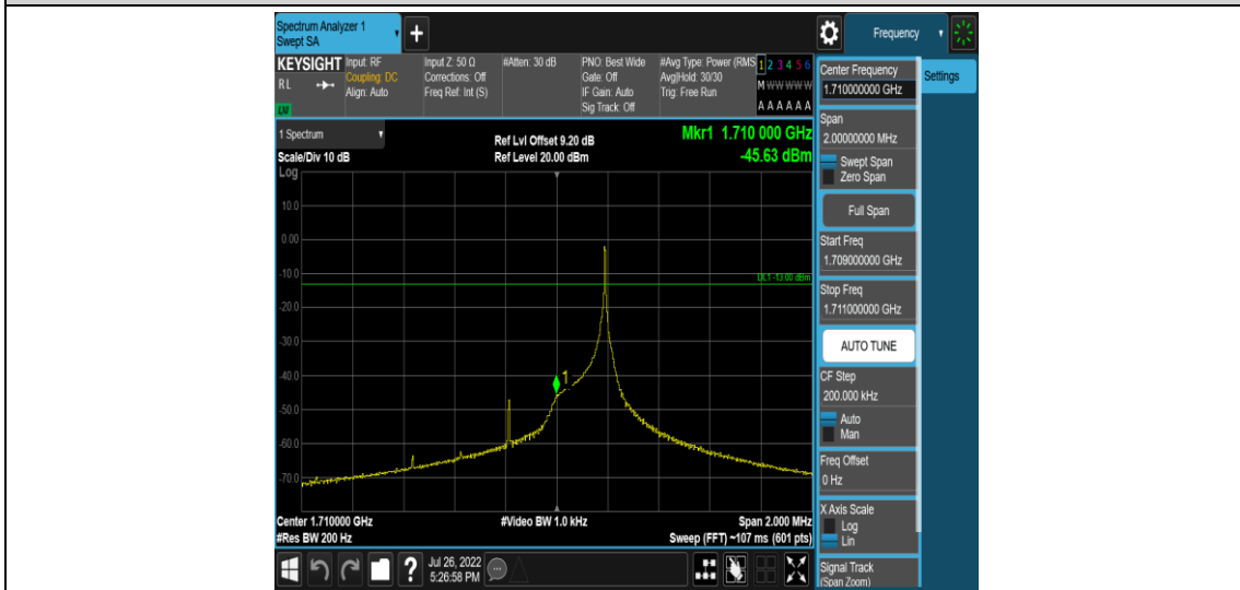
Band4-Stand-Alone-NaN-BPSK-19951-1 @47-3.75kHz--45.63-PASS
