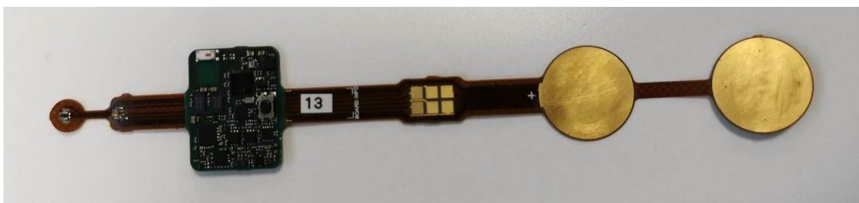
PCB component side, without battery attached
