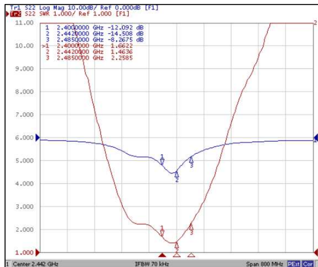
Return Loss & VSWR
