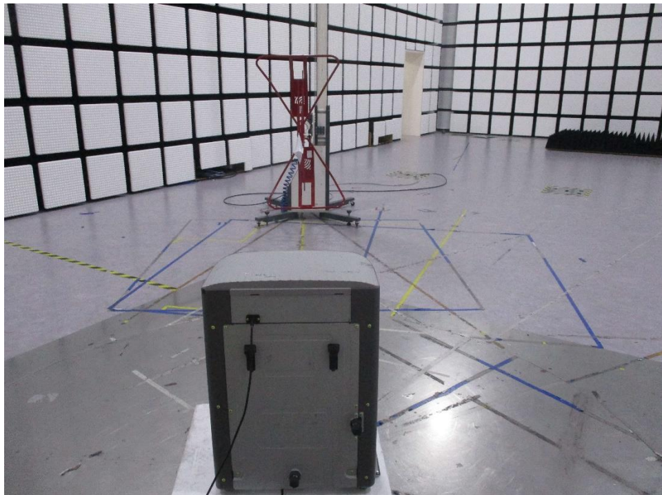
Radiated disturbance (30-1000 MHz)
