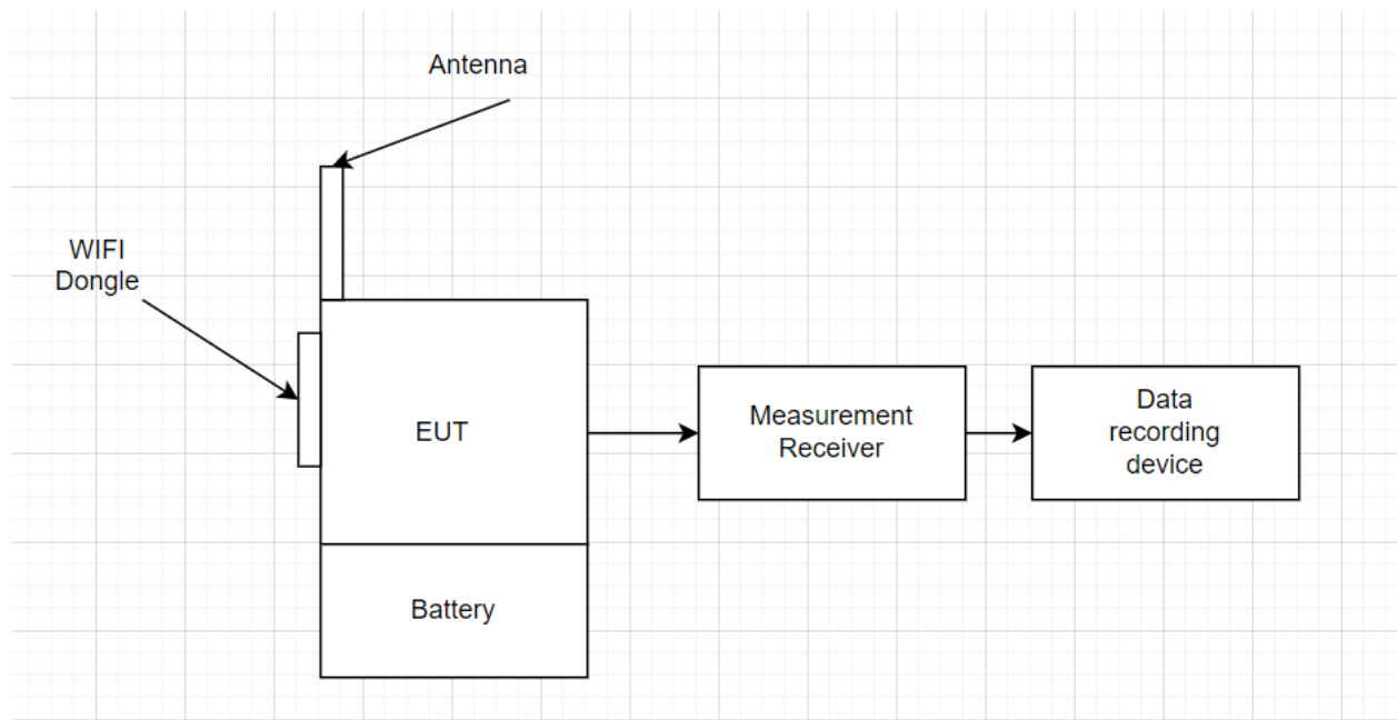
Figure 3.4-1: Setup diagram
