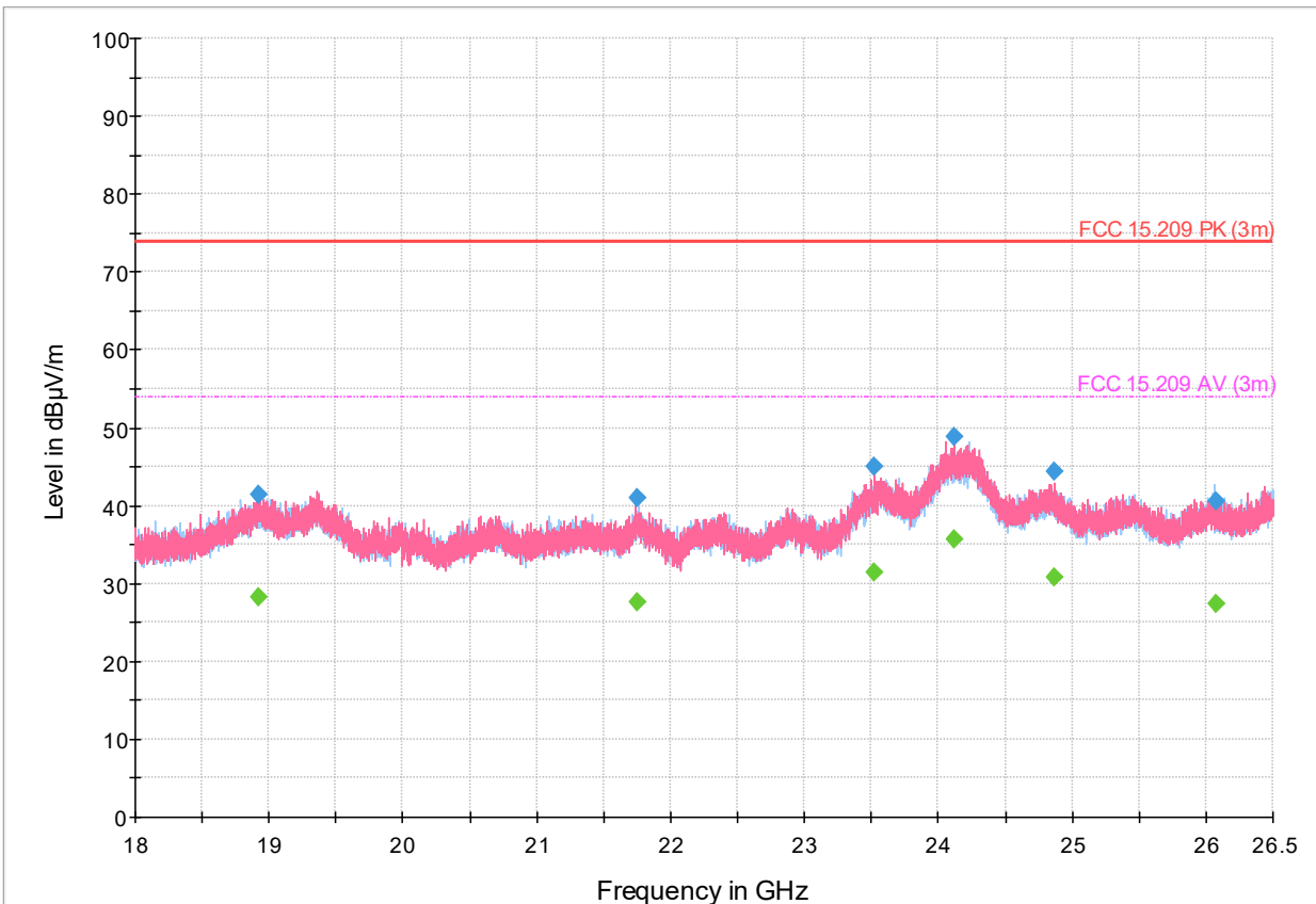
Figure 8.1-8: Radiated emission TSM-18-26.5GHz-2404-BW4-TW950 Wi-Fi channel g
