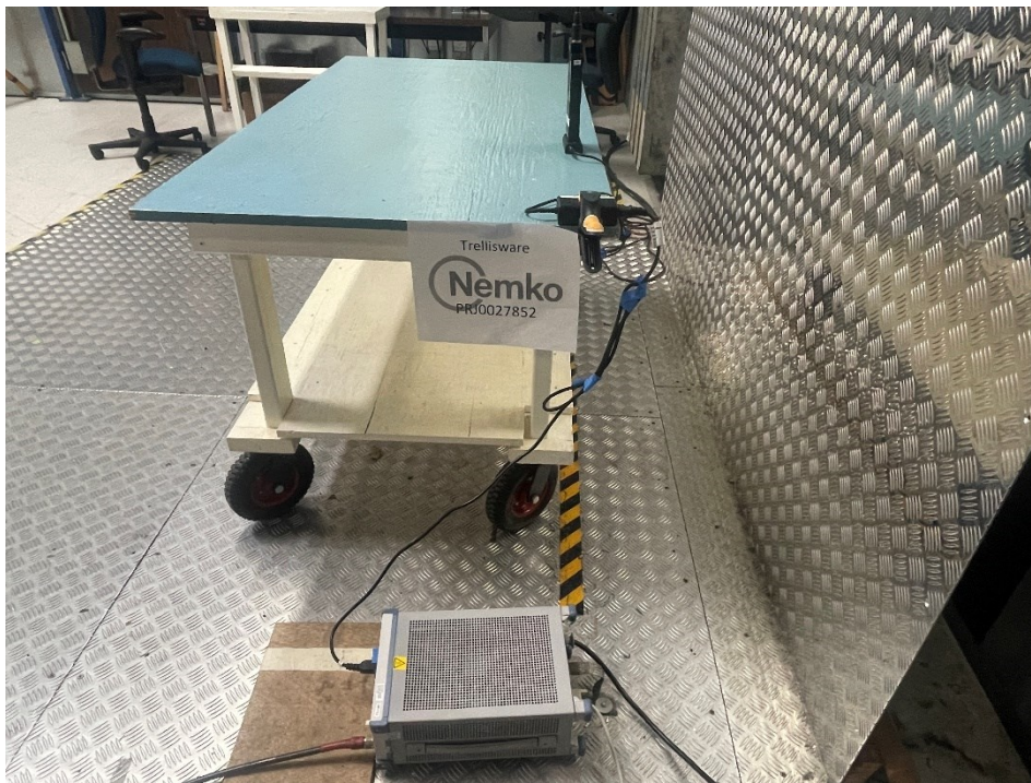
Figure 8.2.3 Conducted disturbance at AC mains port setup photo side
