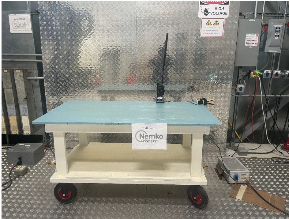
Figure 8.2.2 Conducted disturbance at AC mains port setup photo front
