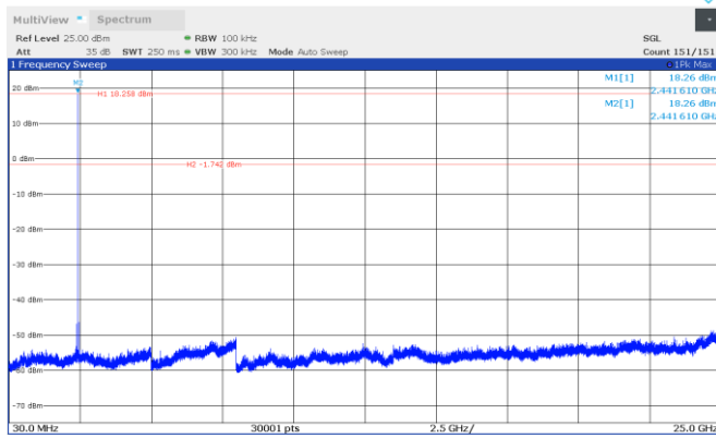
Figure 8.3-13: TSM-Bandwidth 1.2MHz conducted spurious emission, 2442 MHz
