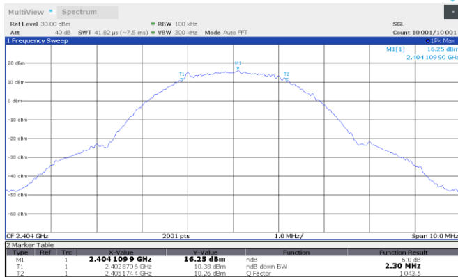
Figure 8.1-4: TSM Bandwidth 3.6MHz 6dB DTS bandwidth, 2404 MHz
