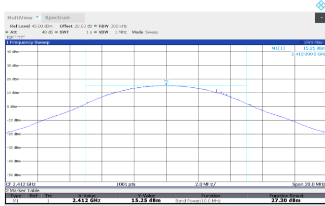
Figure 8.2-7: TSM-Bandwidth 10MHz Conducted output power, 2412 MHz
