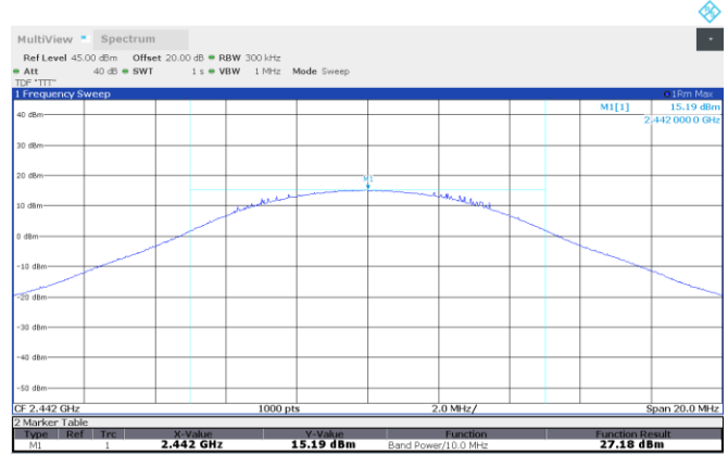
Figure 8.2-8: TSM-Bandwidth 10MHz Conducted output power, 2442 MHz
