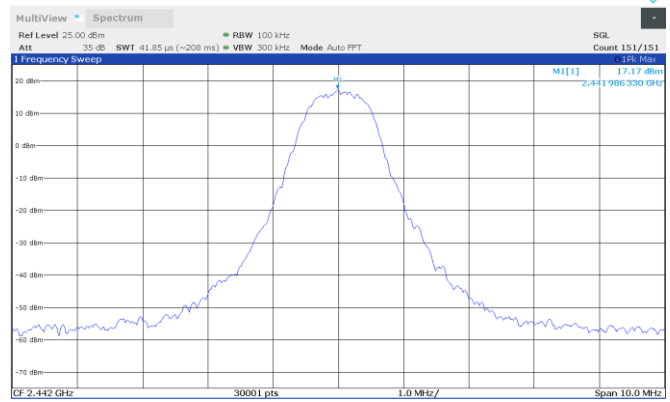
Figure 8.3-14: TSM-Bandwidth 1.2MHz conducted spurious emission reference level, 2442 MHz
