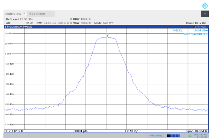
Figure 8.4-12: TSM-Bandwidth 1.2MHz conducted spurious emission reference level, 2442 MHz
